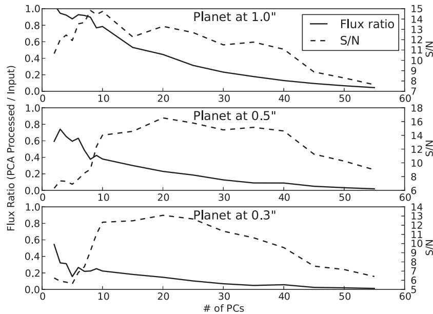
Figure 3. Comparison of the flux ratio and S/N based on number of PCs at different radii. The top panel is for a fake planet at 1''.0 , the middle panel is for 0''.5 and the bottom panel is for 0''.3 . These panels demonstrate that, while the flux ratio does decrease with PCs, the S/N follows a different curve.
