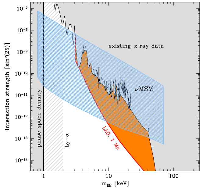
FIG. 8 (color online). Grey shading: Bounds on sterile neutrino parameters [54]. Blue hatching shows the allowed parameter space of the \nu\text{MSM} model. The vertical solid line marks the lower bound on the mass from the phase space density constraint; the grey-hatched region shows the excluded limit based on the \text{Ly}\alpha data. The data point with error bars makes the claimed detection of the 7.1 keV decaying dark matter line in galaxy clusters and M31 [58,59]. Orange shading shows the sensitivity limit of LOFT for 1 Ms exposure.
