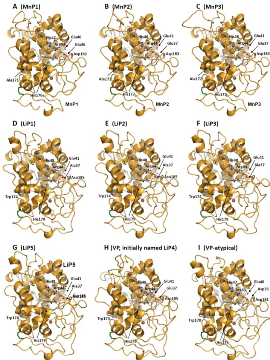
Figure 6 Molecular models for the nine class-II heme peroxidases (AA2) found in the P. cinnabarinus genome. MnP models (A-C) present a Mn 2+ oxidation site characteristic of typical MnPs, formed by two glutamates and one aspartate at the internal heme propionate region; LiP models (D-G) exhibit a Trp residue exposed to the solvent, which has been involved in high-redox-potential aromatic compound oxidation by typical LiPs; the VP model (H) obtained for the only peroxidase of this family identified in the genome analysis evidences both the Mn 2+ oxidation site and the Trp residue exposed to the solvent, characteristic of members of this class-II family; the atypical VP (I) contains an aspartate residue (Asp36) in a position occupied by a glutamate in VPs and MnPs. Two axial histidines, one acting as heme iron ligand (proximal histidine) and the second (distal histidine) contributing to the heme reaction with peroxide, together with an arginine residue characterizing class-II peroxidases are also shown in the nine molecular homology models. Four disulfide bridges are depicted as green sticks. These homology models were obtained at the Swiss-Model protein-homology server [83] using P. eryngii VPL (PDB entries 4FCS, 2VKA and 3FJW) and P. chrysosporium LiPH2 and LiPH8 (PDB entries 1LLP, 1B80 and 1B82) crystal structures as templates.
