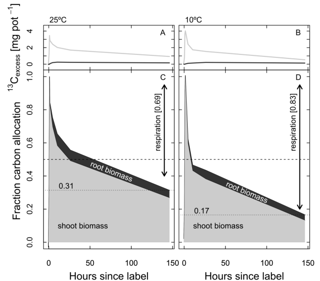
Fig. 3. (A, B) Time course of ^{13}\text{C}_{\text{excess}} in shoot (light grey) and root (dark grey) and (C, D) the derived fraction of carbon allocation relative to the initial shoot enrichment of shoot bulk material ( \delta^{13}\text{C}_{\text{SB}} ); warm treatment ( 25^\circ\text{C} , left panels); cold treatment ( 10^\circ\text{C} ; right panels); final value of biomass allocated to roots and shoots (dotted line); 0.5 fraction carbon allocation is indicated for reference (dashed line).
