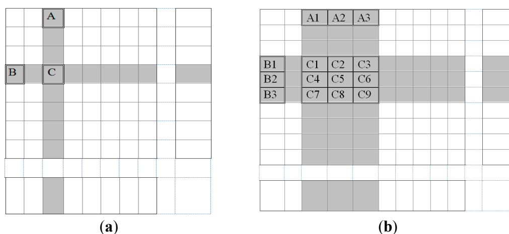
Figure 1. Disaggregation principle for obtaining a detailed initial estimate. Aggregated values (a) are either disaggregated per column (case A), per row (case B) or both (case C). (a) Original aggregate table; (b) “Initial estimate” disaggregated table.
