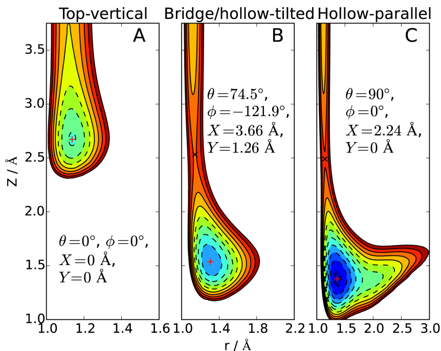
Figure 2: The PBE interaction energy is plotted as a function of r and Z for the three configurations corresponding to the molecular adsorption geometries. The position of the adsorption geometries is indicated in the plots by a red +, and a black \times indicates the position of the saddle point in the entrance channel. Interaction energies have been evaluated on a dense grid in r and Z and spline interpolated for illustration purposes. Contour lines separate 0.2 eV energy intervals up to a maximum of 0.8 eV. Dashed lines identify negative energy values.
