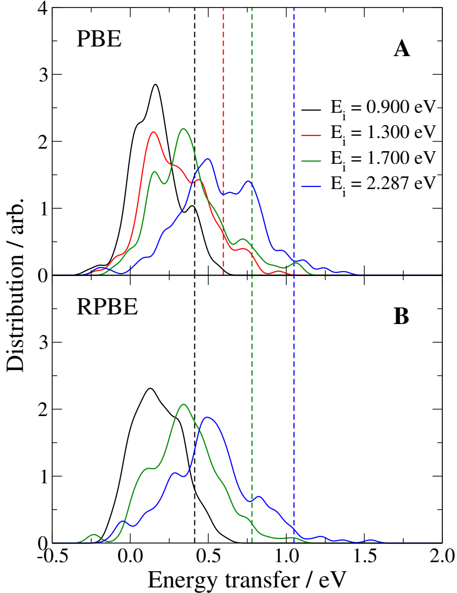
Figure 7: Energy transfer distributions computed for molecules scattered without performing any rebound on the surface are plotted as solid lines. Smooth distributions have been obtained by summing Gaussian functions centered at the computed energy distribution values with a \sigma parameter equal to 40 meV. The energy transfer values according to the Baule model are plotted as vertical dashed lines. Different colors correspond to the various initial collision energies: black for 0.9 eV, red for 1.3 eV, green for 1.7 eV and blue for 2.287 eV. A is for PBE and B is for RPBE.
