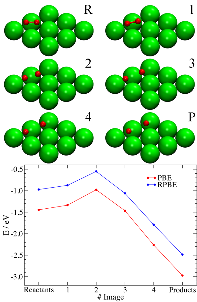
Figure S3: Same as Figure S1, but the reactants (R) correspond here to the hollow-parallel molecular adsorption configuration.
