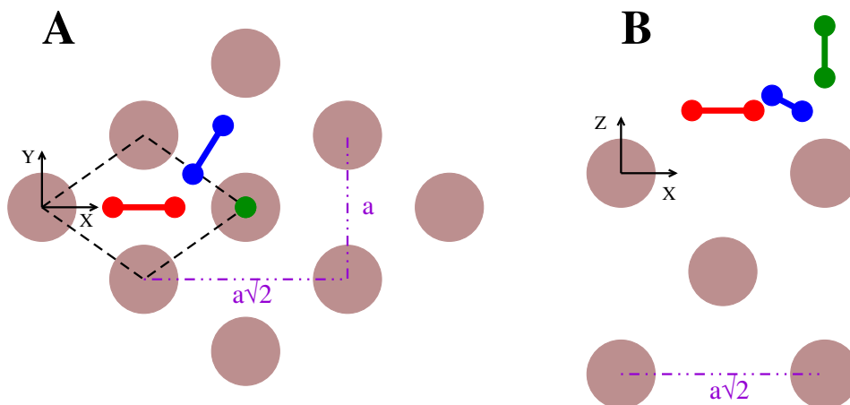
Figure 1: Graphical illustration of the molecular adsorption states: green for top-vertical, red for hollow-parallel and blue for bridge-hollow-tilted, using nomenclature as in the text. A and B represent bird's-eye and side views, respectively. Brown circles represent the surface atoms. The dashed black line delimits the surface unit cell.
