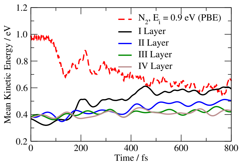
Figure 9: The mean kinetic energies evaluated for the PBE trajectories with E_i = 0.9 eV dissociating at propagation times larger than 800 fs is plotted as a function of time. The dashed red line corresponds to the mean kinetic energy of the molecule, while black, blue, green and brown solid lines correspond to the mean kinetic energy of the first, second, third and fourth atomic layers, respectively.
