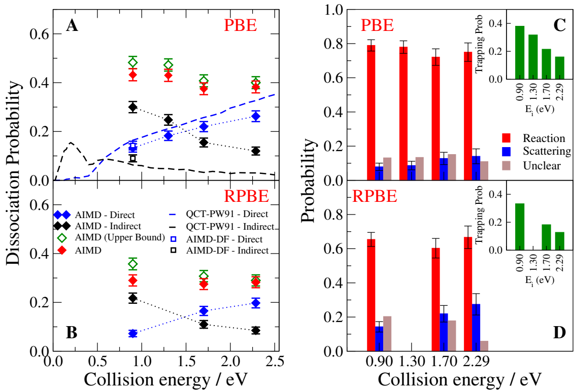
Figure 6: A-B: The direct (blue diamonds) and trapping-mediated (black diamonds) contributions to the dissociation probability (full red diamonds) obtained with AIMD are plotted as a function of E_i . Upper bound for the dissociation probabilities are also provided (empty green diamonds), assuming that all the unclear trajectories will dissociate. Direct and indirect dissociation probabilities for AIMD calculations simulating a distorted frozen surface (AIMD-DF) are plotted as empty blue and black squares, respectively. The direct and trapping-mediated contributions to the dissociation probability determined in the previous static-surface QCT study [12] are also plotted as dashed lines for comparison. In A, the AIMD employed the PBE functional and the QCT calculations the PW91 functional, while in B the RPBE functional has been employed in the AIMD. C-D: Reaction and scattering probabilities for trapped molecules are plotted as red and blue bars, respectively. The fraction of trapped molecules that are neither dissociated nor scattered at the end of the propagation time is plotted in brown. In the insets, the trapping probability as a function of E_i . C is for PBE, D is for RPBE.
