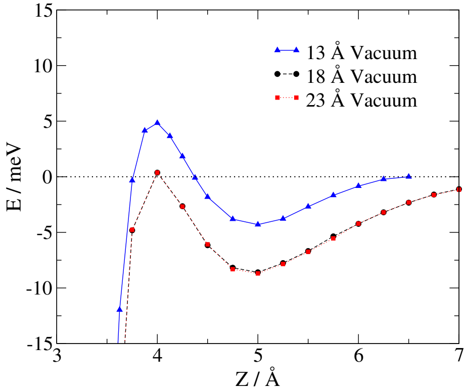
Figure 4: The PBE interaction energy is plotted as a function of Z , using the same equilibrium 5-layer slab to model the W(110) surface, but using different vacuum spaces along the surface normal. The N_2 bond length has been kept equal to the equilibrium value of 1.117 \text{ \AA} . The zero of energy is defined as the energy of the molecule in its equilibrium geometry placed midway between two slabs.
