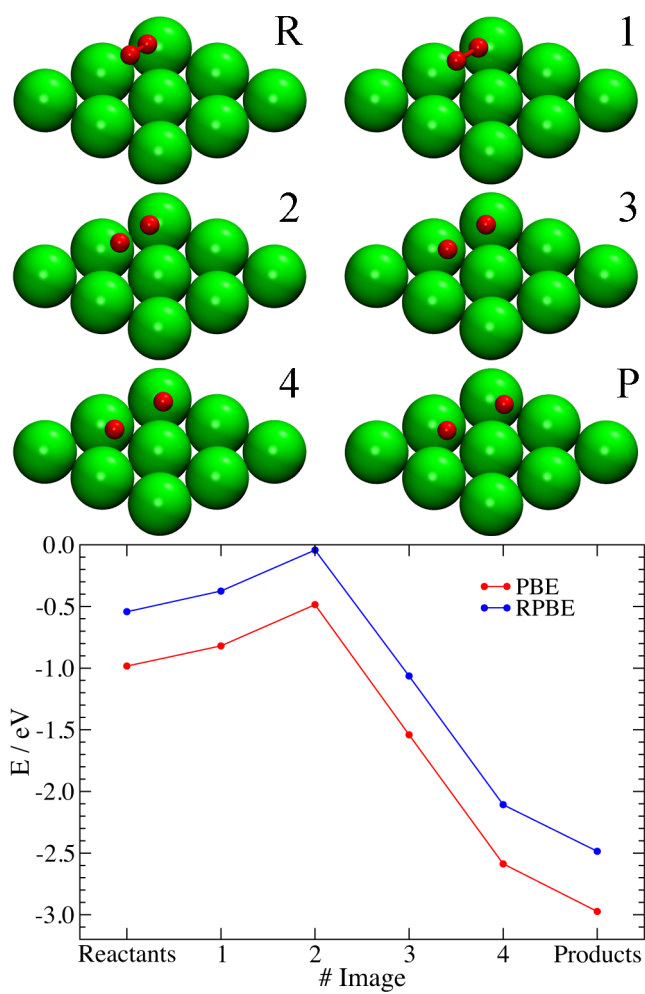
Figure S2: Same as Figure S1, but the reactants (R) correspond here to the bridge/hollow-tilted molecular adsorption configuration.
