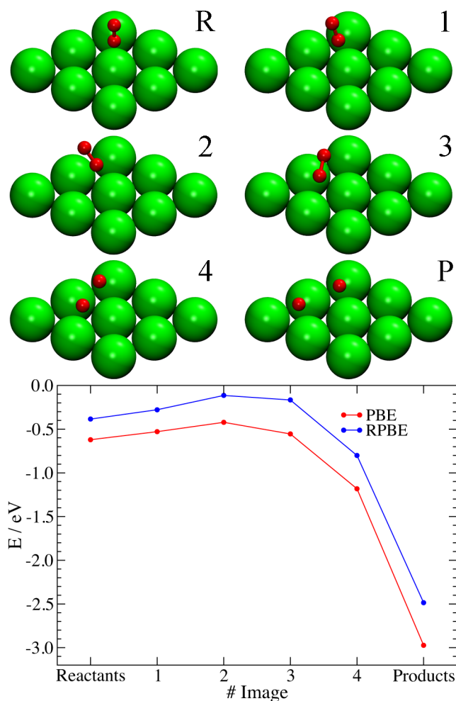
Figure S1: Results of CI-NEB calculations, optimizing four images (1-4) between the top-vertical molecular adsorption geometry (reactants, R), and the lowest-energy dissociated adsorption state (products, P). In the lower panel, the energy of each configuration is plotted as a function of the image number. Red is for PBE and blue for RPBE. Straight lines connect points corresponding to consecutive images. The molecular configurations, as well as first layer surface atoms, are schematically represented above.
