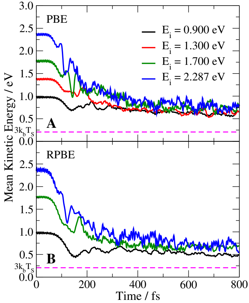
Figure 8: The mean kinetic energy of the molecules dissociating at propagation times larger than 800 fs is plotted as a function of time. A is for PBE and B is for RPBE. Colors are as for figure 7. The dashed horizontal line indicates the energy corresponding to 3k_b T_S .
