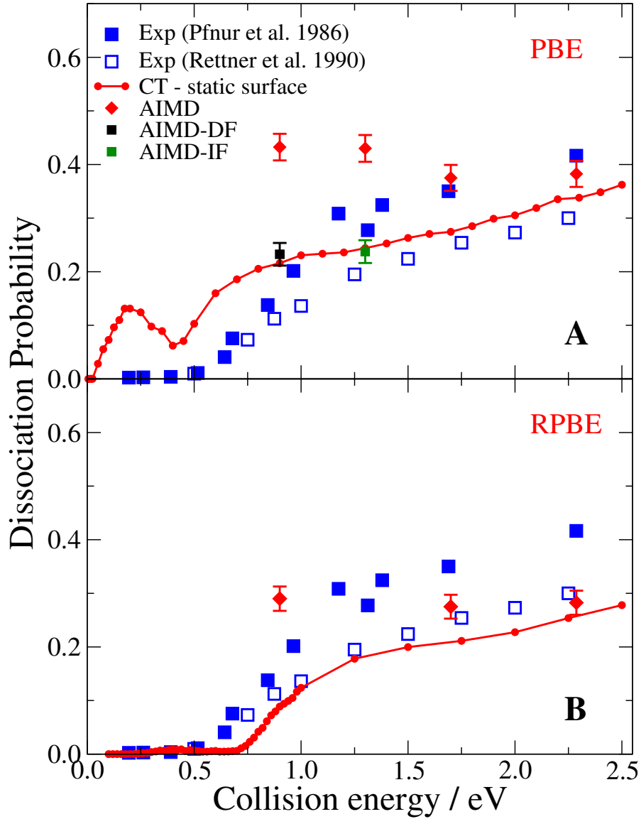
Figure 5: Dissociation probability as a function of the initial collision energy. AIMD moving-surface results (AIMD, diamonds) are compared to experimental data (blue squares, solid from Ref. [5] and empty from Ref. [9]) and to previous static-surface CT calculations [15]. The dissociation probability values computed using AIMD, simulating an ideal frozen surface (AIMD-IF, green) and simulating a distorted frozen surface (AIMD-DF, black) are also reported. In A, all AIMD calculations employed the PBE functional and the CT calculations the PW91 functional, while in B the RPBE functional has been employed by both AIMD and CT calculations.
