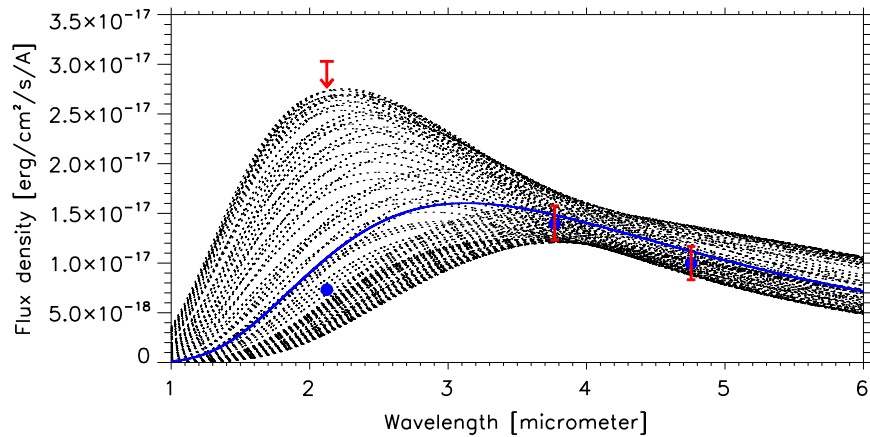
Figure 5. Observed flux densities (with 1\sigma error bars) and upper limit (all red data points) overlaid on blackbody emission curves. The blue line corresponds to the best \chi^2 fit for effective temperature and emitting area. The blue points result from convolving the blue line with the transmission curves of the K_s , L' , and M' filters. The black dotted lines are a set of representative blackbodies from within the 1\sigma region of the \chi^2 fit.
