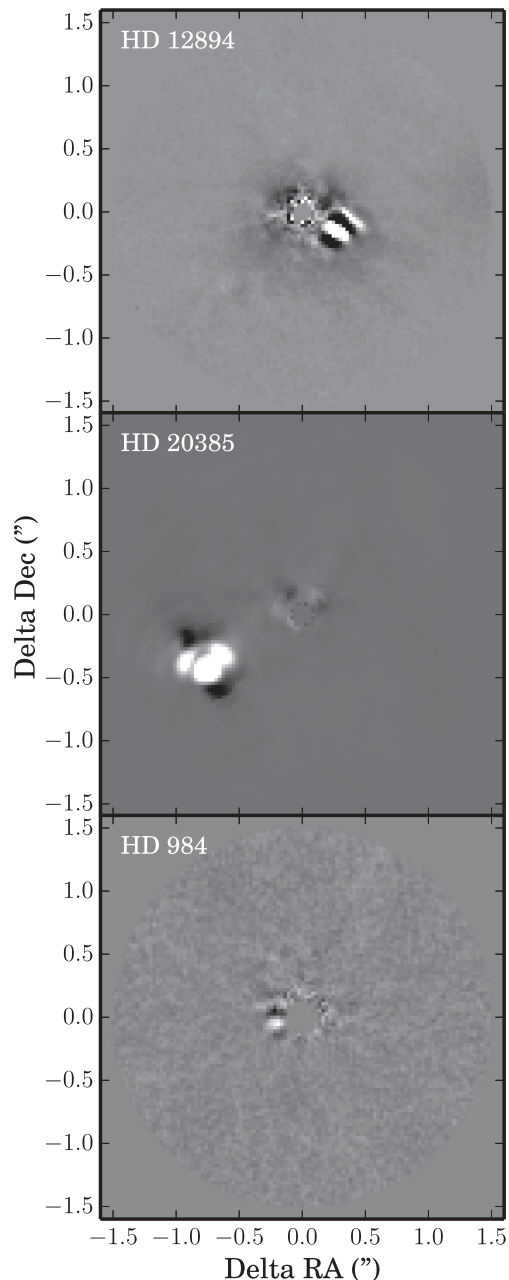
Figure 3. Top: HD 12894 ADI processed image, with the companion at 0.31 arcsec. Middle: HD 20385 ADI processed image, with the companion at 0.87 arcsec. The shape of the companion PSF is due to the APP PSF. Bottom: HD 984 PCA processed image with the companion 0.19 arcsec from star.
