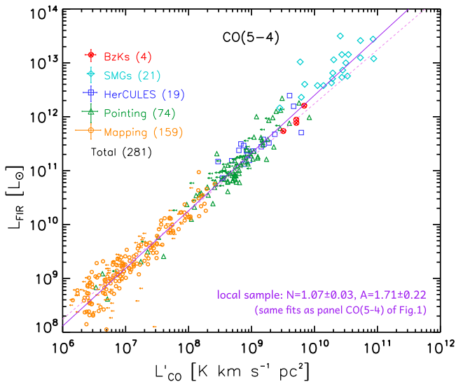
Figure 3. CO(5–4)–FIR correlation including high- z galaxies. The cyan diamonds are high- z galaxies from CW13. The crossed red circles are z \sim 1.5 BzKs from Daddi et al. (2015). The other data points and the best fit of the local sample are the same as the CO(5–4) panel of Figure 1.
