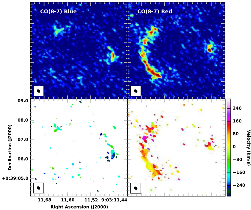
Figure 5. CO J = 8 - 7 integrated intensity (top) and velocity field (bottom) images for the B and R components. The B and R components were defined from -307 to -76 km s^{-1} and -55 to 239 km s^{-1} , respectively, based on their spectral profiles (Figure 3).
