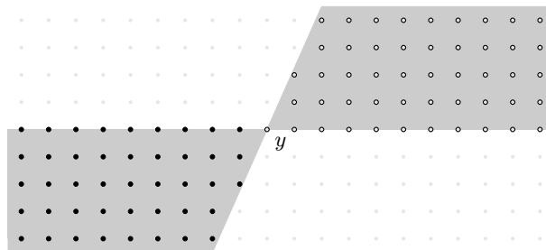
Figure 3: An illustration of the sets \angle(y) (represented by white circles) and \overline{\angle}(y) (represented by filled black circles), with y = (x, n) \in \mathbb{Z}^2 .
