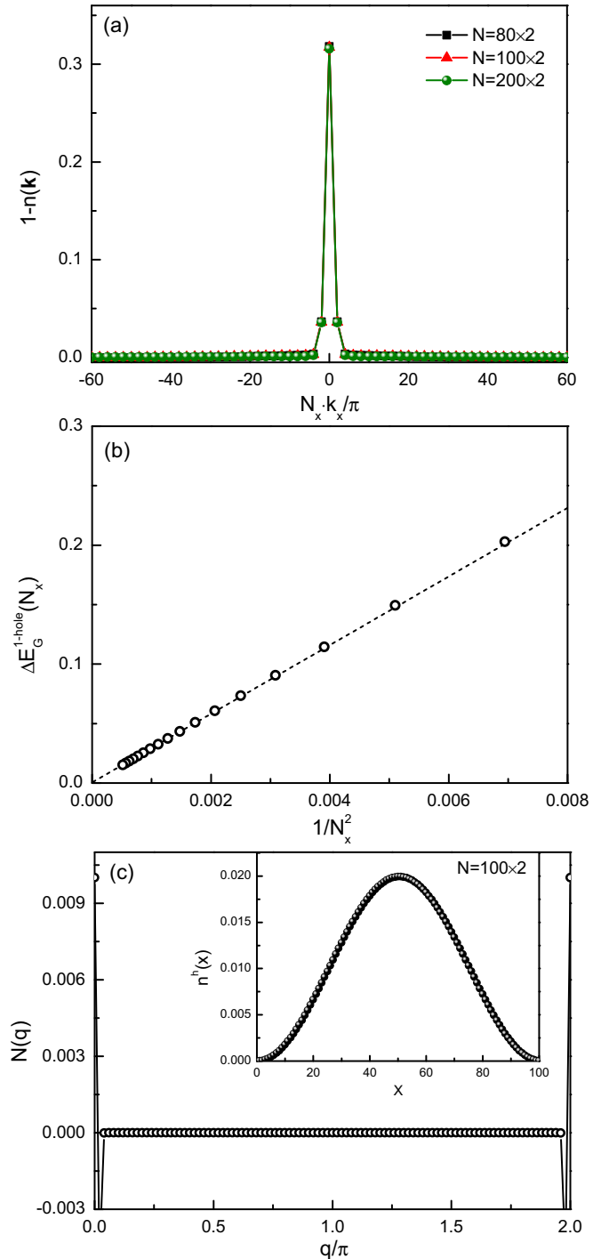
FIG. 6. (Color online) The simulation results for the single-hole doped \sigma \cdot t - J ladder. (a) The single-hole momentum distributions for different ladders fall into a universal curve displaying a sharp quasiparticle peak. (b) The hole's energy also displays a “free-particle”-like behavior, i.e., \Delta E_G^{1\text{-hole}} \sim N_x^{-2} . (c) Both the spatial resolution (inset) and the Fourier transformation (main panel) of the hole density profile show the absence of charge modulations. Here, \alpha = 1 and t/J = 3 .
