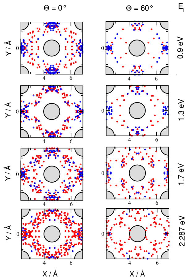
FIG. 11. XY position of the COM of the reactive molecules at the time of the dissociation (see text for definition). The COM positions have been reported in the minimum wedge and then replicated in the \sqrt{2} \times \sqrt{2} super-cell using symmetry operations. Direct and indirect events are indicated as red and blue circles, respectively. Tungsten first layer atoms in their equilibrium positions are shown as gray circles.
