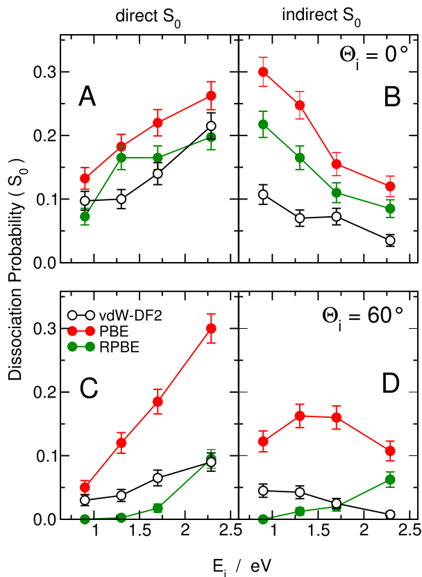
FIG. 10. Direct ((a) and (c)) and indirect ((b) and (d)) reaction probabilities as a function of E_i for \Theta_i = 0^\circ ((a) and (b)) and \Theta_i = 60^\circ ((c) and (d)). vdW-DF2 results are reported as black empty circles. PBE and RPBE data (full red and green circles, respectively) for normal incidence are taken from Ref. 15.
