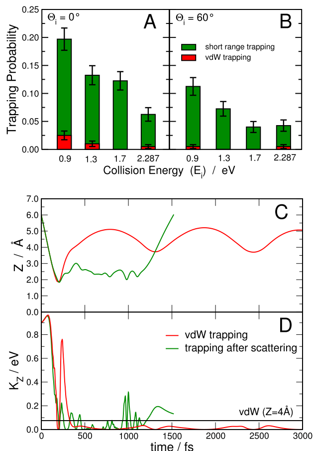
FIG. 16. ((a) and (b)) Probability of short range and vdW trapping for the collision energies and angles studied. ((c) and (d)) Comparison between two trajectories undergoing short-range (green) and vdW (red) trapping; the distance from the surface ( Z ) and the kinetic energy along Z ( K_z ) is plotted as a function of time. In panel (d), the interaction potential calculated at Z = 4 Å is plotted as an horizontal black line.
