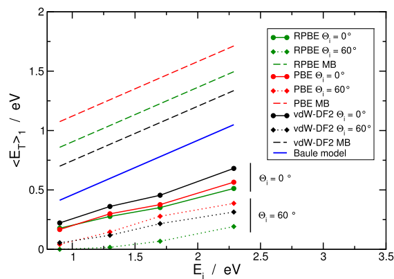
FIG. 13. Comparison between the mean energy transfer to the surface calculated from the molecules that do not perform any rebounds on the surface ( \langle E_T \rangle_1 ) and the energy transfer predicted by the modified Baule model. Data are reported for the functionals considered (in red, green, and black, for PBE, RPBE, and vdW-DF2, respectively) for \Theta_i = 0^\circ (solid lines), \Theta_i = 60^\circ (dotted lines), and for the modified Baule model (dashed lines). The standard Baule model is reported as a thick blue line. PBE and RPBE data are taken from Ref. 15.
