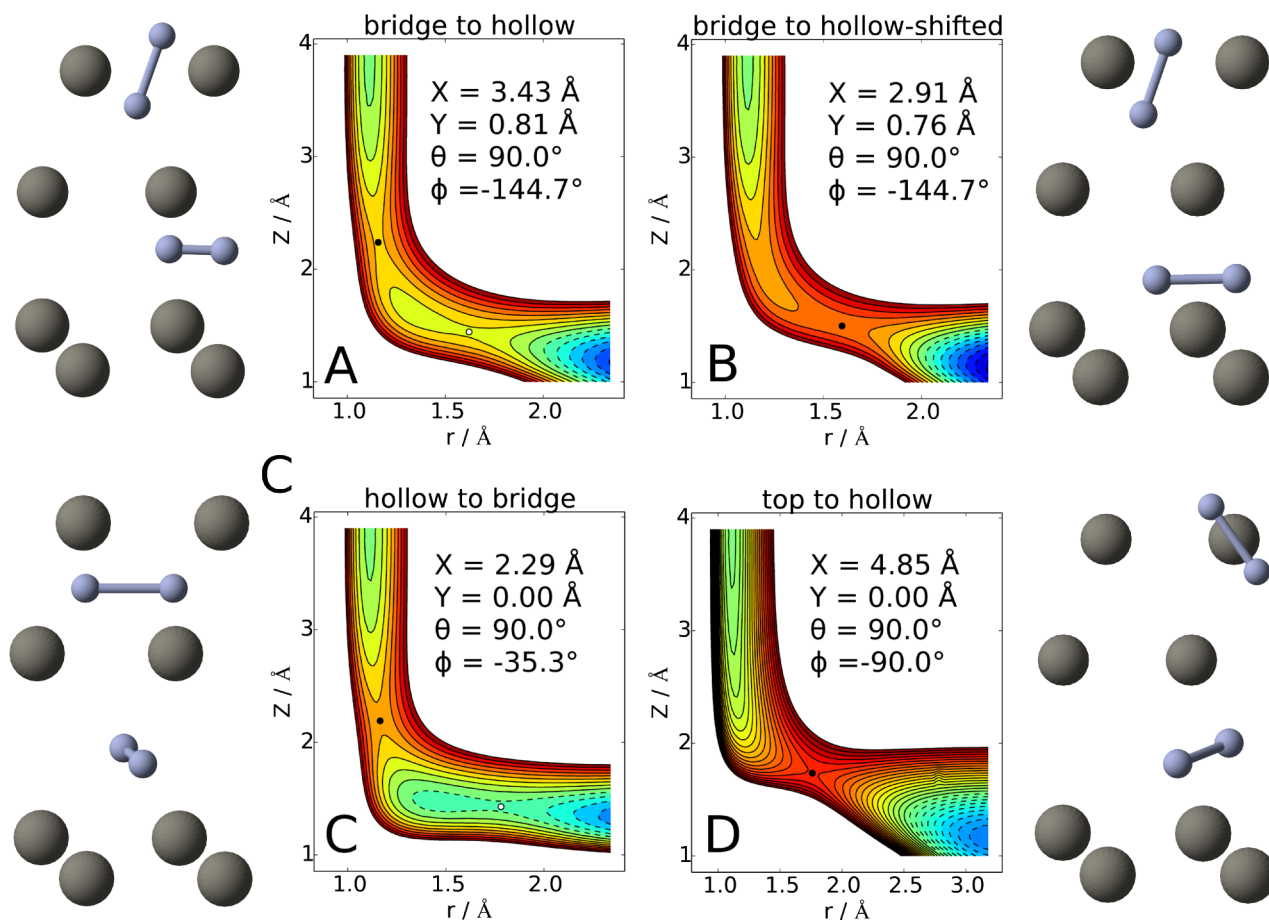
FIG. 6. 2D ( r,Z ) cuts of the PES computed for four dissociation geometries: bridge-to-hollow (a), bridge-to-hollow-shifted (b), hollow-to-bridge (c), and top-to-hollow (d). Contour lines separate 0.2 eV energy intervals, solid lines are used for E \geq 0 eV, and dashed lines for E < 0 eV. Circles indicate all the stationary points. The black circles represent the entrance channel barriers for dissociation ( E_b^{DirDiss} ) and the white circles are 2D saddle-points that are not real first order saddle-points in the 6D space (see text for details). The top and the side view sketches of the direct dissociation barrier geometries are reported next to the corresponding elbow plots.
