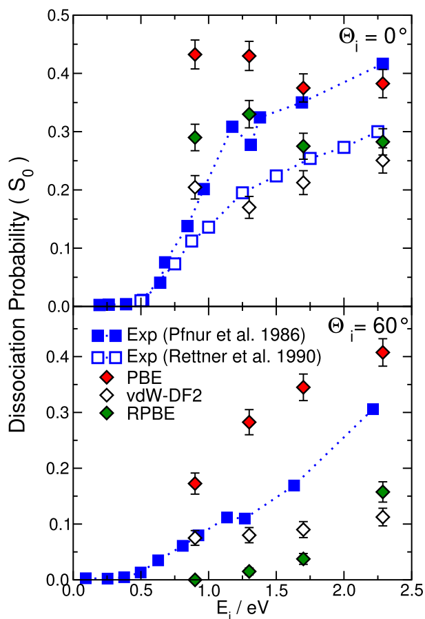
FIG. 9. Reaction probability as a function of the collision energy E_i for \Theta_i = 0^\circ (top panel) and \Theta_i = 60^\circ (bottom panel). vdW-DF2 results are reported as black empty diamonds. PBE and RPBE data (full red and green diamonds, respectively) for normal incidence are taken from Ref. 15. Experimental data are taken from Ref. 7 (full blue squares) and Ref. 8 (empty blue squares).
