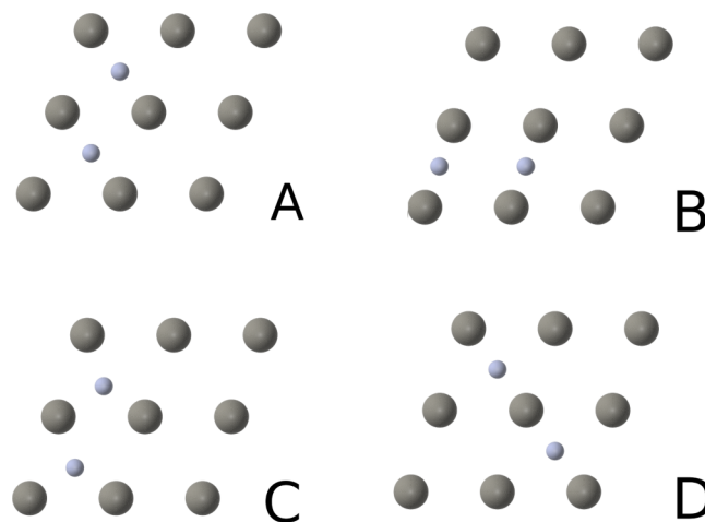
FIG. 7. Dissociation products considered as a result of a bridge-to-hollow (a), hollow-to-bridge (b), bridge-to-hollow-shifted (c), and top-to-hollow (d) dissociation.
