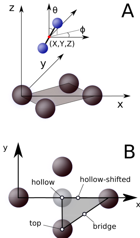
FIG. 2. Coordinate system (a) and sites on the surface (b). Dark gray, light gray, and blue are used for first layer W atoms, second layer W atoms, and nitrogen, respectively. In (a), the coordinates of the molecular center of mass are reported (X, Y, Z) . In (b), the irreducible wedge is indicated.
