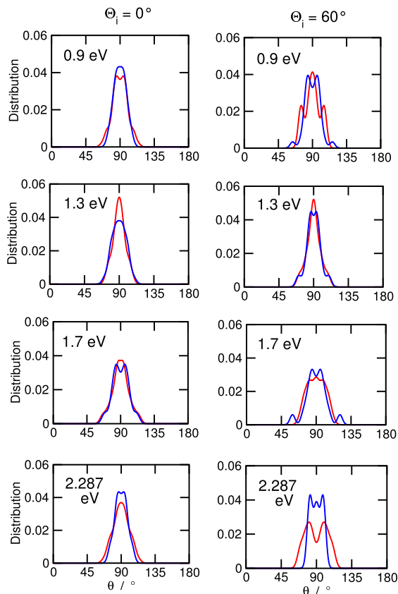
FIG. 12. Distribution of the angle between the molecular axis and the surface normal ( \theta ) at the time of the reaction (see text for definition) for both the direct and the indirect mechanisms (red and blue lines, respectively). To increase the resolution of the data, for each molecule have been reported the two values of \theta obtained inverting the N atoms (i.e., the angles \theta and 180^\circ - \theta have been reported for each atom). The incidence energy E_i is reported as inset.
