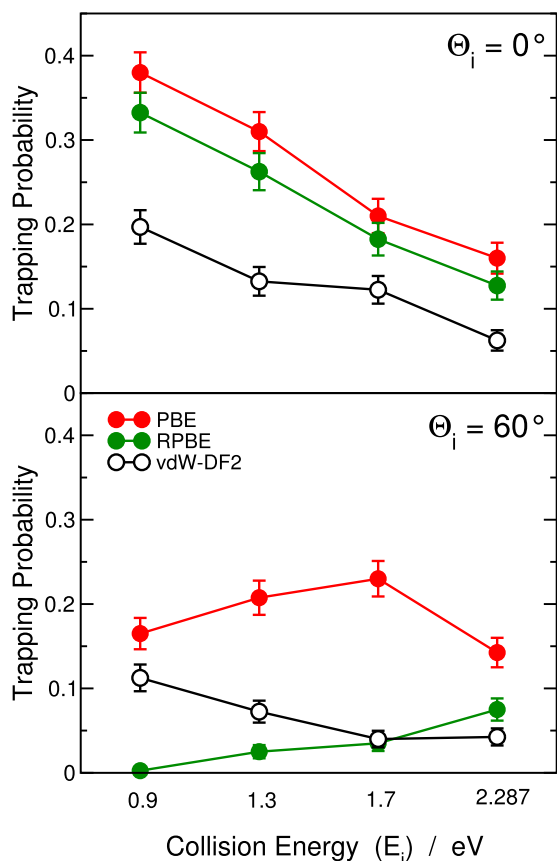
FIG. 14. Comparison between the trapping probabilities computed with the PBE, RPBE, and vdW-DF2 functional (reported as full red, full green, and empty black circles, respectively) for both \Theta_i = 0^\circ (top panel) and \Theta_i = 60^\circ (bottom panel).
