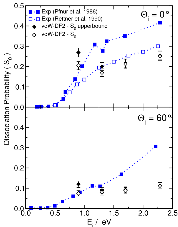
FIG. 8. Reaction probability as a function of the collision energy E_i for \Theta_i = 0^\circ (top panel) and \Theta_i = 60^\circ (bottom panel). Comparison between experimental data and AIMD vdW-DF2 results. The dissociation probabilities and their upperbounds are reported as empty and full black symbols, respectively. Experimental data are taken from Ref. 7 (full blue symbols) and Ref. 8 (empty blue symbols).
