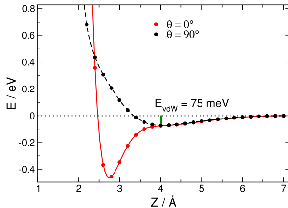
FIG. 4. 1D cuts of the potential as a function of the distance between the molecule's COM from the surface ( Z ) above a top site oriented either parallel ( \theta = 90^\circ ) or perpendicular ( \theta = 0^\circ ) to the surface. The zero of energy is the absolute energy of the molecule in the asymptotic configuration at gas phase equilibrium intramolecular distance ( r = r_e ).
