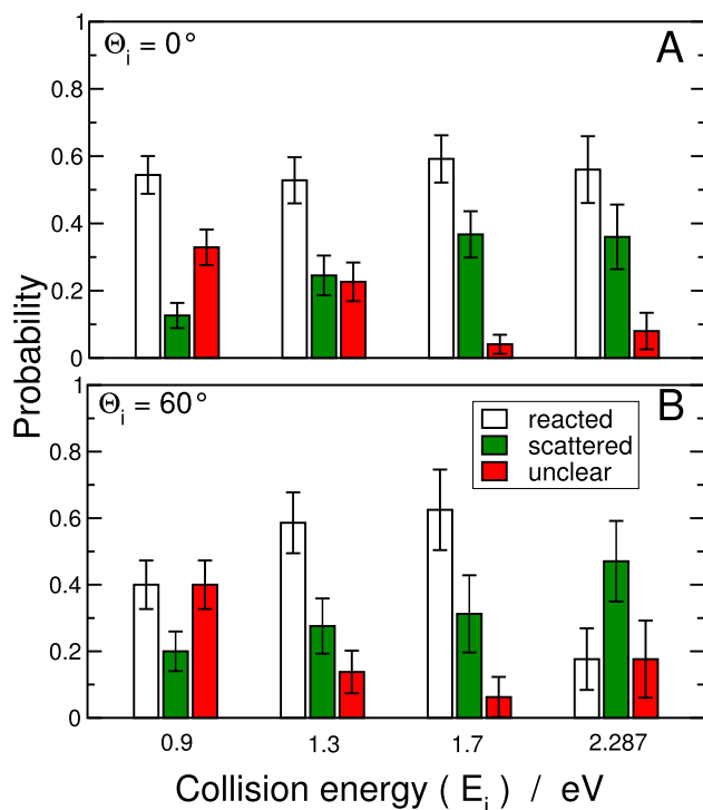
FIG. 15. The white, green and red bars represent the probabilities for a trapped molecule to dissociate, to scatter or to remain trapped (unclear outcome), respectively. The result reported is for \Theta_i = 0^\circ (panel (a)) and \Theta_i = 60^\circ (panel (b)).
