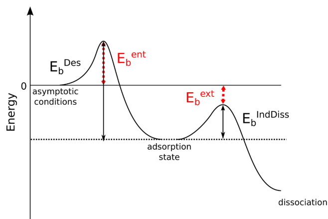
FIG. 1. Scheme of the barriers considered. The barrier for the desorption ( E_b^{Des} ) and the barrier for the indirect dissociation ( E_b^{IndDiss} ), represented as thick black lines are referred to the energy of the adsorption state. The entrance channel barrier for the molecular adsorption ( E_b^{ent} ) and the exit channel barrier for the dissociative chemisorption ( E_b^{ext} ), represented as red dashed lines, are referred to the asymptotic energy.
