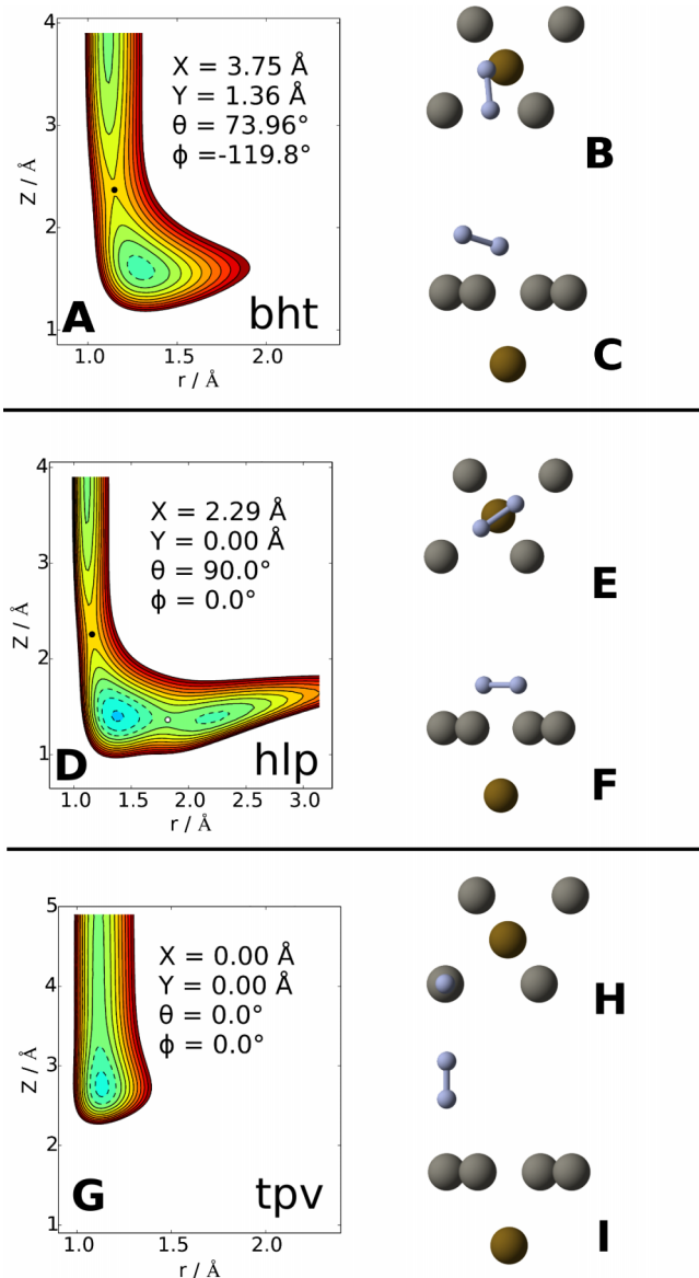
FIG. 3. Left: 2D ( r, Z ) cuts of the PES ((a), (d), (g)) computed for the three molecular adsorption geometries. Contour lines separate 0.2 eV energy intervals, solid lines are used for E \geq 0 eV and dashed lines for E < 0 eV. Circles indicate all the (first order) saddle points. The black circles represent the entrance channel barriers for molecular adsorption ( E_b^{ent} ) and the white circles are 2D saddle-points that are not real first order saddle-points in the 6D space (see text for details). Some details about the molecular adsorption geometries considered are reported as insets in the related plots. Right: top view ((b), (e), (h)) and side view ((c), (f), (i)) of the adsorption states. The 2D PES cuts are shown for the geometries bridge-hollow-tilted ((a)–(c)), hollow-parallel ((d)–(f)), and for top-vertical adsorption ((g)–(i)). The first layer atoms are shown in gray and the second layer atom closest to the molecule is shown in brown, the nitrogen atoms are shown in blue.
