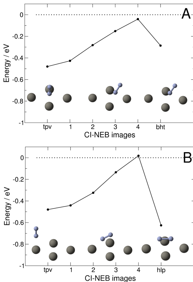
FIG. 5. Paths connecting two molecular adsorption states as obtained from CI-NEB calculations. The paths connect the top vertical state to either the bridge hollow tilted (a) or to the hollow parallel state (b). The zero of energy is the absolute energy of the molecule in the asymptotic configuration. The initial, the barrier and the final geometries are sketched as insets in the plots.
