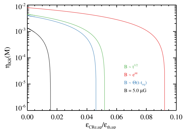
Figure 8. Required acceleration efficiency over pre-existing CRE energy density to match the observed relic. The pre-existing CRE energy density is shown in units of the upstream thermal energy density.
