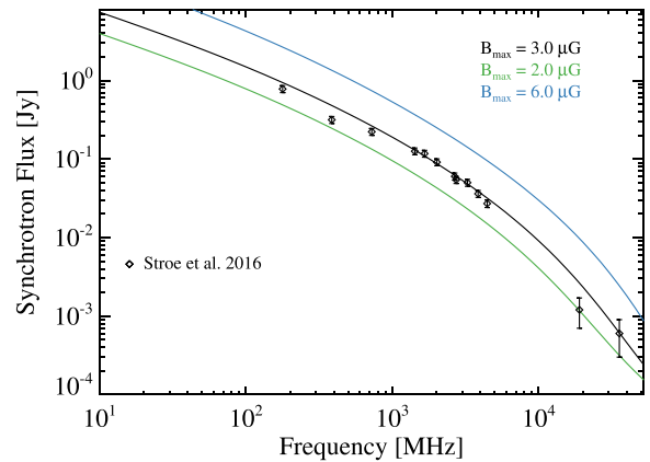
Figure C2. Beam convolved brightness profiles at 150 MHz and 610 MHz and integrated synchrotron spectrum (top to bottom) for the exponential model with maximum magnetic field B_{\max} equal to 3 \mu\text{G} (standard model, black), 2 \mu\text{G} (green) and 6 \mu\text{G} (blue).
