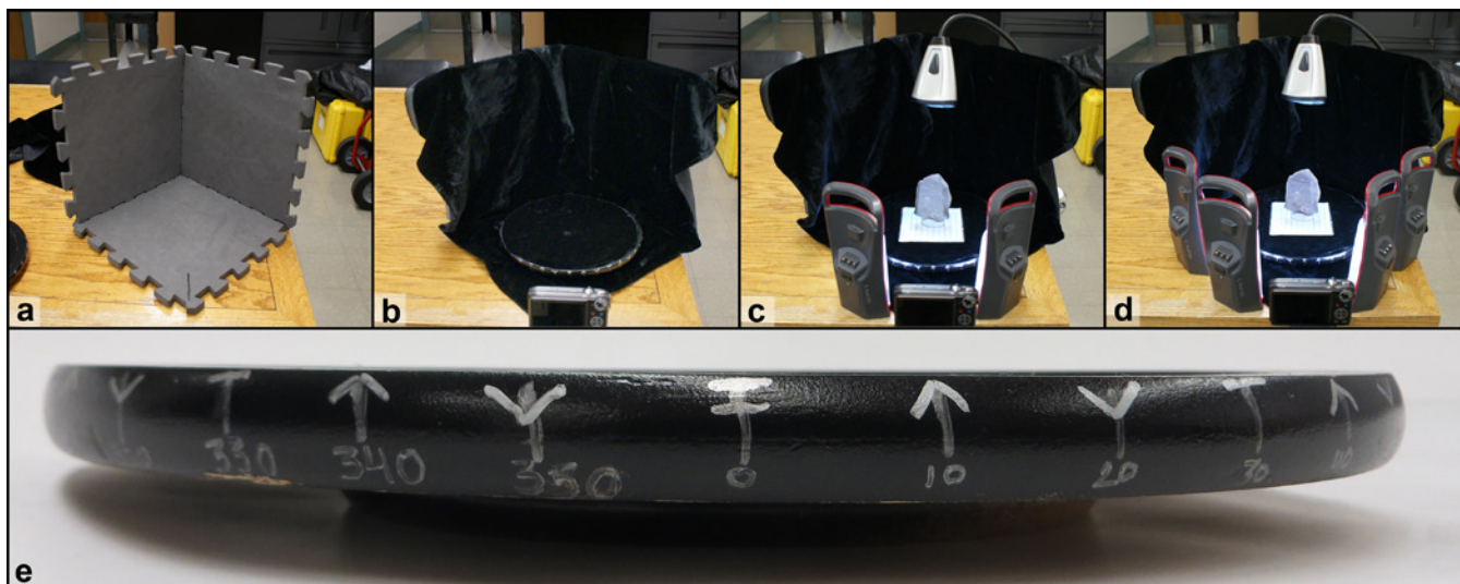
FIGURE 2. Setup and details of the portable photogrammetry rig described in this paper: (a) piecing together foam tiles; (b) addition of velvet backdrop, turntable covered with velvet, camera, and tripod; (c) addition of artifact, scale, overhead lamp, and two panel lamps; (d) four lamp version of the setup used when more side illumination is required; (e) detail of the turntable edge showing, T, ↑, and Y-shaped symbols used to denote object orientations to be captured during the first, second, and third rotations of photo-taking.
