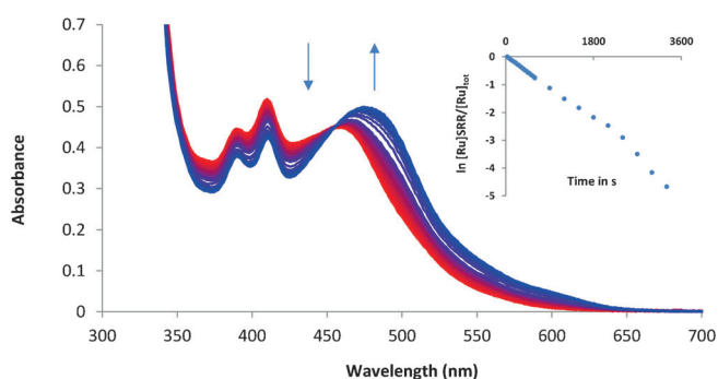
Figure 2. Electronic absorption spectra of [D-2][PF_6]_2 in deoxygenated H_2O irradiated at for 60 min. Spectra were taken every 30 s for the first 10 min, and then every 5 min until 60 min. T = 298 K, [Ru]_{tot} = 4.23 \times 10^{-5} , \lambda_{exc} = 450 nm, photon flux = 1.77 \times 10^{-7} Einstein s^{-1} . Insert depicts the evolution of \ln[RuSRR]/[Ru]_{tot} vs. irradiation time (s), where [RuSRR] is the concentration of [2]^{2+} at irradiation time t and [Ru]_{tot} the total ruthenium concentration.
