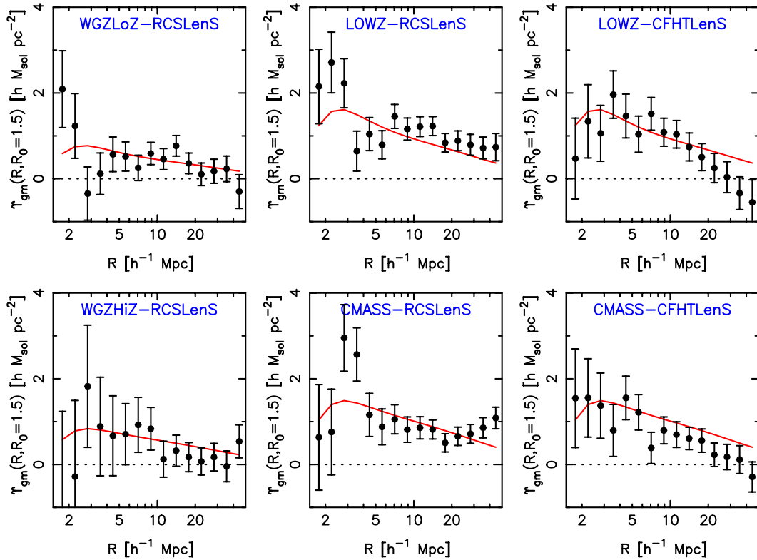
Figure 14. The ADSD statistic for the galaxy–mass cross-correlation, \Upsilon_{\text{gm}}(R, R_0) , measured for the different combinations of lens–source data sets assuming R_0 = 1.5 h^{-1} Mpc. We also plot the best-fitting model for each cross-correlation using both the w_p(R) and \Delta\Sigma(R) measurements. The errors are based on measurements for a set of 374 mock catalogues. The horizontal dotted line marks \Upsilon_{\text{gm}} = 0 .
