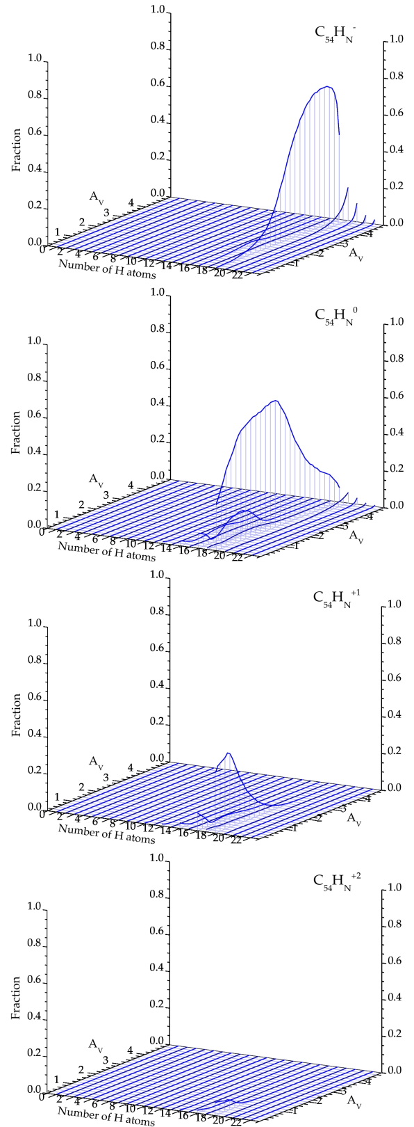
Fig. D.2. Fractional contribution from circumcoronene derivatives in the NW PDR of NGC 7023 according to the physical conditions modelled by the Meudon PDR Code. Unlike coronene, these molecules are found in their normally hydrogenated state ( N_{\text{H}} = 18 ) with traces of partial dehydrogenation at the surface of the cloud, and at A_{\text{V}} \sim 1.8 . No contribution from trications is observed.
