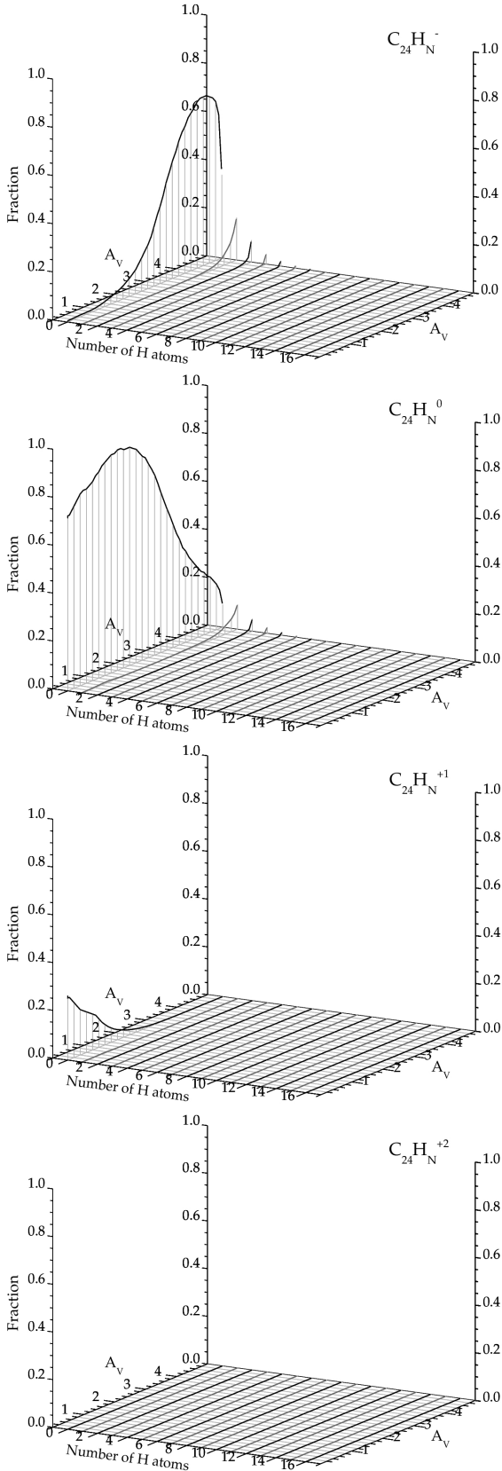
Fig. D.1. Fractional contribution from coronene derivatives in the NW PDR of NGC 7023 according to the physical conditions modelled by the Meudon PDR Code. Coronene is completely dehydrogenated throughout most of the cloud ( N_{\text{H}} = 0 ). No contribution from dicationic species is observed.
