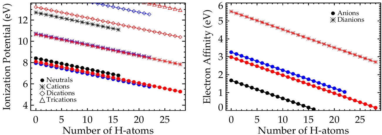
Fig. 4. Ionization potentials and electron affinities assumed in our model. Energies for coronene, circumcoronene and circumcircumcoronene derivatives are shown in black, blue and red, respectively. Given that PAHs in our model can absorb photon energies up to 13.6 eV, the highest charge state for coronene derivatives is the doubly charged one ( Z = 2 ). Circumcoronene derivatives can be doubly ionized, and only those having more than 12 H atoms can be triply ionized ( Z = 3 ). Circumcircumcoronene derivatives on the other hand can be triply ionized, and those having more than 22 H atoms can be found in the +4 charge state. Given the uncertainty in the electron affinities for highly negative charge states ( Z < -1 ), we do not take into account that the more dehydrogenated molecules could also exist in these highly negative states (e.g., Z = -2 for circumcoronene derivatives).
