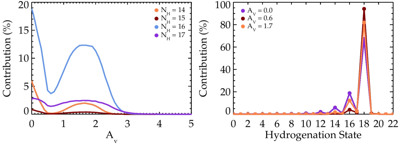
Fig. 7. Left panel: relative contribution of dehydrogenated states of circumcoronene as a function of depth into the cloud, A_V . The contributions consider all ionization states at which the molecules are present. The curves are shown for the first 4 dehydrogenated states of the parent molecule ( N_H = 17-4 ). Other partially dehydrogenated states contribute in smaller fractions. Right panel: distribution of circumcoronene derivatives at different A_V values where partially dehydrogenated species are observed.
