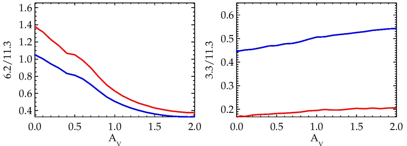
Fig. 11. PAH band ratios in the NW PDR of NGC 7023. The 6.2/11.3 ratio is usually used as a proxy for the ionization level of the PAH population, while the 3.3/11.3 ratio is expected to trace PAH size. Here we have plotted them for circumcoronene in blue, and circumcircumcoronene in red. The spectra for C 96 H 24 derivatives are complete in this A V range. The spectra for C 54 H 18 species are missing only the small contributions from partially dehydrogenated species (read text). Observational studies have derived typical 3.3/11.3 ratios of 0.5 to 0.3 from the surface to the PDR up to distances of about 52 arcsec from the star. As seen in the figure, intermediate size PAHs could potentially reproduce these values. However, the ionization ratio 6.2/11.3 would then be highly underestimated compared to the observations that predict a value of 2 at the surface of the PDR, decreasing in about 14% to a distance of ~55 arcsec from the star.
