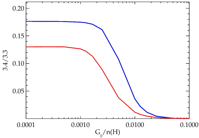
Fig. 12. Hydrogenation ratio for different G_0/n(\text{H}) values. The ratios derived from circumcoronene derivatives are shown in blue, while those from circumcircumcoronene derivatives are shown in red. We have assumed a gas temperature of 50 K, and that the fraction of atomic hydrogen is 10% that of molecular hydrogen, in order to model more shielded environments. The 3.4/3.3 ratio traces the superhydrogenation level of the PAHs as the 3.4 \mu\text{m} band is related to the stretching modes of the pair of \text{CH}_2 complexes within the same ring (which are duo rings for the coronene family). Observed 3.4/3.3 ratios in NGC 7023 range between 0.028 and 0.13, starting from the cavity and going into the NW PDR region, where G_0 is expected to vary from 7000–150 (Pillari et al. 2015). We see that these ratios can be achieved with superhydrogenated species but for G_0/n(\text{H}) ratios of 0.002–0.006, which is lower than what is expected in the NW PDR of NGC 7023.
