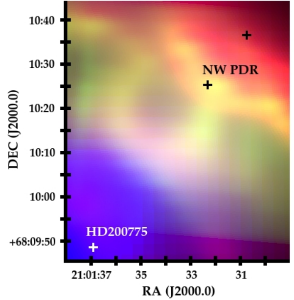
Fig. 2. Composite image of the NW PDR of NGC 7023. The three-color image combines the PACS 70 \mu\text{m} (red), PAH emission at 6.2 \mu\text{m} (green, image courtesy of O. Berné), and MIPS 24 \mu\text{m} (blue) images. The white cross indicates the position of the star HD 200775, while the black crosses indicate the reference extension of the NW PDR (at 45'' and 60'' away from the star).
