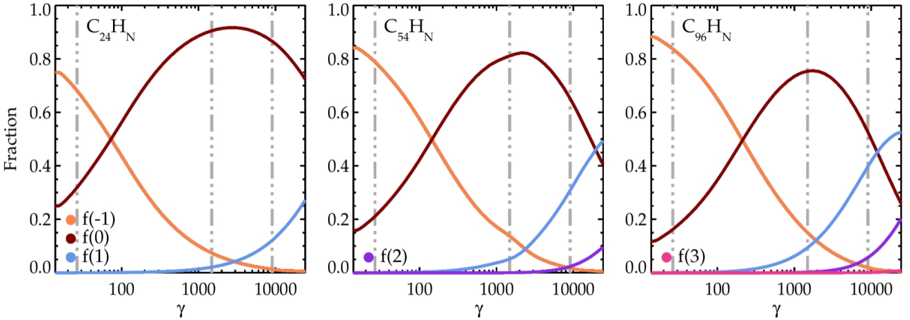
Fig. 8. Charge distribution of the PAHs considered in our study. The contribution from each ionization state is shown as a function of the ionization parameter \gamma \equiv G_0 \sqrt{T_{\text{gas}}/n(e)} for coronene ( left panel ), circumcoronene ( middle panel ) and circumcircumcoronene ( right panel ) derivatives. The color scheme is the same for all panels. Dashed grey lines are at A_V = 1, 2 and 4 . As observed from the panels, the main charge states throughout the cloud are the neutrals ( Z = 0 ), anions ( Z = -1 ) and cations ( Z = 1 ). Higher positively charged states are only present in minor levels at the surface of the NW PDR of NGC 7023. Higher anionic states ( Z < -1 ) are not observed.
