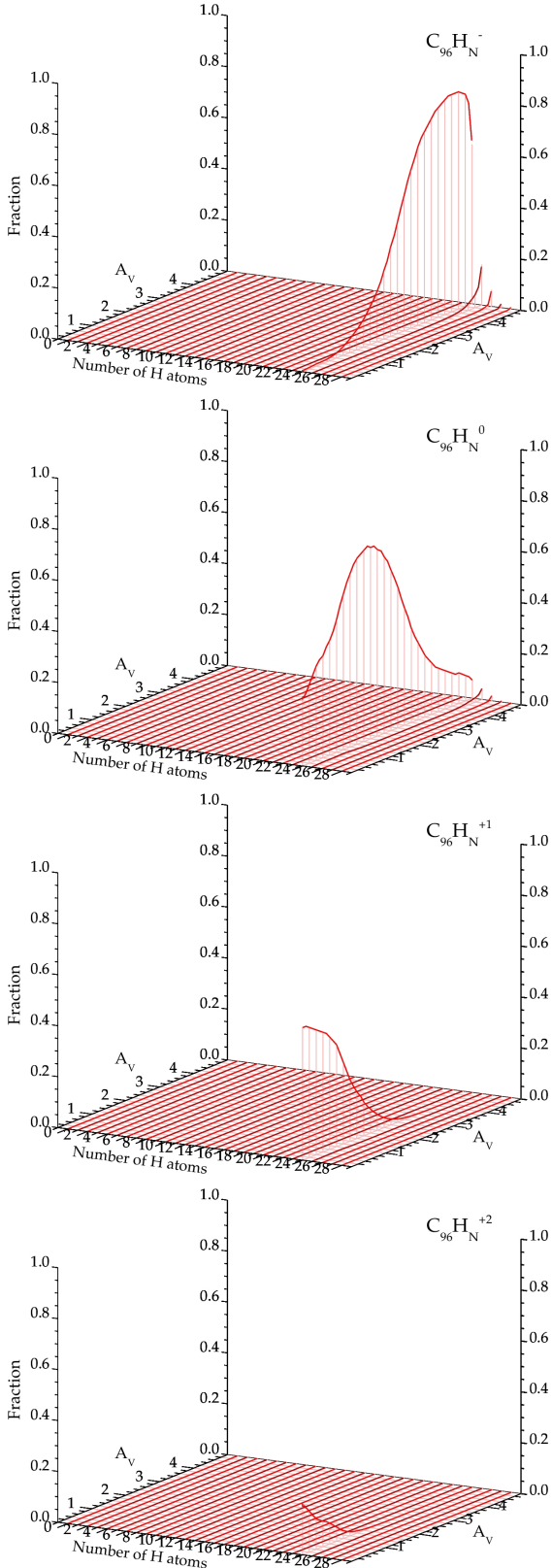
Fig. D.3. Fractional contribution from circumcircumcoronene derivatives in the NW PDR of NGC 7023 according to the physical conditions modelled by the Meudon PDR Code. Compared to the smaller species, circumcircumcoronene is mainly found in its normal hydrogenated state ( N_{\text{H}} = 24 ). There is no significant contribution from Z > 2 species (trications contribute in only 0.9% at A_V = 0 ).
