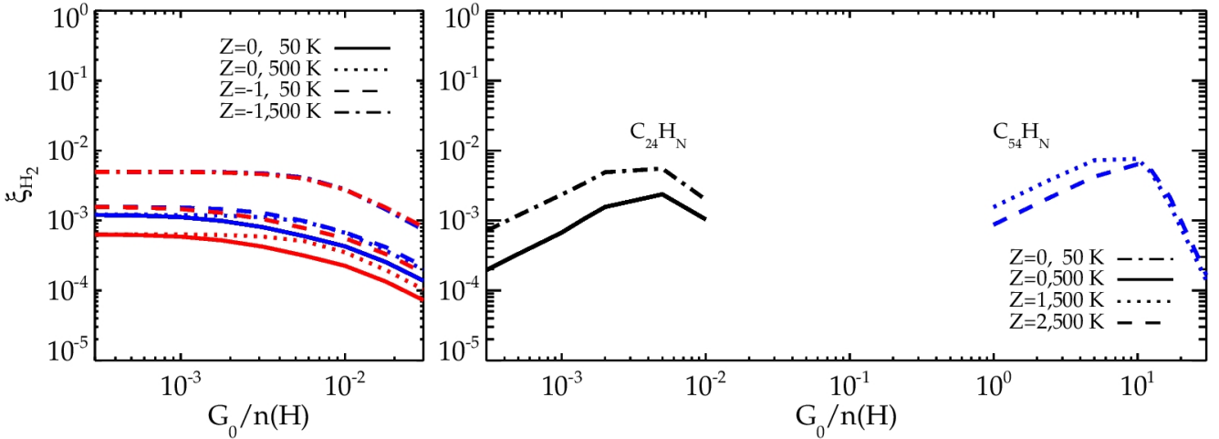
Fig. 10. Efficiencies of H 2 formation from PAHs. The left panel shows the efficiencies of H 2 formation through Eley-Rideal abstraction from superhydrogenated species as a function of G_0/n(\text{H}) . Estimates for circumcoronene and circumcircumcoronene superhydrogenated species are shown in blue and red, respectively. The efficiencies have been derived for neutrals and anions, since these are the charge states at which superhydrogenated species can be found according to our model. Two gas temperatures have been assumed as a reference. The right panel shows the efficiencies of H 2 formation from photodissociation of PAHs. The efficiencies have been derived for neutral coronene at G_0 = 10 , and Z > 0 circumcoronene at G_0 = 10^3 . We have considered different G_0 values due to the different dehydrogenation behaviour of the species in the G_0 - n(\text{H}) parameter space (see Fig. 9). As it can be derived from the figure, efficiencies stay below 1% for both mechanisms.
