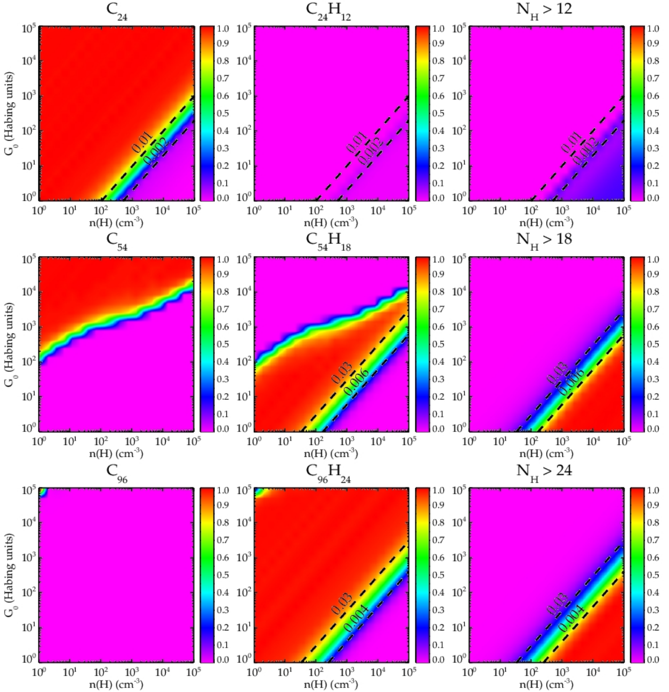
Fig. 9. Fractional contribution from coronene ( top panels ), circumcoronene ( middle panels ) and circumcircumcoronene ( bottom panels ) derivatives for different G_0 and n(\text{H}) values. The contributions include all ionization states. The left column shows the contribution from the completely dehydrogenated molecules, \text{C}_{24} , \text{C}_{54} and \text{C}_{96} ; the middle column shows the fraction of the normally hydrogenated molecules; and the right column shows the distribution of the superhydrogenated species. In all cases, we have assumed a fraction of molecular hydrogen of 0.5, and a carbon abundance of 3.5 \times 10^{-4} relative to hydrogen. Black lines represent constant G_0/n(\text{H}) ratios and are given as a reference.
