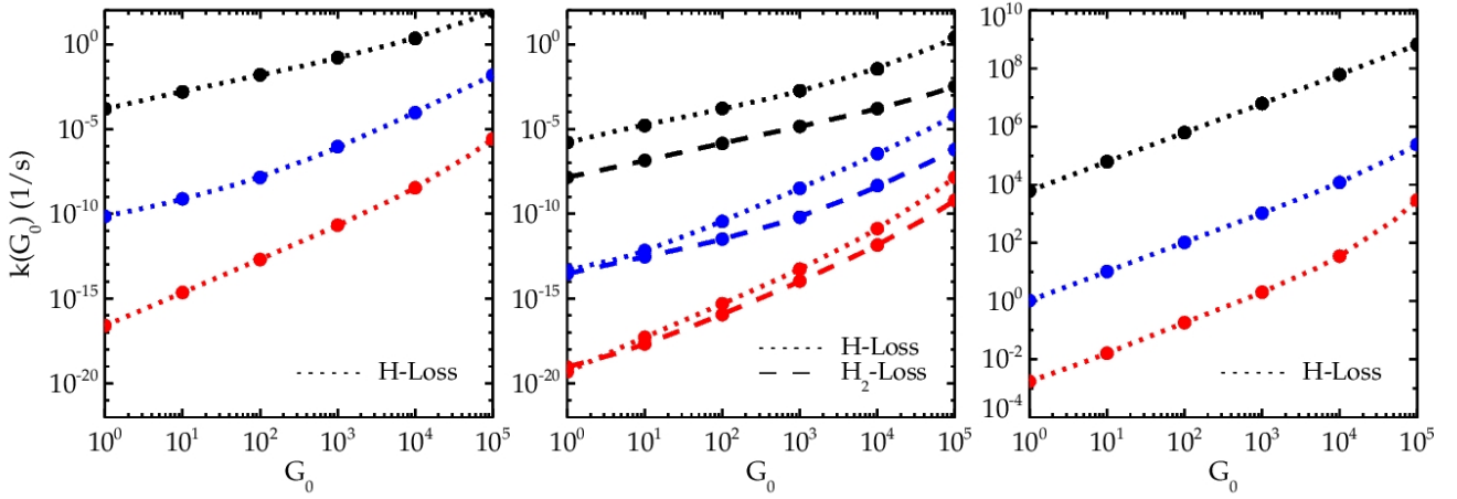
Fig. 6. Variation of the photodissociation rates with respect to the intensity of the UV field, G_0 . The rates are shown for the same molecules as in Fig. 5, following the same color scheme. For the smallest molecule (black curves) the rates scale linearly with G_0 at the range of interest for NGC 7023 ( G_0 \leq 2600 ) indicating single photon events occurrence for coronene derivatives. For the larger molecules, multiphoton events are important. Even though H-loss is the dominant dissociation channel, at low G_0 values, H 2 -loss can become a competitive process for the larger circumcoronene and circumcircumcoronene species.
