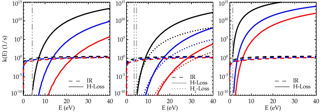
Fig. 5. Comparison of IR emission and photodissociation rates as a function of internal energy of the PAH. The rates determined for coronene derivatives are shown in black, while the rates for circumcoronene and circumcircumcoronene are shown in blue and red respectively, following the color scheme of Fig. 4. The grey vertical lines show the activation energies assumed listed in Table 2. The left panel shows the rates for the first dehydrogenated state of each parent molecule in their neutral state ( C_{24}H_{11}^0 , C_{54}H_{17}^0 and C_{96}H_{23}^0 ), in order to exemplify the rates for molecules with an odd number of H atoms. The middle panel shows the rates for the parent neutral molecules, illustrating the H and H_2 -loss rates for PAHs with an even number of H atoms. The right panel shows the rates for the first superhydrogenated state of the neutral molecules (i.e., C_{24}H_{13}^0 , C_{54}H_{19}^0 , and C_{96}H_{25}^0 ) for which no direct H_2 -loss is considered. IR emission rates as a function of internal energy, k_{IR}(E) , have been calculated using the IR cross sections of each molecule whenever available (see Appendix A). For C_{24}H_{11}^0 and C_{96}H_{23}^0 we have assumed the intrinsic frequencies of the parent molecules.
