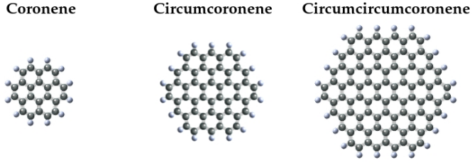
Fig. 1. PAHs studied in this work. From left to right: coronene (C 24 H 12 ), circumcoronene (C 54 H 18 ) and circumcircumcoronene (C 96 H 24 ). The carbon cores are depicted in grey, while H atoms are depicted in white.
