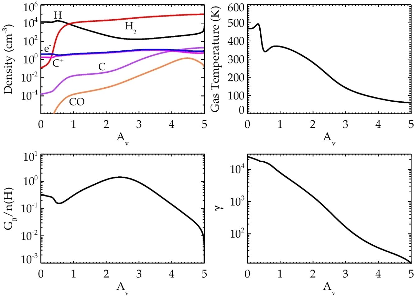
Fig. 3. Physical conditions in the NW PDR of NGC 7023. The top panels show the variation of the densities and gas temperature inside the cloud. The HI to \text{H}_2 transition occurs at an A_V \sim 0.9 , while the CII–CI transition occurs deeper in the cloud at an A_V \sim 4 . The bottom panels show the physical parameters relevant for PAH hydrogenation and ionization evolution. The hydrogenation of PAHs is expected to be controlled by the ratio between the UV field intensity G_0 and the density of atomic hydrogen, which in our case only varies by about 2 orders of magnitude throughout the cloud. The ionization state of the PAH population on the other hand depends on the so-called ionization parameter, \gamma \equiv G_0 \sqrt{T_{\text{gas}}/n(e)} , which measures the ratio between ionization and electron recombination of the PAH species.
