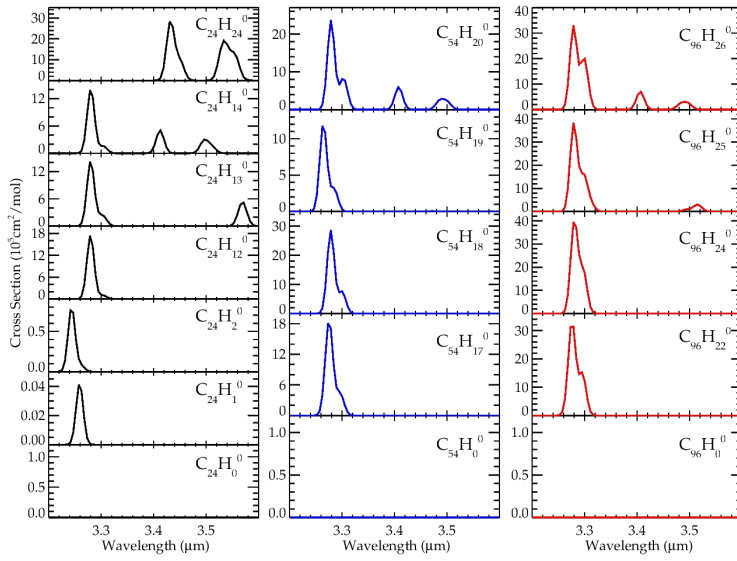
Fig. F.3. Intrinsic spectra of different hydrogenation states of the neutral coronene ( left ), circumcoronene ( middle ) and circumcircumcoronene ( right panel ) molecules. Only the 3 \mu\text{m} region is presented. This spectral region is the one where differences in the hydrogenation state of PAHs can be clearly observed. Differences in the hydrogenation state (within a given PAH size and ionization state) are clear from the appearance of more features at 3.4 and 3.5 \mu\text{m} .
