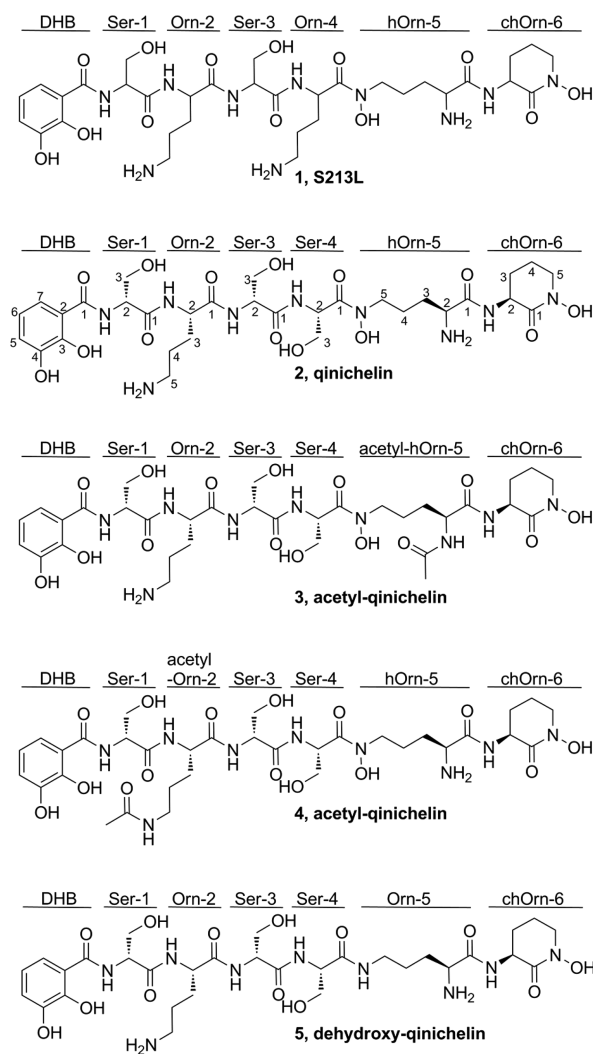
Figure 2. Molecular structures of S213L (1), qinichelin (2), acetyl-qinichelin (3,4), and dehydroxy-qinichelin (5). Abbreviations of moieties are shown to facilitate the comparison of respective structure. DHB, dihydroxybenzoate; Ser, serine; Orn, ornithine; hOrn, \delta - N -hydroxy-ornithine; chOrn, cyclized \delta - N -hydroxy-ornithine hydroxamate. Acetylation of qinichelin can occur on two positions as indicated. The shown configurations of DHB– D -Ser– L -Orn– D -Ser– L -Ser– L -hOrn– L -chOrn in qinichelins were based on Marfey's protocol (Supporting Information data and Figures S10–S15) combined with biosynthetic considerations (see Figure 5).
