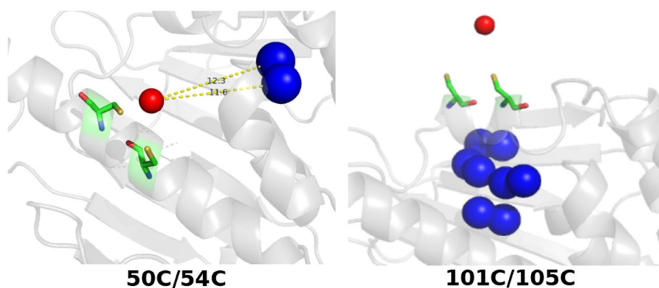
Fig. 9 Highly reliably assigned methyl groups, represented in blue spheres, using a single paramagnetic center for the assignment. The numbers in the 50C/54C panel indicate the distances from the lanthanoid to the methyl groups in Å
