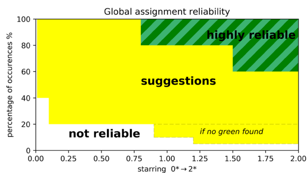
Fig. 5 Assignment reliability. The average quality score from the 100 assignment runs is indicated on the horizontal axis and the occurrence percentage of the runs in which the assignment is found is plotted vertically. Dark and light green refer to stereospecific and non-stereospecific assignment of Leu and Val methyl groups
