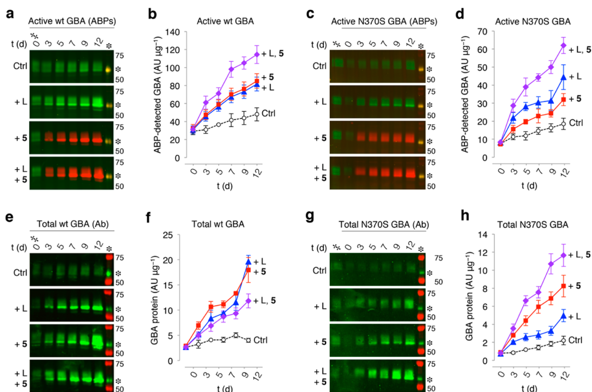
Figure 5. In situ stabilization of GBA by ABP 5 and leupeptin. Wild-type GBA fibroblasts were incubated with leupeptin, ABP 5 (red), or both for the indicated lengths of time. (a) GBA levels in untreated fibroblasts (top row) and cells incubated with leupeptin (second row), visualized in vitro with ABP 4 (green). Labeling of GBA in cells in situ with ABP 5 (red, third row) and in combination with leupeptin (bottom row). Equal green and red fluorescence yields a yellow overlay; fluorescence was calibrated with 50 fmol of equimolar green ABP 4- and red ABP 5-labeled imiglucerase present in each SDS-PAGE gel (asterisk). (b) Quantification of ABP-emitted fluorescence from in vitro ABP 4-labeled controls (open black circles), cells treated with leupeptin only (blue triangles), cells treated with in situ ABP 5-labeled GBA (red squares), and cells treated with a combination of ABP 5-labeled GBA and leupeptin (purple diamonds). Data are the mean of n = 2 \pm \text{SD} . (c) GBA levels in N370S/N370S fibroblasts treated in the same manner as wild-type GBA fibroblasts in panel a, vide supra . (d) Quantifications of ABP fluorescence in N370S/N370S fibroblasts. (e) Detection of total GBA protein in wild-type fibroblasts (green) by western immunoblotting of gels depicted in panel a (molecular weight ladder is in red). (f) Quantification of total GBA protein from in vitro ABP 4-labeled controls (open black circles), cells treated with leupeptin only (blue triangles), cells treated with in situ ABP 5-labeled GBA (red squares), and cells treated with a combination of ABP 5-labeled GBA and leupeptin (purple diamonds). Data are the mean of n = 2 \pm \text{SD} . (g) Total GBA protein in N370S/N370S fibroblasts treated in the same manner as wild-type GBA fibroblasts in panel a, vide supra . (h) Quantifications of ABP fluorescence in N370S/N370S fibroblasts. All data are expressed as average of n = 2 \pm \text{SD} .
