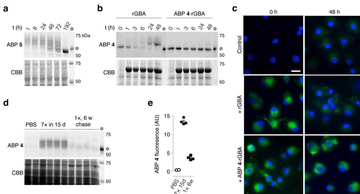
Figure 4. In situ labeling of GBA with cyclophellitol ABPs 4 and 5. (a) Continuous labeling of human monocyte-derived macrophage GBA with ABP 5 (top) and Coomassie brilliant blue (CBB) staining of protein input (bottom). (b) Chase of ABP 4 (pre-) labeled rGBA (imiglucerase) taken up by CBE 2 pretreated human monocyte-derived macrophages (top) and CBB staining (bottom). (c) Fluorescence micrographs of macrophages in (c): control (top) and cells treated with unlabeled rGBA (middle) and ABP 4-labeled rGBA (bottom) after 0 and 48 h (left and right, respectively). Unlabeled rGBA was detected by labeling for 30 min with 10 nM ABP 4 prior to fixation. Scale bar represents 25 \mu\text{m} . (d) Chase of murine hepatic (endogenous) GBA of animals treated either with vehicle, ABP 4 for 15 days (7 injections), or a single dose 6 weeks prior to sacrifice (top) and CBB staining (bottom). (e) Densitometry of ABP 4-emitted fluorescence from (d), normalized using CBB, with no treatment (open circles) or treated with repeated doses of ABP 4 (closed diamonds) or a single dose (closed squares); data are the mean of duplicate quantifications \pm SEM. All gels contain 50 fmol of equimolar ABP 4- and 5-labeled \sim 59 kDa imiglucerase (asterisk) as a positive control.
