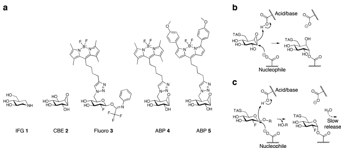
Figure 1. Inhibitors and reaction mechanism. (a) Structural formulas of competitive, reversible inhibitor isofagomine (IFG 1), irreversible inhibitors conduritol \beta -epoxide (CBE 2), semi-irreversible inhibitor 2-deoxy-2-fluoro- \beta -D-glucopyranosyl- N -phenyltrifluoroacetimidate 33 (fluoro 3), cyclophellitol \beta -epoxide type ABP 4 (MDW933, green fluorescent), and \beta -epoxide-type ABP 5 (MDW941, red fluorescent). 35 (b) Irreversible binding mechanism of \beta -epoxide-type ABPs to the nucleophile of GBA via its double-displacement mechanism. (c) Hydrolysis of fluoro 3 and temporary trapping of the glycosylated nucleophile adducts of GBA.
