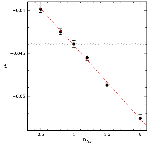
Figure 5. Multiplicative bias for galaxies with magnitude 20 < m < 24.5 as a function of n_{\text{fac}} , the relative increase in the number density of galaxies brighter than magnitude 26. For reference, the hatched region indicates a variation in \mu of size 10^{-4} .
