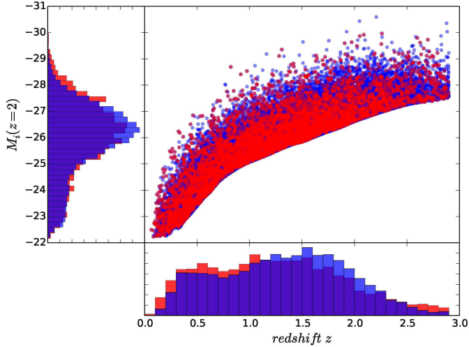
Fig. 4. Distribution of RLQs (red) and RQs (blue) in the optical-luminosity space. The absolute magnitude in the i -band at z = 2 M_i(z = 2) is calculated using the K -correction from Richards et al. (2006). The left and bottom panels show the M_i(z = 2) and redshift histograms. The normalized redshift and optical-luminosity distributions are displayed in the left and bottom panels. The normalized distributions for both samples show a good degree of similarity, allowing a direct comparison of their clustering measurements.
