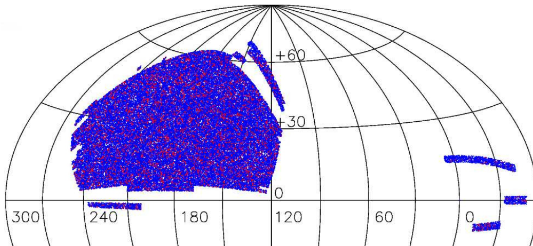
Fig. 2. Aitoff projection for the sky coverage of the SDSS DR7 uniform quasar sample from Shen et al. (2011). RQQs are denoted by blue points, while the RLQs are represented by red points. See Sect. 2 for a description of the methodology employed in the selection for the RLQs.
