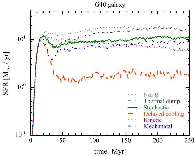
Figure 3. SFRs, as in Fig. 2, but for the more massive and lower resolution G10 galaxy (note that the y-axis is scaled up by a factor of 10). Here, we find larger differences between thermal dump, stochastic and mechanical feedback, while kinetic feedback and delayed cooling remain qualitatively the same as in the less massive galaxy.
