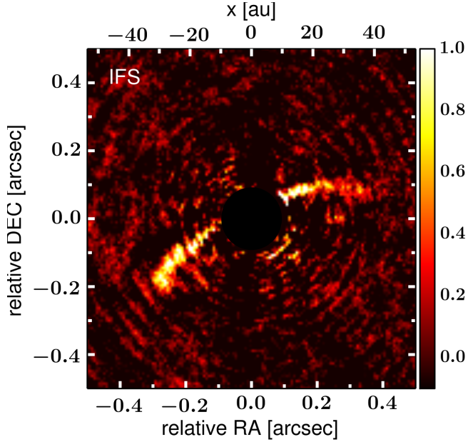
Fig. 4. IFS image after PCA+SDI reduction with 100 modes: median across the entire wavelength range \lambda . North is up, east is toward the left; the image is normalized to the highest disk brightness and the color scale considers the same dynamical range as in Fig. 3. The inner 0''.18 region masked by the coronagraph is represented by the black circular area.
