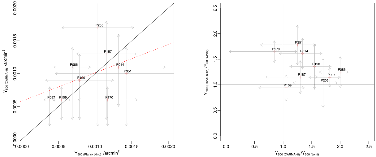
Figure 7. Left: Y_{500} measured by CARMA-8 against the blind Planck Y_{500} . No strong bias indications are detected between the Planck , blind and CARMA-8 Y_{500} results. The best-fitting (red, dotted) and 1:1 (black, solid) lines are included in this plot. Right: ratio of the Planck , blind Y_{500} and the joint Y_{500} values against the ratio of the CARMA-8 Y_{500} and the joint Y_{500} . For Y_{500} , both the CARMA-8 and Planck , blind values are practically always higher than the joint values by as much as a factor of 2.
