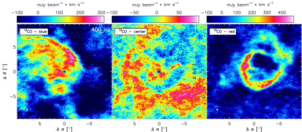
Figure 3. Moments 0 maps of the ^{12}\text{CO} line. The blueshifted side of the velocities (left), the low-velocity side (centre) and the redshifted side (right) are shown. We divided the three parts following the velocity ranges listed in Table 2. The beam size is \sim 0.25 arcsec, shown on the lower-left corner of the image. The continuum is shown in blue contour map.
