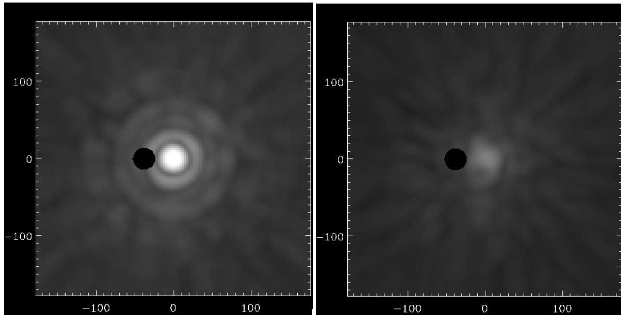
Fig. 2. Left: realistic simulation of a SPHERE AO-corrected image in the 600–780 nm band, centered on the star. The dark hole indicates the position and size of an optical fiber that would pick up the planet light to send it to ESPRESSO. The planet is 37 mas away from the star ( 2.0 \lambda/D at 750 nm), while the fiber radius is 14 mas. Right: coronagraphic image, limited by the aberrations of the incoming beam (both turbulence residuals and optical defects), assuming an ideal coronagraph. Units on both axes are milli-arcseconds (mas).
