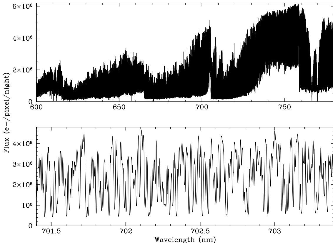
Fig. 4. PHOENIX high-resolution spectrum simulating an observation of Proxima with SPHERE+ESPRESSO. The total integration time is eight hours. Top : the 600–780 nm region, which would be used for SPHERE+ESPRESSO observations. Bottom : close-up view showing the very high density of spectral lines in this star.
