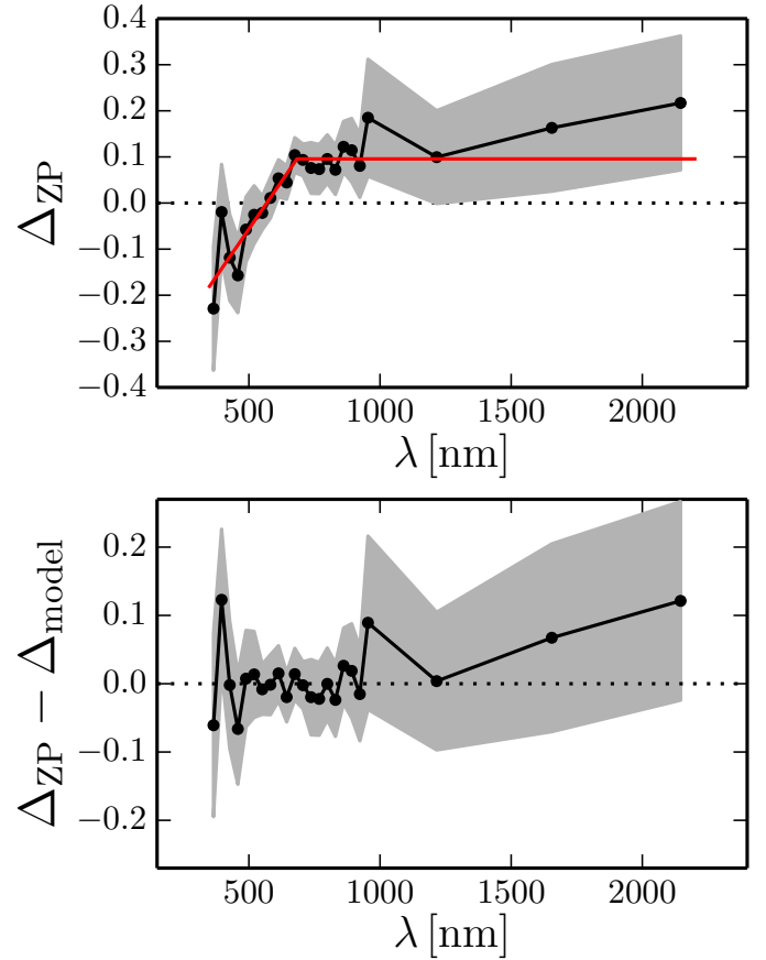
Fig. A.2. Top panel: median zero point correction \Delta_{ZP} applied by BPZ2 to the original ALHAMBRA photometry (black points). The observed structure is modelled with a linear function and a constant value (red solid line). Bottom panel: residual zero point correction after removing the model from the median correction. The grey area in both panels shows the field-to-field dispersion of the correction.
