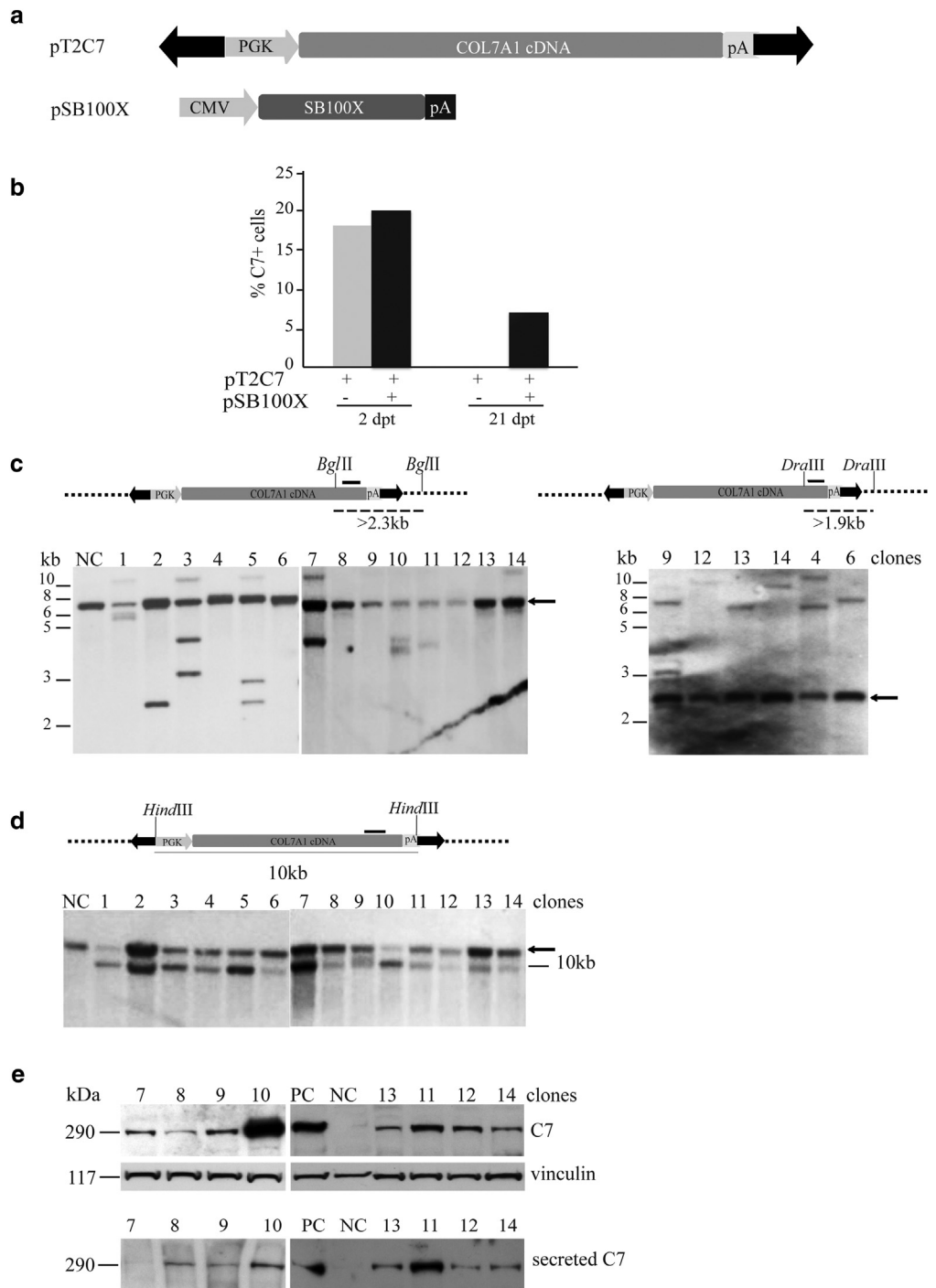
Figure 1. C7 transposition in iRDEB keratinocytes. (a) Schematic outline of pT2C7 and pSB100X plasmids. The black arrows represent the IR of the transposon. (b) pT2C7-transfected iRDEB in presence or in absence of pSB100X. C7 + cells scored by immunofluorescence 2 and 21 days after transfection. (c) Southern blot on iRDEB clones. Bgl III (left panel) and Dra III (right panel) digested DNA hybridized to a C7-specific probe. Dotted lines represent human genome. (d) Southern blot on iRDEB clones. Hind III digested DNA probed with a C7-specific probe. Black bars indicate C7-specific probe. Black arrows indicate endogenous signal. (e) Western blot analysis on total extracts (upper panel) and on culture supernatants (lower panel) of iRDEB-transposed clones. Vinculin represents internal loading control. CMV, cytomegalovirus; iRDEB, immortalized recessive dystrophic epidermolysis bullosa; NC, not treated; PC, wild-type keratinocytes; PGK, phosphoglycerate kinase.
