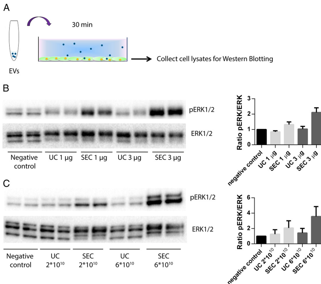
Figure 3. Assessment of UC-EV and SEC-EV functionality. (A) HMECs were stimulated with EVs for 30 min, after which phosphorylated ERK1/2 and total ERK1/2 protein levels were determined using Western blotting. (B) Stimulation of HMECs with equal amounts of UC-EV and SEC-EV protein. (C) Stimulation with equal numbers of UC-EV and SEC-EV particles. Abbreviations: ERK = extracellular signal-regulated kinase, SEC = size-exclusion chromatography, UC = ultracentrifugation.
