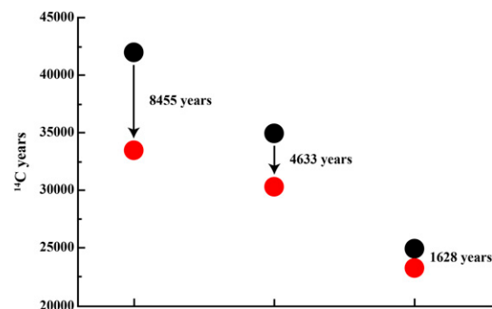
Fig. 1. Contamination effect on radiocarbon dates. The black dots represent three examples of radiocarbon dates without contamination, and the red dots represent the effect of only 1% contamination by modern carbon on the same samples.
