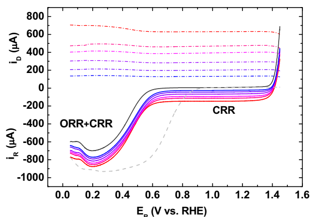
Fig. 2. LSV of the Pt ring electrode, while keeping the \text{IrO}_x/\text{GC} disk electrode at constant potential in 0.5 \text{ M KHSO}_4 + 100 \text{ mM KCl} , scan rate 5 \text{ mVs}^{-1} , rotation rate 1500 RPM. pH = 0.88, solution saturated with \text{O}_2 . Dotted curves with positive values correspond to disk currents, remaining curves correspond to ring currents. The ring LSV sweeps were taken in the positive-going direction. Disk potentials were chosen in the region of exclusive CER, with values increasing from the blue curve to the red curve, E_D = 1.449 \text{ V} , 1.456 \text{ V} , 1.462 \text{ V} , 1.467 \text{ V} , 1.470 \text{ V} , and 1.475 \text{ V} . Black curve shows ring response while disk is not connected. Grey dashed curve shows ring response while disk is not connected, in \text{Cl}^- -free conditions. (For interpretation of the references to color in this figure legend, the reader is referred to the web version of this article.)
