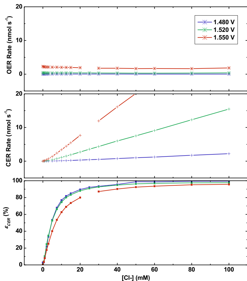
Fig. 5. Plots of OER and CER reaction rates as function of [Cl^-] , for three disk potentials: E_D = 1.480 V (blue lines), 1.520 V (green lines), and 1.550 V (red lines). Values were obtained from CVs identical to Fig. 1, while varying [Cl^-] . Rates were obtained by dividing currents by nF , the number of electrons transferred and Faraday's constant. (For interpretation of the references to color in this figure legend, the reader is referred to the web version of this article.)
