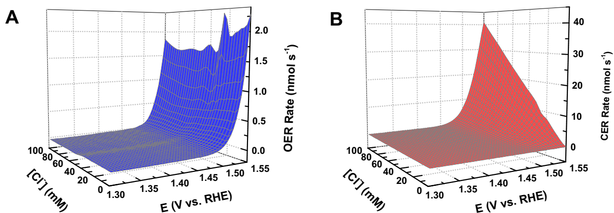
Fig. 6. Plots of A) OER rates and B) CER rates as function of E_D and [Cl^-] , constructed from CVs identical to Fig. 1, while varying [Cl^-] . Rates were obtained by dividing currents by nF , the number of electrons transferred and Faraday's constant.
