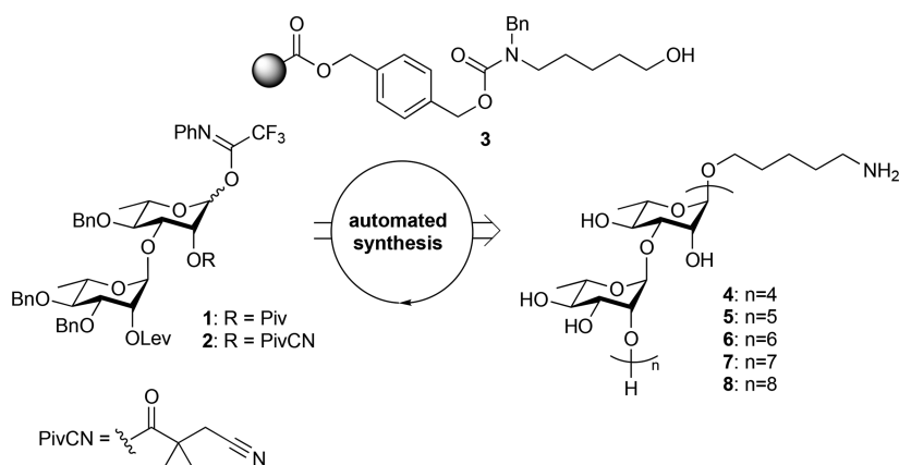
Figure 1. Synthetic approach described in this work.
