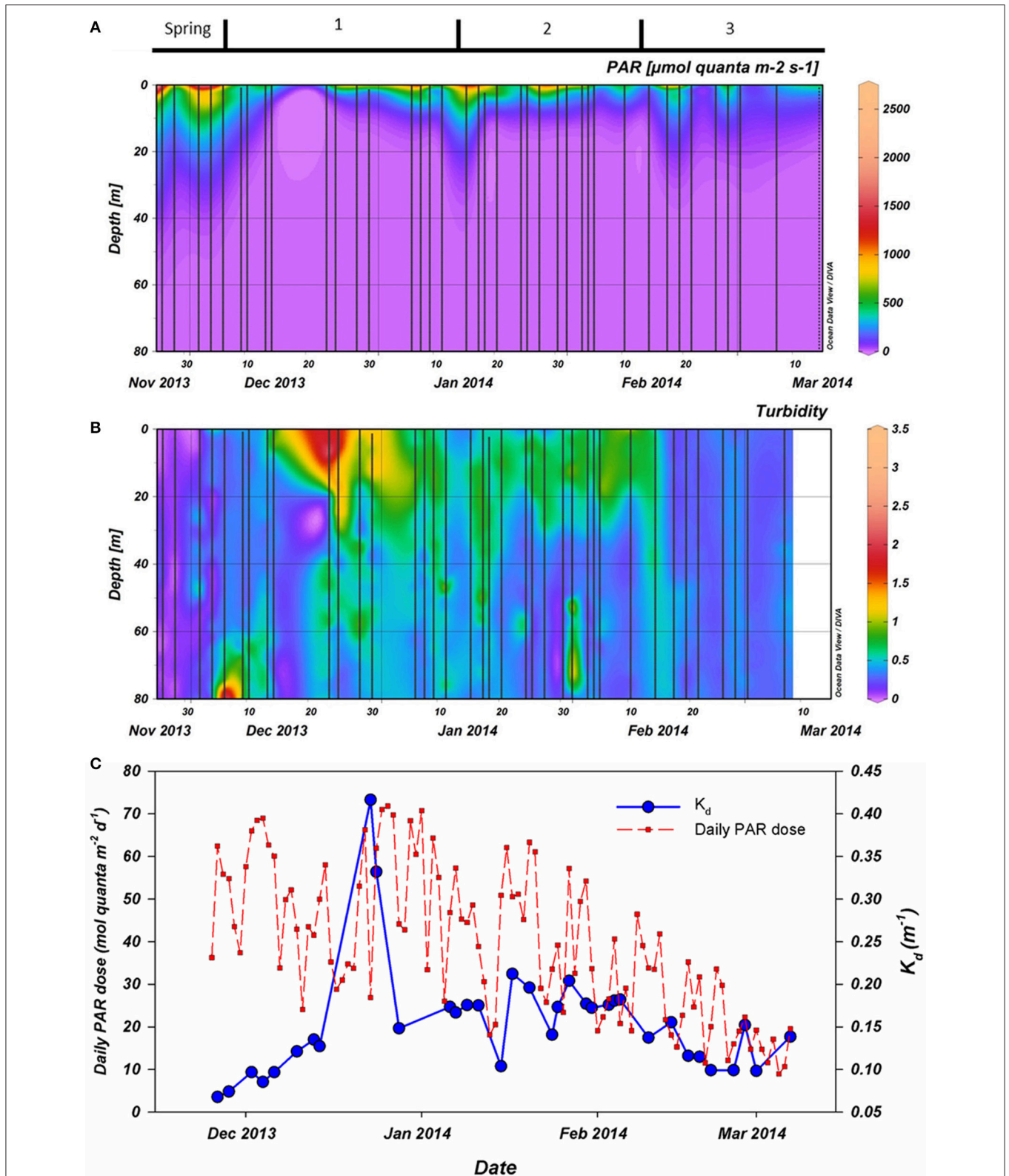
FIGURE 2 | (A): Photosynthetically active radiation (PAR) as measured during CTD casts (vertical casts). (B): Turbidity as also measured during the CTD casts. (C): First, the extinction coefficient ( K_d in blue) as calculated using the PAR data collected by CTD. Also, the daily irradiance dose for PAR (red) integrated from continuous measurement at Rothera station. All data were collected during the 2013–2014 season. Period 1 starts on December 6th, period 2 on January 15th and period 3 on February 10th.
