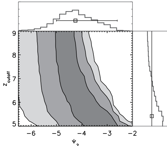
Figure 4. 68, 95, and 99.7% confidence intervals (represented by the contours in the gray-scale image) for the two parameters explored in this work to describe the evolution of the IRLF in the Casey et al. (2018b,a) models. The confidence intervals were determined by fitting the corresponding predicted number counts through a maximum likelihood approach. The derived probability distribution for each individual parameter is represented by the solid line in the external panels (top and right, respectively).
