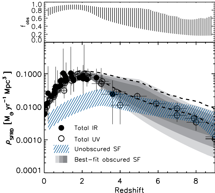
Figure 5. The cosmic star formation rate density as a function of redshift, comparing measurements from rest-frame UV/optical to the obscured component constrained by our 3 mm number counts. Black circles represent measurements from the literature from both dust-corrected UV (empty circles) and IR rest-frame (filled circles) studies (Madau & Dickinson 2014), which are dominated by UV surveys at z \gtrsim 3.5 . The implied star formation rate densities of the Casey et al. (2018b,a) models that best fit the measured 3 mm number counts are illustrated by the gray regions, where the darkest gray represents the 68% confidence interval (the 95, and 99.7% are plotted with lighter grays, respectively). On the other hand, the unobscured sources’ contribution derived from UV-based measurements, uncorrected by dust attenuation, is represented by the blue hashed region. The implied total (obscured + unobscured) CSFR is represented by the region delimited by the dashed black lines (68% confidence interval). Finally, the fraction of obscured star formation ( \text{SF}_{\text{IR}}/\text{SF}_{\text{UV+IR}} ) as a function of redshift derived from the best-fit model predictions is shown in the top panel.
