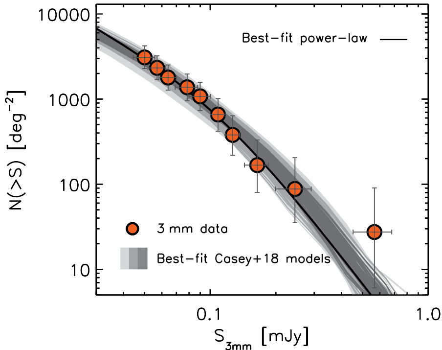
Figure 3. Integral galaxy number counts at 3 mm. The measurements derived in this work are represented by the red points and the best-fit broken power is plotted as the black solid line. We also plot the number counts from the Casey et al. (2018b,a) model when different evolutions on the IRLF are assumed, which are used to fit the data through a maximum likelihood estimation method. The 68, 95, and 99.7% confidence intervals for the best-fit models are color-coded from the darkest to the lightest gray, respectively. Their corresponding contributions to the cosmic star-formation rate density are plotted in Figure 5.
