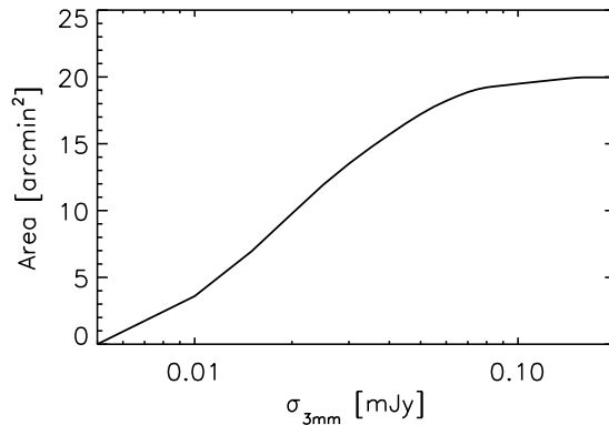
Figure A.1. Cumulative area covered by those ALMA maps with blind detections as a function of 1\sigma r.m.s. As it can be seen, the depths probed by these maps encompass a large range from \sim 6 to 100 \mu\text{Jy} .
