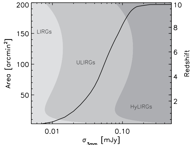
Figure 1. The cumulative area covered by our survey as a function of 1\sigma r.m.s. depth is represented by the black solid line. Additionally, the corresponding luminosity detection limit at 5\sigma is shown as a function of redshift assuming a typical DSFG SED (a gray body with T_D = 35 \text{ K} and \beta = 1.8 ), including the impact of CMB (da Cunha et al. 2013). Three luminosity ranges are illustrated: LIRGs ( 10^{11} \leq L_{\text{IR}} < 10^{12} L_{\odot} ), ULIRGs ( 10^{12} \leq L_{\text{IR}} < 10^{13} L_{\odot} ), and HyLIRGs ( L_{\text{IR}} \geq 10^{13} L_{\odot} ). Given the strong negative K -correction in the 3 mm band, we are sensitive to galaxies with L_{\text{IR}} \gtrsim 10^{12} - 10^{13} L_{\odot} up to z \sim 10 .
