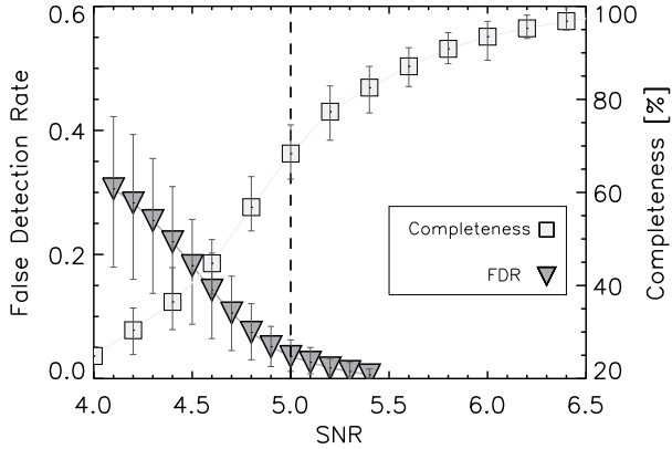
Figure 2. Estimated contamination from spurious sources (dark gray triangles) and completeness (light gray squares) and as a function of SNR of the detected sources. The 5\sigma adopted threshold is represented by the dashed vertical line, where the false detection rate and completeness are expected to be \lesssim 5\% and \gtrsim 70\% , respectively.
