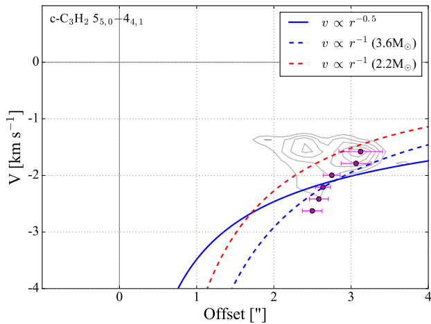
Fig. 10. Position-velocity diagram for c\text{-C}_3\text{H}_2 5_{5,0}-4_{4,1} towards the disk-like structure direction ( \text{PA} = 234^\circ ) and centred at the position of the geometric centre. The magenta dots represent high-velocity ( > 1.7 \text{ km s}^{-1} ) emission peaks. Blue solid and dashed lines show the best fit for a Keplerian and an infalling velocity profile, respectively, while the red dashed line represents an infalling profile for a central mass of 2.2 M_\odot . The cut taken from the image data is shown in grey contours, ranging from 3\sigma ( 1\sigma = 10 \text{ mJy beam}^{-1} ) to the maximum value. Each adjacent contour represents an increment of the 20% of the maximum value.
