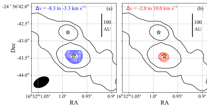
Fig. 8. Contour maps for \text{SO}_2 18_{4,14}-18_{3,15} for two ranges of velocities. The contours start at 4\sigma , following a step of 0.5\sigma . The black contours represent the continuum emission of Fig. 1 for a value of 4 and 15\sigma ( \sigma = 0.4\text{mJy beam}^{-1} ). The green and white stars indicate the position of Oph-IRS67A and B, respectively. The synthesised beam is represented by a black filled ellipse.
