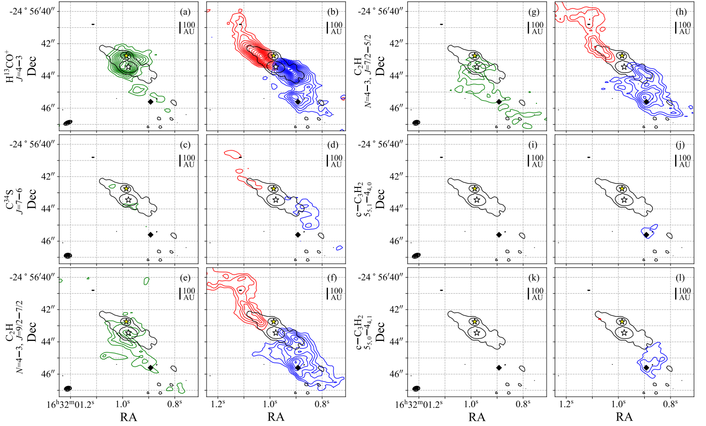
Fig. 7. Contour maps for \text{H}^{13}\text{CO}^+ , \text{C}^{34}\text{S} , both \text{C}_2\text{H} doublets and both c\text{-C}_3\text{H}_2 transitions, starting at 5\sigma and following a step of 4\sigma ( \sigma_{\text{H}^{13}\text{CO}^+} and \sigma_{\text{C}^{34}\text{S}} are 6 \text{ mJy beam}^{-1} \text{ km s}^{-1} , while \sigma_{\text{C}_2\text{H}} and \sigma_{c\text{-C}_3\text{H}_2} are 9 \text{ mJy beam}^{-1} \text{ km s}^{-1} ). Green contours represent low-velocity emission, from -1 to 1 \text{ km s}^{-1} . Blue and red contours indicate intermediate velocities, from -1 to -5 \text{ km s}^{-1} and from 1 to 5 \text{ km s}^{-1} , respectively. The black contours represent the continuum emission of Fig. 1 for a value of 4 and 15\sigma ( \sigma = 0.4 \text{ mJy beam}^{-1} ). The yellow and white stars indicate the position of Oph-IRS67A and B, respectively. The black diamond denotes the location of the high-density region. The synthesised beam for each species is represented by a black filled ellipse.
