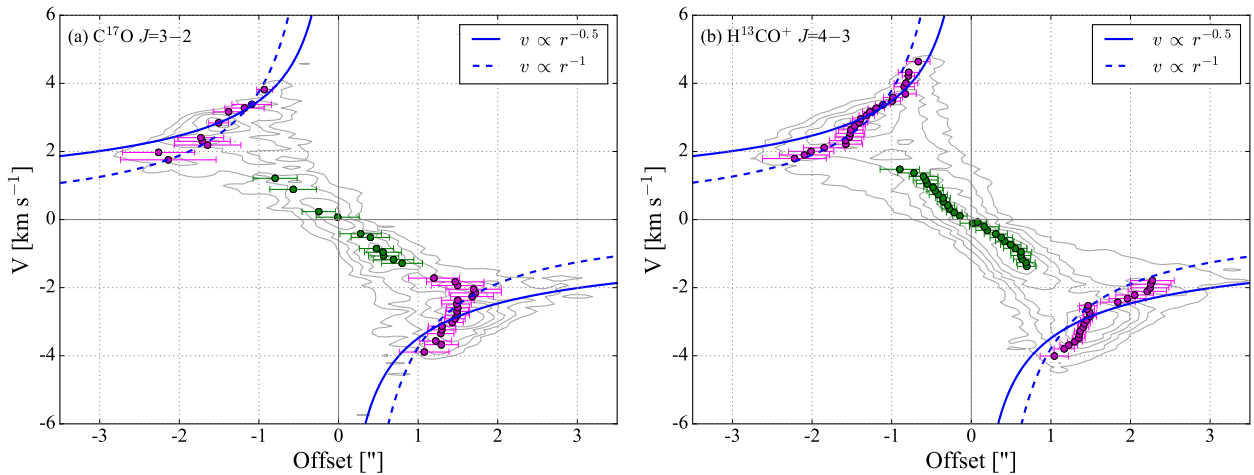
Fig. 9. Position-velocity diagrams for \text{C}^{17}\text{O} and \text{H}^{13}\text{CO}^+ towards the disk-like structure direction (PA = 234^\circ ) and centred at the position of the geometric centre. Green and magenta dots represent low- ( < 1.7 \text{ km s}^{-1} ) and high-velocity ( > 1.7 \text{ km s}^{-1} ) emission peaks, respectively. Blue solid and dashed lines show the best fit for a Keplerian and an infalling velocity profile, respectively. The cut taken from the image data is shown in grey contours, ranging from 3\sigma ( 1\sigma = 10 \text{ mJy beam}^{-1} ) to the maximum value of each transition. Each adjacent contour represents an increment of the 20% of the maximum value.
