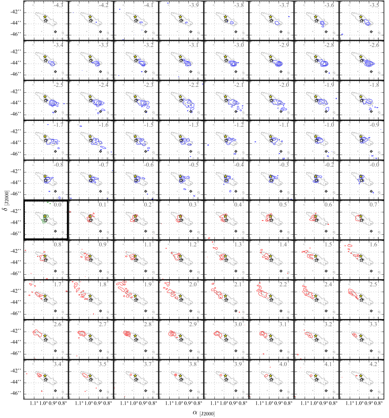
Fig. A.1. Velocity channel maps for \text{C}^{17}\text{O } J=3-2 (contours), superposed on the 0.87 mm continuum image (grey-scale; Fig. 1). The highlighted panel with green contours represents the systemic velocity of 4.2 \text{ km s}^{-1} . Blue and red contours indicate blue- and red-shifted emission with respect to the systemic velocity, respectively. In each panel, the contours start at 4\sigma ( \sigma = 10 \text{ mJy beam}^{-1} per channel), following a step of 3\sigma , and the mean velocity of each channel is also presented in units of \text{km s}^{-1} . The yellow and white stars show the positions of Oph-IRS67A and B, respectively. The grey diamond denotes the location of the high-density region.
