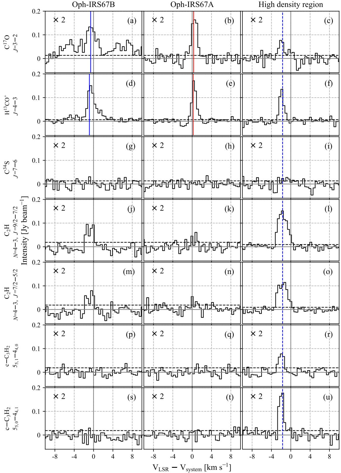
Fig. 4. Spectra of \text{C}^{17}\text{O} , \text{H}^{13}\text{CO}^+ , \text{C}^{34}\text{S} , both \text{C}_2\text{H} doublets and both c\text{-C}_3\text{H}_2 transitions for three different regions: the position of Oph-IRS67B (left column), the position of Oph-IRS67A (middle column) and the high-density region (right column). Spectra from panels (a) to (i) are rebinned spectrally by a factor of 4, while panels (j) to (u) are rebinned spectrally by a factor of 2, so that all spectra have the same spectral resolution ( 0.43 \text{ km s}^{-1} ). The dashed black horizontal line shows the value of 3\sigma ( \sigma = 3 \text{ mJy beam}^{-1} \text{ km s}^{-1} ). All spectra have been shifted to the systemic velocity ( 4.2 \text{ km s}^{-1} ; grey vertical line). The solid blue and red lines indicate the offset of the peak velocity determined from a Gaussian fit (see Table 4). The dashed blue line in the right column represents a velocity of -1.7 \text{ km s}^{-1} . Some spectra have been multiplied by a scaling factor as indicated in the top left corner.
