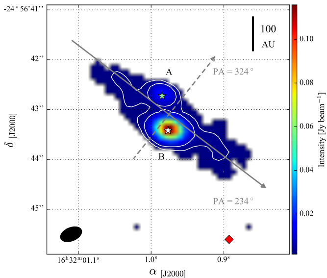
Fig. 1. Continuum emission above 4\sigma ( \sigma = 0.4 mJy beam -1 ) in colour scale and specific values of 7 and 15\sigma in white contours. The synthesised beam is represented by the black filled ellipse. The grey solid and dashed arrows cross at the geometric centre and they represent the direction of and perpendicular to the disk-like structure, respectively. The green and white stars show the positions of Oph-IRS67A and Oph-IRS67B, respectively. The red diamond denotes the location of the offset region.
