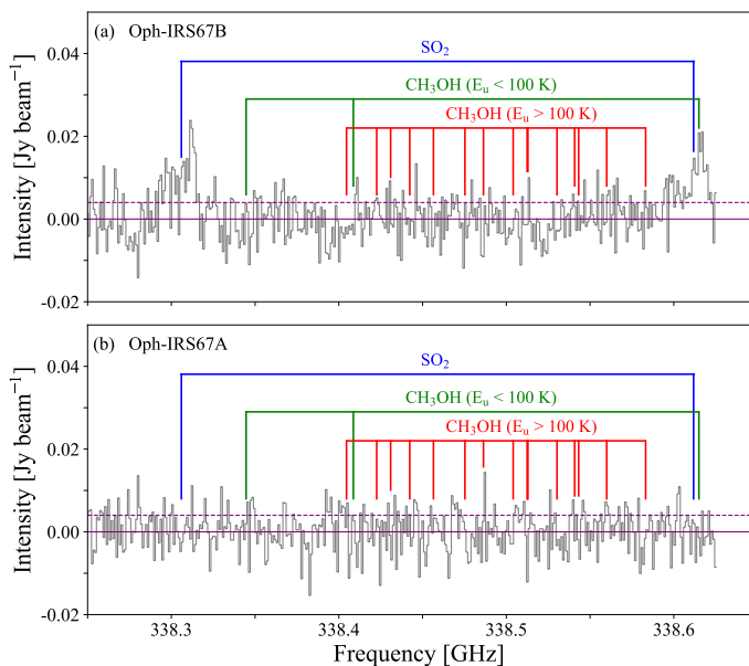
Fig. 5. Spectra from spectral window number 2, taken at the position of Oph-IRS67B ( top ) and Oph-IRS67A ( bottom ), and rebinned by a factor of 4. Blue lines show the rest frequency of SO 2 transitions. Green and red lines indicate the rest frequency of CH 3 OH transitions with upper energy levels ( E_u ) below and above 100 K, respectively. The purple dashed line shows the value of 1\sigma ( \sigma = 4 mJy beam -1 per channel).
