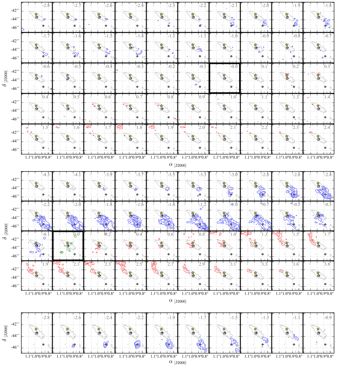
Fig. A.3. As in Fig. A.1 but for \text{C}^{34}\text{S } J=7-6 (upper frame), the doublet \text{C}_2\text{H } N=4-3, J=9/2-7/2 (central frame) and c\text{-C}_3\text{H}_2 5_{5,0}-4_{4,1} (lower frame).
