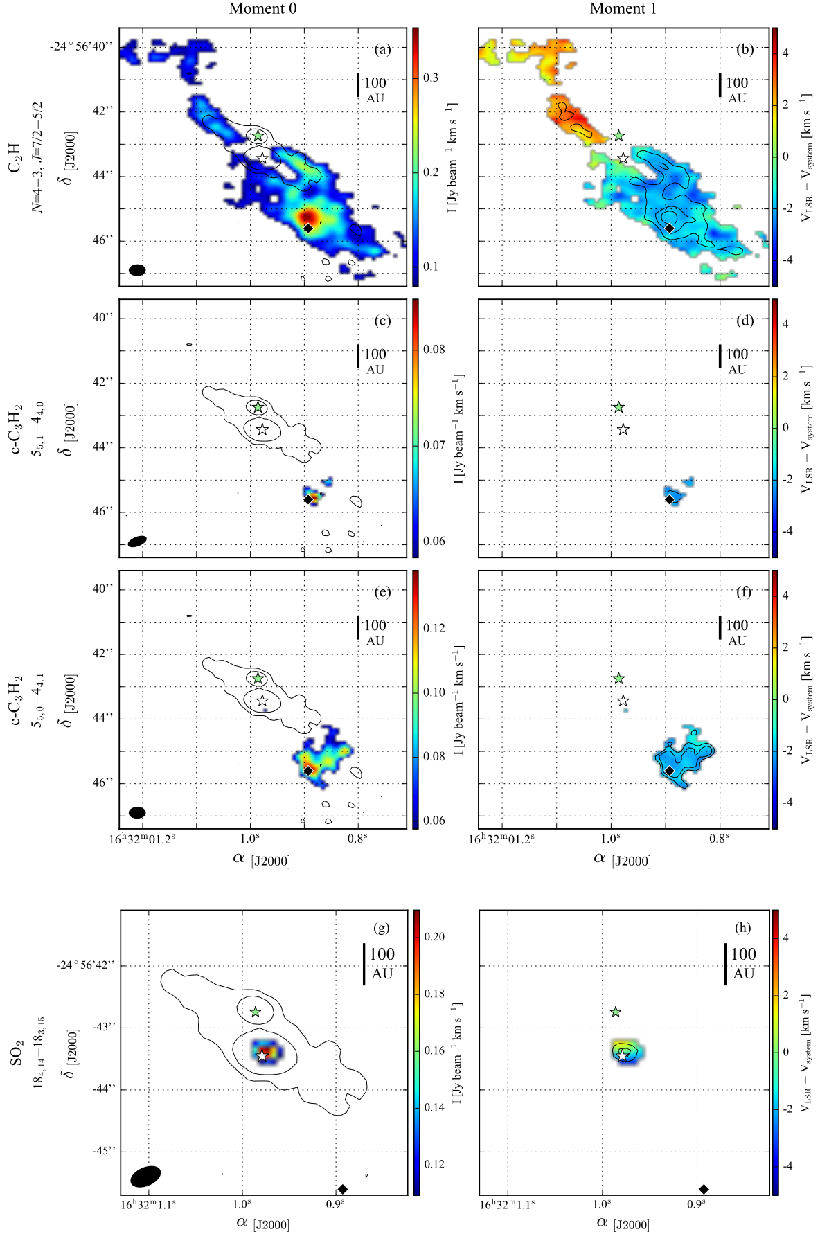
Fig. 3. As in Fig. 2 but for the C_2H N=4-3, J=7/2-5/2 doublet, both c-C_3H_2 transitions and SO_2 18_{4,14}-18_{3,15} ( \sigma_{c-C_3H_2} = 11 mJy beam ^{-1} km s ^{-1} and \sigma_{SO_2} = 25 mJy beam ^{-1} km s ^{-1} ). For SO_2 , the emission is above 4\sigma . Black contours in moment 1 maps represent 10, 15 and 20\sigma for C_2H , 6 and 8\sigma for c-C_3H_2 , and 5 and 7\sigma for SO_2 . Panels g and h represent a zoomed-in region.
