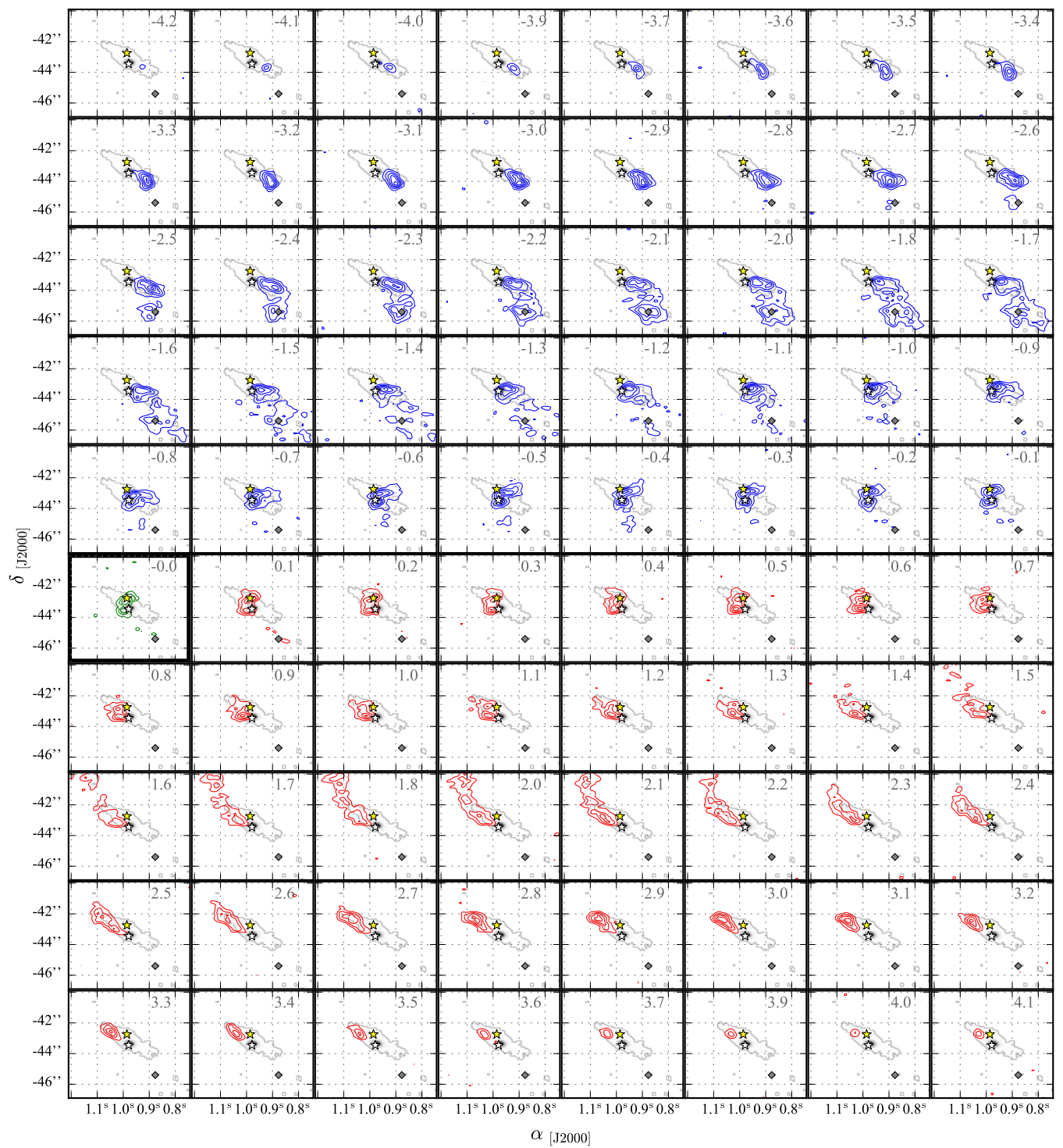
Fig. A.2. As in Fig. A.1 but for \text{H}^{13}\text{CO}^+ J=4-3 , where contours start at 4\sigma and follow a step of 4\sigma .
