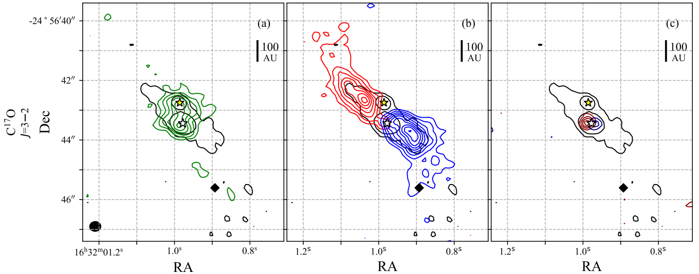
Fig. 6. Channel maps for C^{17}O , starting at 5\sigma ( \sigma = 6 \text{ mJy beam}^{-1} \text{ km s}^{-1} ) and following a step of 4\sigma . Green contours represent low velocities emission, from -1 to 1 \text{ km s}^{-1} (left). Blue and red contours indicate intermediate velocities, from -1 to -5 \text{ km s}^{-1} and from 1 to 5 \text{ km s}^{-1} , respectively (middle). Dark-red and dark-blue contours show high-velocity emission, from -5 to -10 \text{ km s}^{-1} and from 5 to 10 \text{ km s}^{-1} , respectively (right). The black contours represent the continuum emission of Fig. 1 for values of 4 and 15\sigma ( \sigma = 0.4 \text{ mJy beam}^{-1} ). The yellow and white stars indicate the position of Oph-IRS67A and B, respectively. The black diamond denotes the location of the high density region. The synthesised beam is represented by a black filled ellipse.
