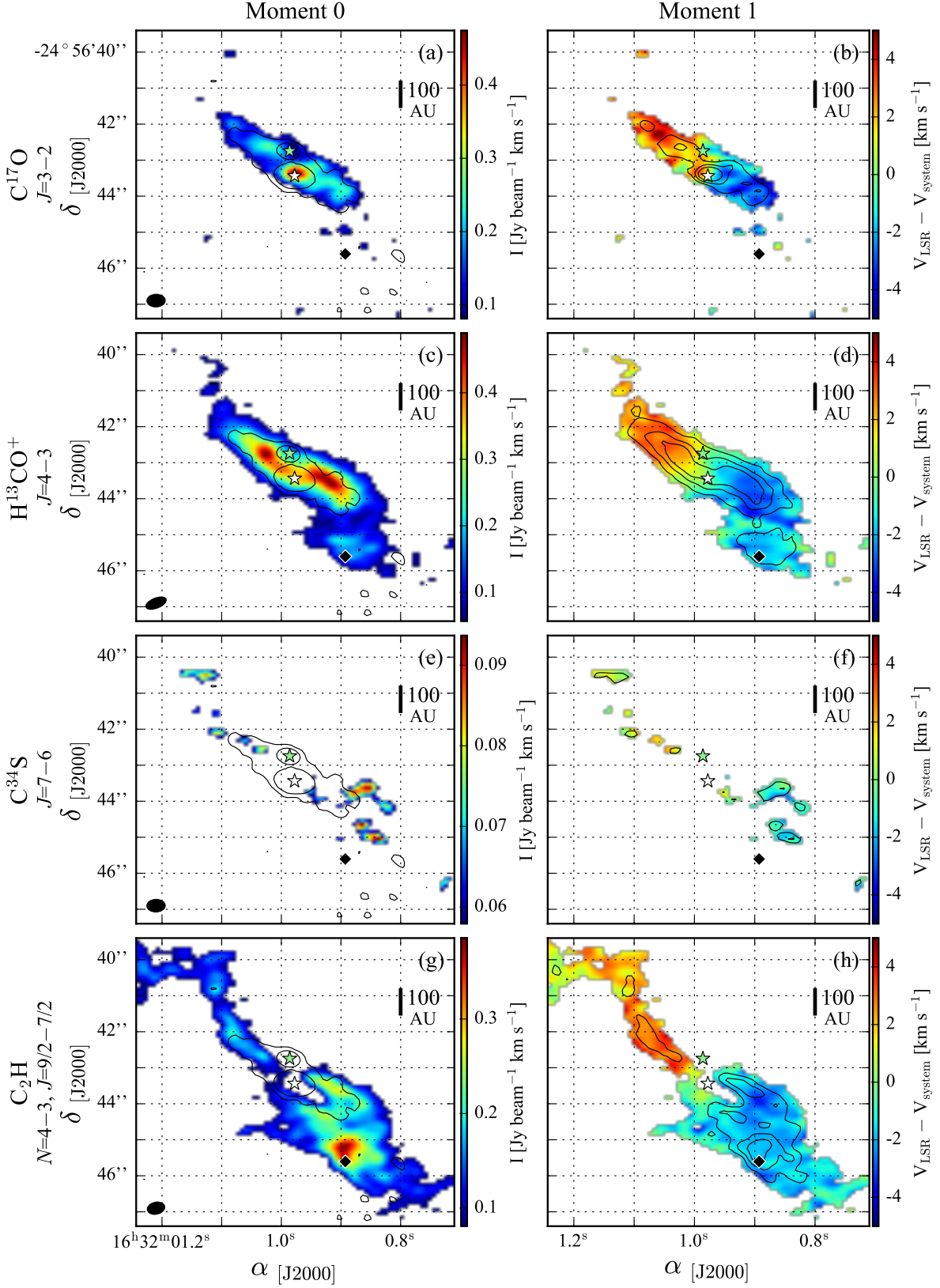
Fig. 2. Moments 0 (left column) and 1 (right column) for C^{17}O , H^{13}CO^+ , C^{34}S and the C_2H N=4-3 , J=9/2-7/2 doublet, above 5\sigma ( \sigma_{C^{17}O} = 15 \text{ mJy beam}^{-1} \text{ km s}^{-1} , \sigma_{H^{13}CO^+} = 10 \text{ mJy beam}^{-1} \text{ km s}^{-1} , \sigma_{C^{34}S} = 10 \text{ mJy beam}^{-1} \text{ km s}^{-1} and \sigma_{C_2H} = 15 \text{ mJy beam}^{-1} \text{ km s}^{-1} ). Each \sigma was calculated using the following formula: \sigma = rms \times \Delta N \times (N)^{0.5} , where \Delta N and N are the channel width and number of channels, respectively. Black contours in moment 0 maps represent the continuum emission from Fig. 1, for values of 4 and 15\sigma . Black contours in moment 1 maps show \sigma values of their respective moment 0 maps, being 10, 15 and 20\sigma for C^{17}O and C_2H , 10, 20 and 30\sigma for H^{13}CO^+ , and 6 and 8\sigma for C^{34}S . The green and white stars indicate the position of Oph-IRS67A and B, respectively. The black diamond denotes the location of the offset region. The synthesised beam for each species is represented by a black filled ellipse.
