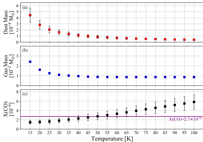
Fig. 11. Dust mass, gas mass, and values of CO abundances, for different temperatures and taken for the entire system (both sources and the circumbinary disk). The CO abundances are calculated by assuming a gas-to-dust ratio of 100. For gas masses (blue squares), the uncertainties are \sim 0.3\% of the value and are imperceptible on the plot. The purple horizontal line shows the value of 2.7 \times 10^{-4} for the abundance of CO with respect to \text{H}_2 .
