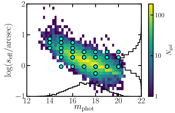
Figure 2. Magnitude and size distribution of satellites in the MENeACS spec+RS sample. The logarithmic color scale shows the number of galaxies per two-dimensional bin, while black histograms show the one-dimensional distributions. Cyan circles show the coordinates used in the grid image simulations used to determine the additive bias on the shape measurements in Section 4.2. Note that galaxies at the bottom-right corner of the distribution, not covered by the simulations, are faint and small and therefore can be safely assumed to produce no obscuration (see Appendix A).
