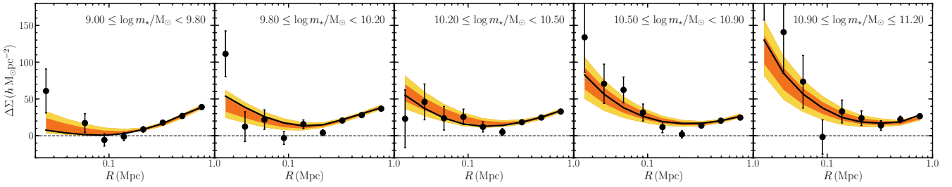
Figure 9. Excess surface mass density of the spec+RS sample, binned by stellar mass as shown in the legends (same as the magenta triangles in Figure 8). The black line shows the best-fitting model from the MCMC and the orange and yellow regions outline the 68 and 95 per cent credible intervals.
