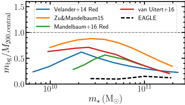
Figure 11. Ratio of subhalo masses measured in this work to central halo masses from different observational studies (solid lines) and measured in the EAGLE simulation by Velliscig et al. (2016) (black dashed line), at fixed stellar mass. The ratios for Velander et al. (2014) and Mandelbaum et al. (2016) are linearly interpolated from the data points. Note that statistical uncertainties dominate measurements at m_* \lesssim 2 \times 10^{10} M_\odot . See Figure 10 for a more detailed description of the different measurements.
