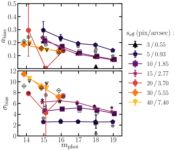
Figure A2. Amplitude and width of Gaussian fits to the additive bias c_t (solid symbols), and the results from an overall fit to each panel given in Equation A2 (empty symbols). Solid lines connect simulation sets with the same half-light radius as shown in the legend.
