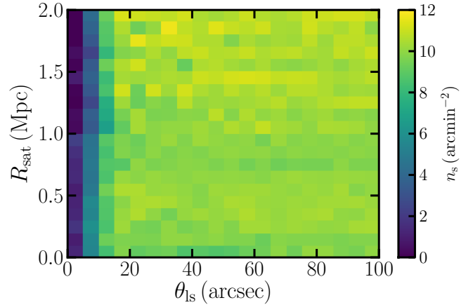
Figure 4. Observed number density of background sources as a function of lens-source separation, \theta_{ls} , and distance from the lens to the cluster centre, R_{\text{sat}} , for all MENeACS clusters, after applying all the cuts described in Section 3.
