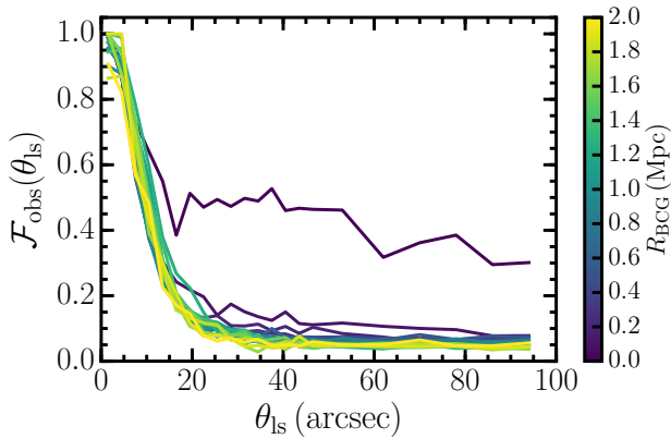
Figure 7. Obscuration profile measured in the image simulations as a function of lens-source separation, \theta_{ls} , in bins of cluster-centric distance, R_{BCG} , averaged over all MENeACS clusters.
