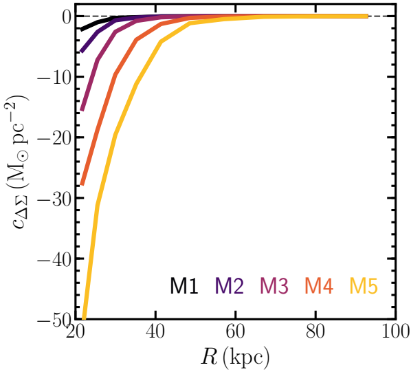
Figure 3. Average tangential additive bias, c_{\Delta\Sigma} \equiv \Sigma_c c_t , for the five stellar mass bins studied in Section 6, from low (M1) to high (M5) stellar mass (see Table 1). Note the smaller extent of the horizontal axis compared to other similar figures.
