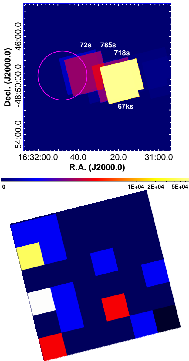
Fig. 1. (Top) SXS exposure map with the designation of the exposure time for each pointing position. The magenta circle corresponds to the source extraction region for the SXI (see figure 4 bottom panel). (Bottom) Spatial event distribution of the SXS microcalorimeter array in the DET coordinate in the energy band from 6.38 to 6.42 keV. Blue, red, yellow and white pixels correspond to detection of one, two, three and four events, respectively. The black pixel at the bottom right is the calibration pixel that is not directly exposed to the sky.
