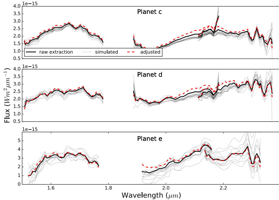
Figure 5. Resulting flux at 10pc of KLIP-FM spectrum extraction for each planet (solid black line) and recovery of artificial sources (gray lines), simulated with the matching spectrum. Increases in flux at the edges of the K1 band, where the filter throughput is low, are not significant. These are not seen in the case of e since these data were processed without the wavelength slices at the edge of the band. The red dotted line shows the adjusted spectrum applying the flux loss factor in Equation 6.
