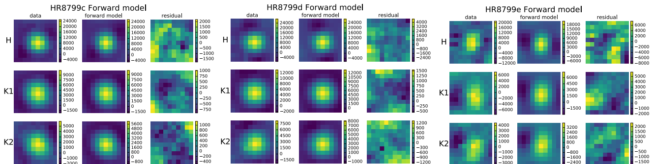
Figure 12. A summary of the forward model performance for HR 8799 c (left) d (middle) and e (right). Klipped data is shown to the left, the forward model is in the middle panel and the rightmost panel shows the difference between these two. Each image stamp is summed over the bandpass. Pixel values are in raw data units. Residual speckle noise appears to be influencing the K1 reduction of HR 8799 e.
