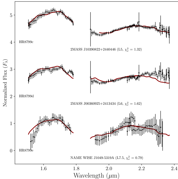
Figure 10. Best fit object to each of HR 8799 c, d, and e spectra within the described spectral library. Both the unrestricted and restricted case fits yielded the same best fitting object spectrum (Zhang et al. 2009; Chiu et al. 2006; Schneider et al. 2014; Luhman 2013).
