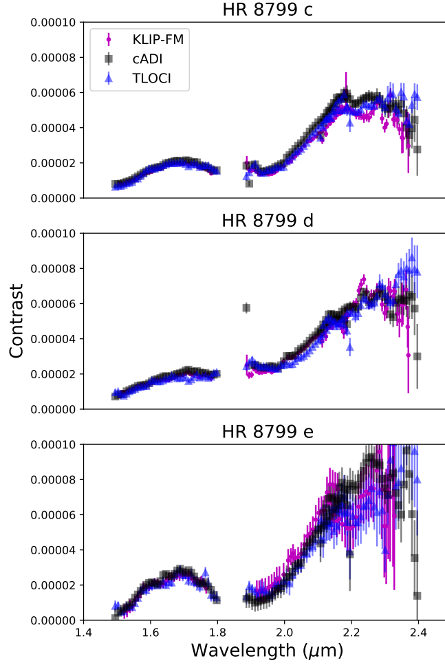
Figure 13. Comparison of the KLIP forward modeling algorithm reduction presented in this paper (magenta circles) with cADI (black squares) and TLOCI (blue triangles) reductions. The planet-to-star contrast is plotted vs. wavelength.
