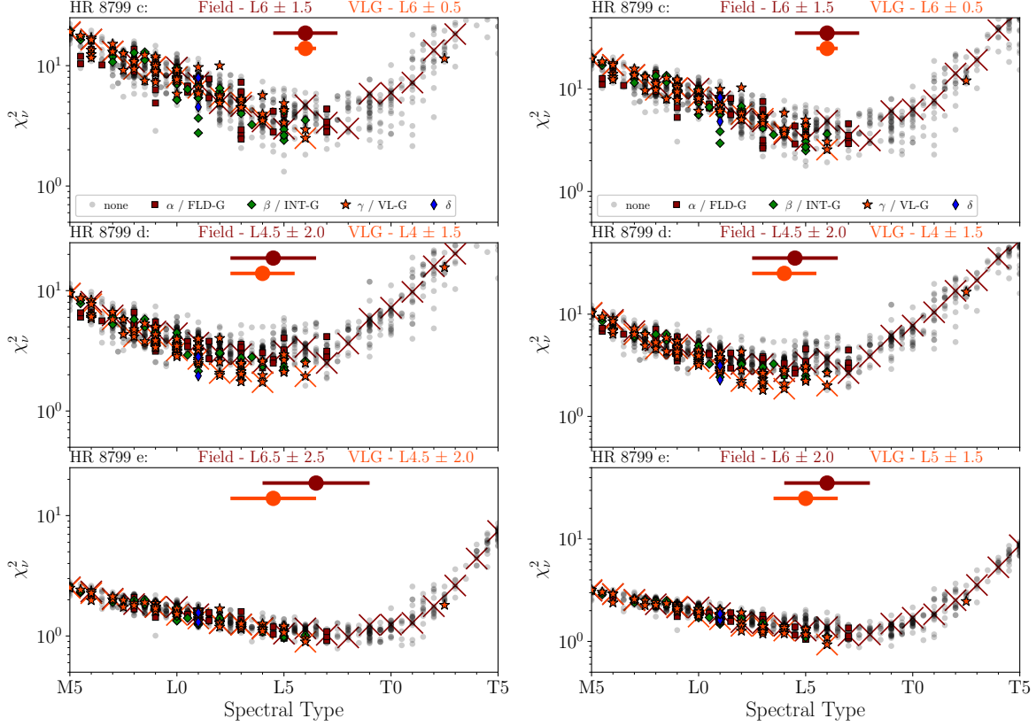
Figure 9. Left: Unrestricted \chi^2 fit of spectral library objects to the combined H & K GPI spectrum. The unrestricted fit allows the normalization to vary between H and K1+K2 bands. Right: Restricted \chi^2 fit of spectral library objects to the combined H & K GPI spectrum. The restricted fit only allows the normalization to vary within the uncertainty of photometric calibration. The two agree within error in all cases.
