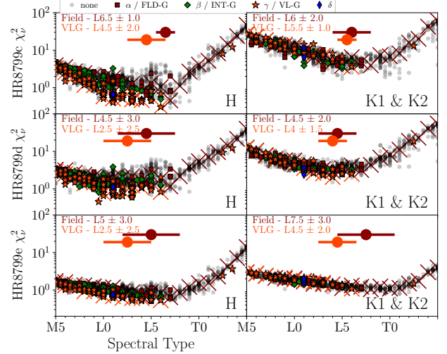
Figure 8. We plot \chi^2_{\nu} between our GPI spectrum and each object in the spectral libraries described, as a function of spectral type of field objects for each planet. From top to bottom we plot planets c, d, and e. The left shows \chi^2 for H band, the right shows the \chi^2 for combined K1, K2 bands. The large red and orange points at the top of each panel represent the mean and 1 - \sigma error for the best fit SED for field and VLG objects, respectively. We indicate gravity classification by the legend at the top. Spectral standards for FLD-G (Burgasser 2014; Kirkpatrick et al. 2010) and VL-G (Allers & Liu 2013) are indicated by red and yellow crosses, respectively.
