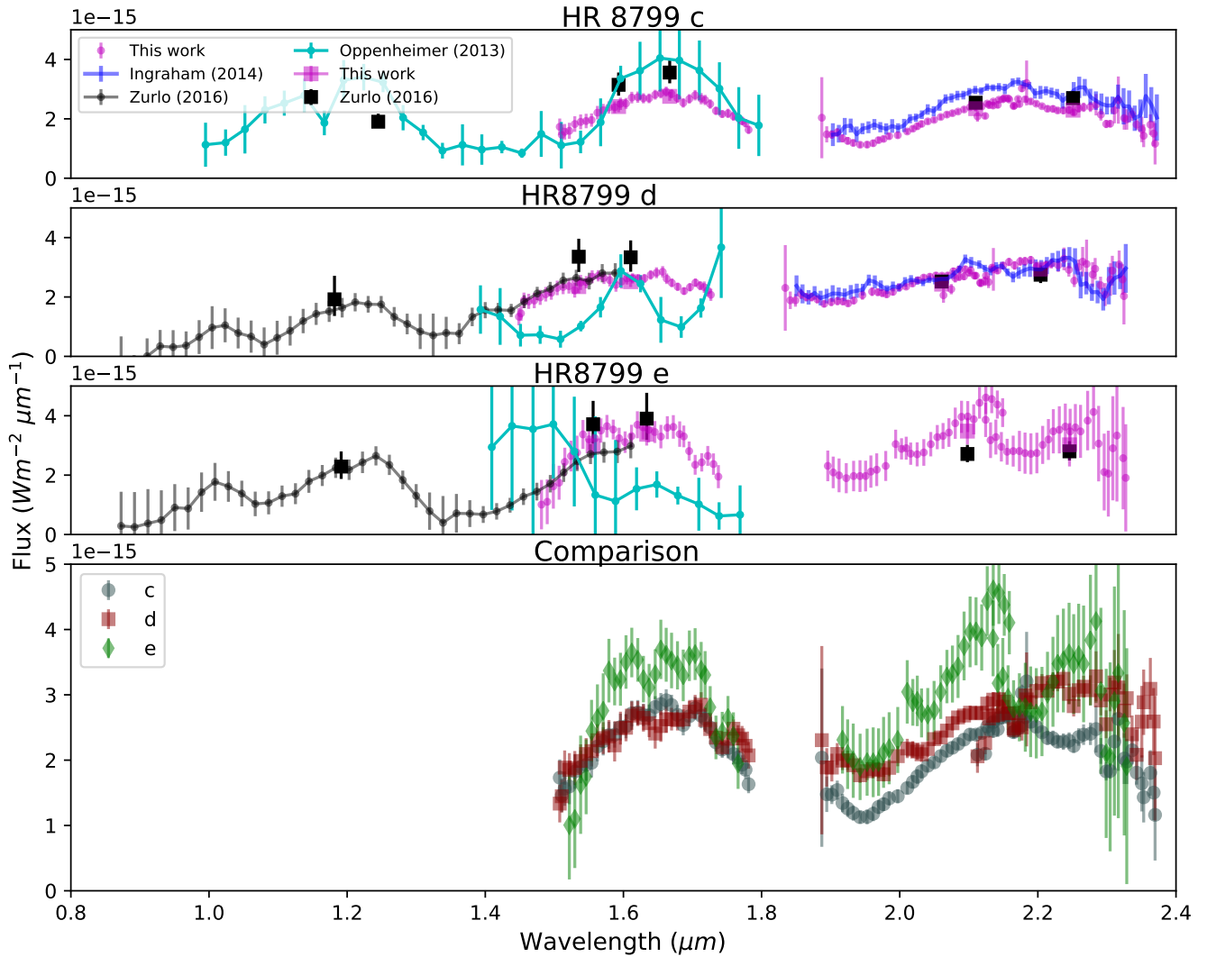
Figure 6. Spectra recovered with KLIP FM for HR 8799 c, d, and e showing flux at 10pc. Overplotted are the original GPI K-band spectra of c and d for the same dataset in dark blue (Ingraham et al. 2014), YJH spectra from Palomar/P1640 (Oppenheimer et al. 2013) (KLIP reduction) in cyan points, YJH spectra and JHK photometry using the VLT/SPHERE instrument (Zurlo et al. 2016) in black points and squares. The P1640 points are scaled from normalized flux units to match our data for this comparison. The bottom panel shows a comparison of our three recovered spectra.
