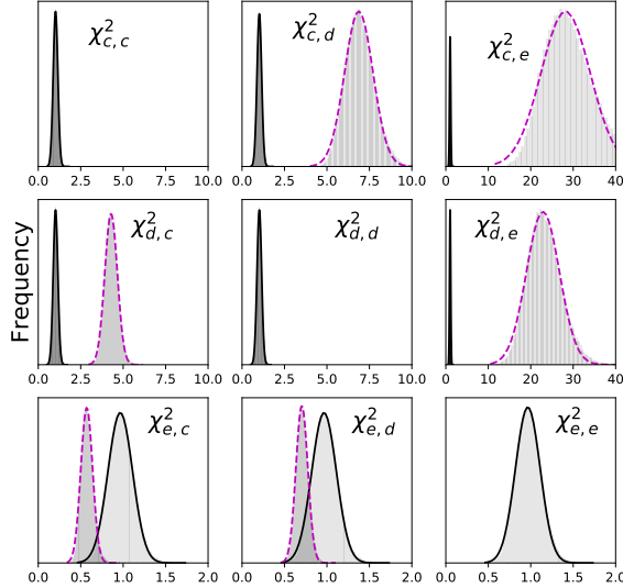
Figure 7. A cross-comparison of all three planets showing the distribution of \chi^2_{i,j} (defined in Equation 7). The diagonal shows each spectrum compared with 10^5 random draws from itself within the error bars. These, in solid outline are repeated for each panel in the same row. The off-diagonal panels also show the comparison with random draws from a different object spectrum, as indicated. These show clear ( > 5\sigma ) discrepancy between c and d planets.
