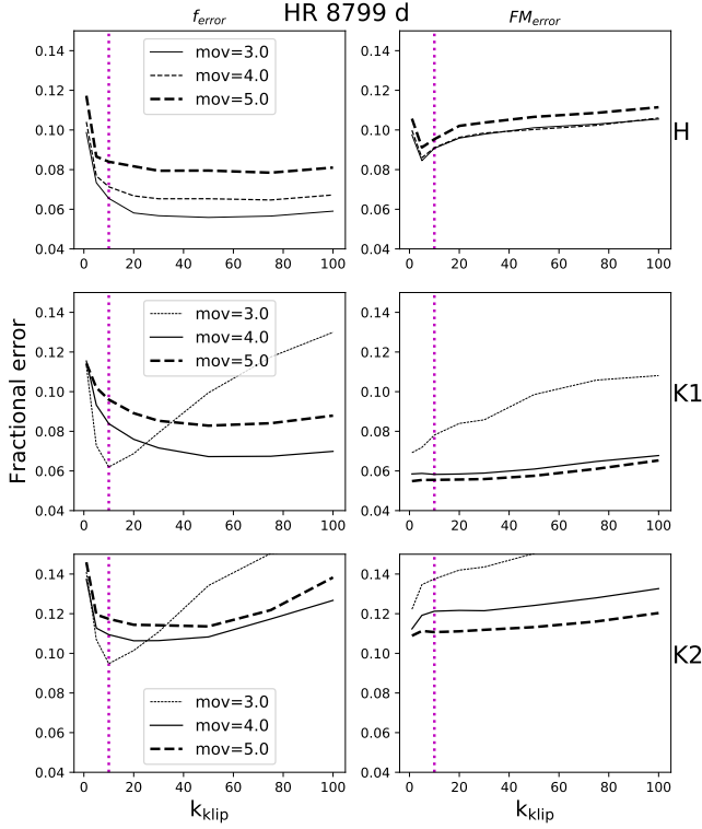
Figure 2. Same as Figure 1, but for HR 8799 d. The intersection of the solid curve and vertical dotted line denote our choice of parameters.
