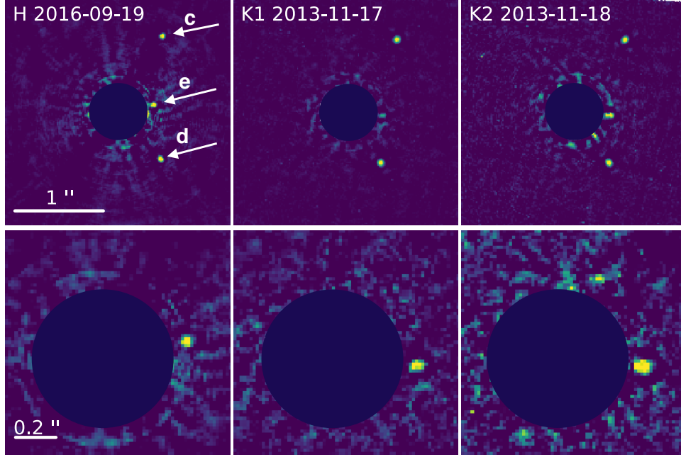
Figure 4. Top: Our standard KLIP subtracted cubes with mov = 3 pixels. Bottom: Subtracted cubes with mov = 1 pixel. The data are zoomed in to highlight HR 8799. The H band data quality is higher due to larger field rotation. We see the relative position difference of planet e due to orbital motion between the 2013 (K band) and 2016 (H band) epochs.
