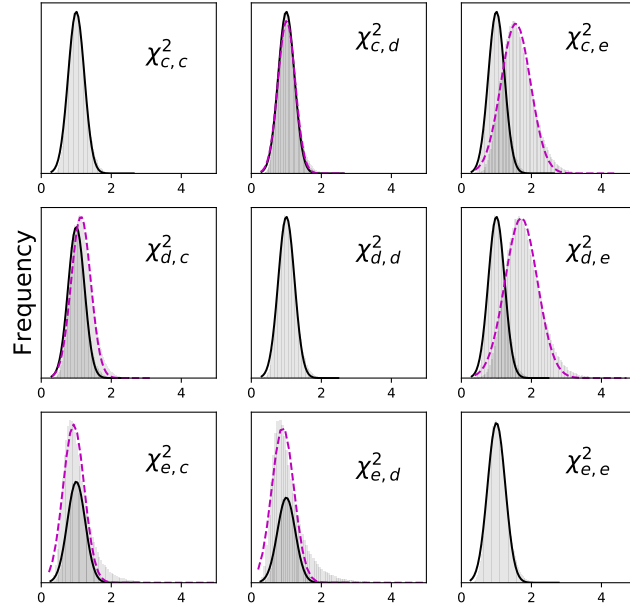
Figure 14. Comparison of \chi^2 distributions for H band.
