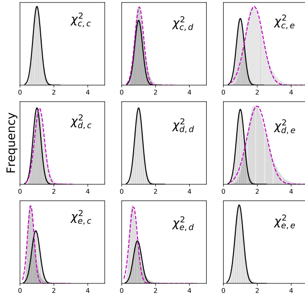
Figure 15. Comparison of \chi^2 distributions for K1 band.
