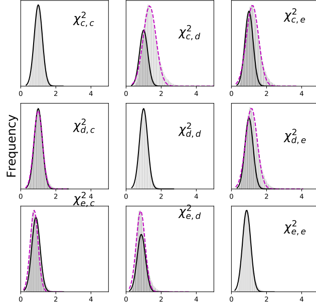
Figure 16. Comparison of \chi^2 distributions for K2 band.
