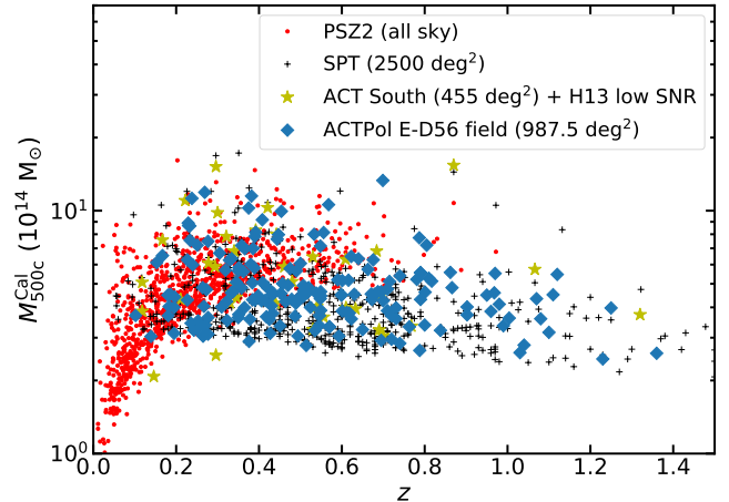
Figure 27. Comparison of the ACTPol E-D56 cluster sample in the (mass, redshift) plane with other blind SZ surveys: SPT (Bleem et al. 2015), and PSZ2 (Planck Collaboration et al. 2016a). Additional clusters from the southern ACT field (Marriage et al. 2011; 23 objects) and equatorial clusters that were masked/not detected in the E-D56 field with \text{SNR} > 4 (Table A4; 15 objects) are shown as yellow stars, using the masses and redshifts as listed in H13. Here, all the ACT SZ masses have been re-scaled according to a richness-based weak-lensing mass calibration (Section 6.1). The SPT and PSZ2 mass measurements are as reported in Bleem et al. (2015) and Planck Collaboration et al. (2016a) respectively (see Section 6.2).
