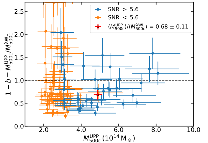
Figure 24. Comparison of richness-based weak-lensing masses ( M_{500c}^{AWL} ), derived from applying the Simet et al. (2017) scaling relation to ACTPol clusters in common with redMaPPer, with ACTPol UPP/A10 SZ masses. The red square marks the ratio \langle M_{500c}^{UPP} \rangle / \langle M_{500c}^{AWL} \rangle = 0.68 \pm 0.11 for the SNR > 5.6 subsample, which is complete at z < 0.6 . The effect of a Malmquist-type bias in the SZ selection can be seen on the clusters with SNR < 5.6 , many of which have SNR close to the detection threshold.
