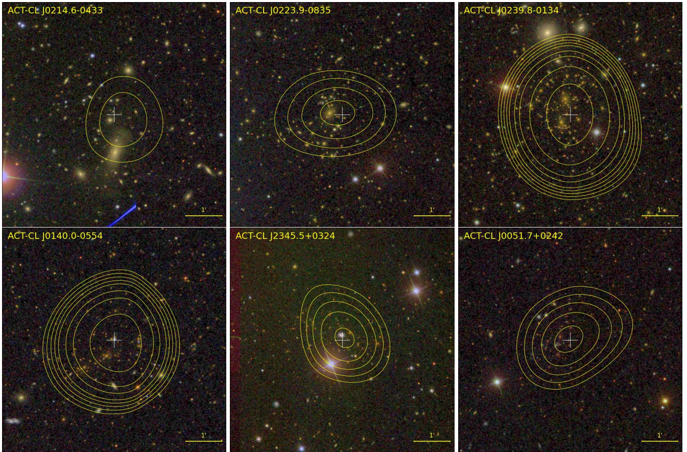
Figure 13. Example optical gri images of clusters confirmed in SDSS (these objects correspond to those shown in Fig. 12). Each image is 6' on a side, with North at the top and East at the left. The yellow contours (minimum 3\sigma , increasing in steps of 0.5\sigma up to \text{SNR} = 5 , and then by 1-2\sigma thereafter) indicate the (smoothed) 148 GHz decrement in the matched-filtered ACT map. The white cross indicates the ACT SZ cluster position. Note that ACT-CL J0051.7+0242 is a newly discovered cluster.
