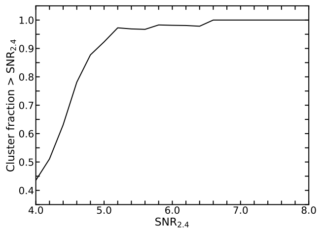
Figure 19. The cumulative fraction of candidates that are confirmed clusters as a function of \text{SNR}_{2.4} . For \text{SNR}_{2.4} > 5 , the fraction is less than 1 because of incomplete redshift follow-up; there is evidence from e.g., WISE imaging that these candidates are likely to be high-redshift ( z > 1 ) clusters. At \text{SNR}_{2.4} < 5 , the dominant effect is sample impurity (see Fig. 5).
