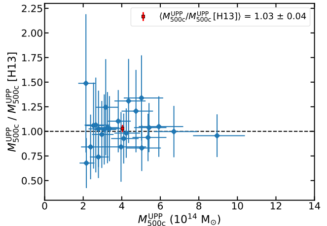
Figure 8. End-to-end test of M_{500c} recovery, comparing clusters cross-matched with H13 ( 2.5' matching radius) with M_{500c} values inferred from SZ decrement measurements made on D56 maps containing only ACTPol data, filtered at the \theta_{500c} = 2.4' scale (this work). The data sets used for this test have independent detector noise. The red square marks the unweighted mean ratio ( \pm standard error) between the two sets of measurements. This test assumes that clusters are described by both the UPP and the A10 mass-scaling relation.
