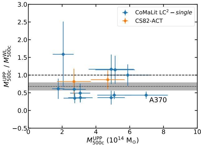
Figure 23. Comparison of weak-lensing masses from the CoMaLit database (Sereno 2015, blue) and the stacked weak-lensing analysis of Battaglia et al. (CS82-ACT; 2016, orange) with ACTPol SZ masses based on the UPP and A10 mass-scaling relation. The CS82-ACT masses plotted here are from NFW profile fits to the stacked weak-lensing signal. Here we used the LC^2 - single catalog from CoMaLit, which consists of objects modeled using a single halo. The dotted line and shaded area indicates the richness-based weak-lensing mass calibration factor and its uncertainty ( 0.68 \pm 0.11 ), obtained independently from these data by applying the Simet et al. (2017) scaling relation to ACTPol clusters cross matched with the redMaPPer catalog (see Section 6.1).
