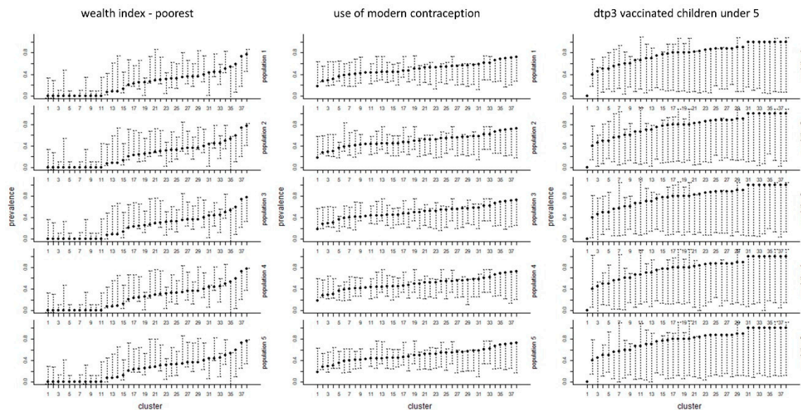
Figure 5. 2013 Namibia DHS PSU-level estimates (black dot) of average household wealth level, contraceptive use, and DTP3 vaccination versus the distribution of estimates from 100 samples (bar) selected in EAs located within 5 m of the DHS PSUs for five synthetic population realizations.
