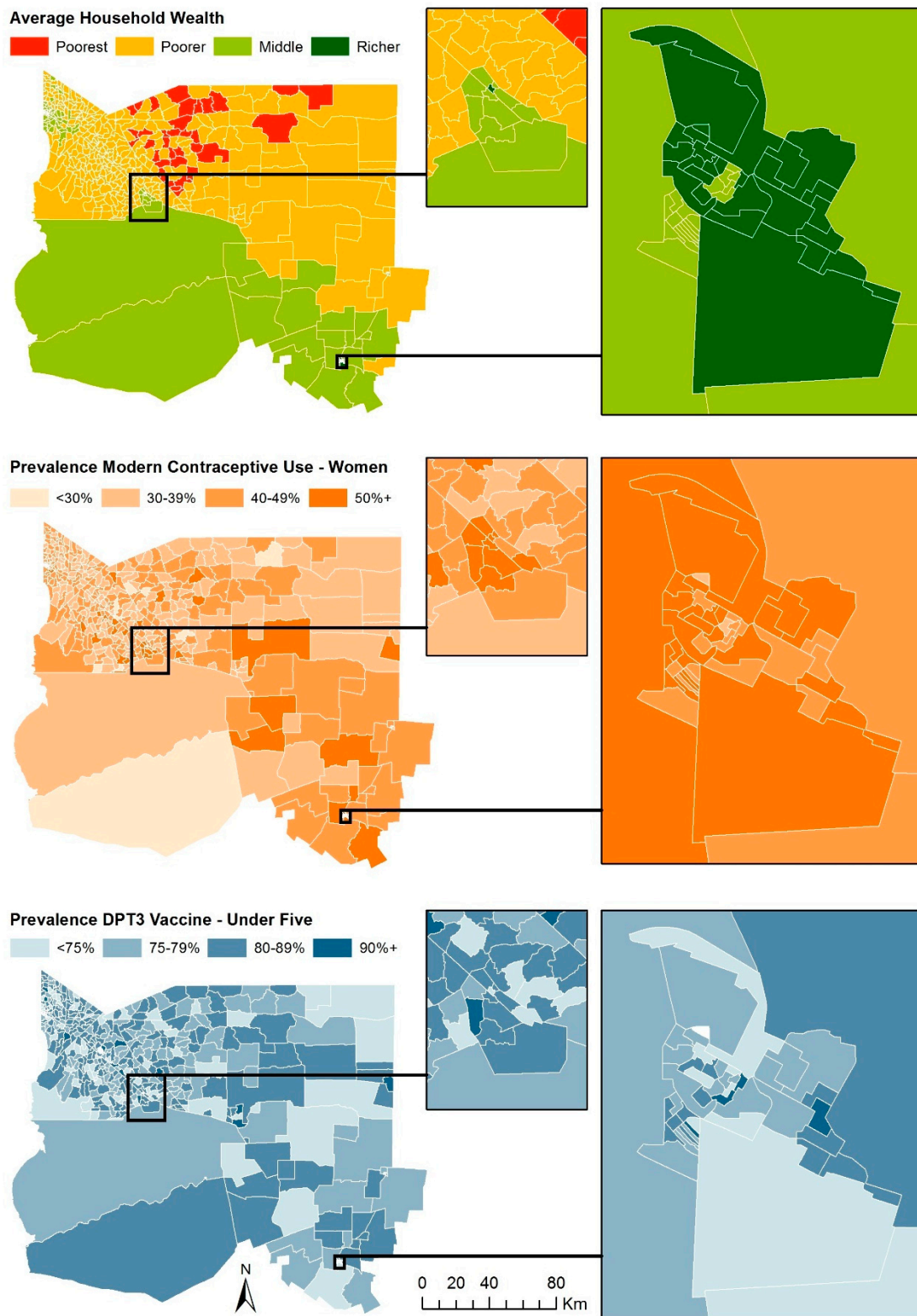
Figure 4. Maps of average household wealth level, conceptive use, and DPT3 vaccination by EA in one simulated population (synth_pop_1) in Oshikoto, Namibia.
