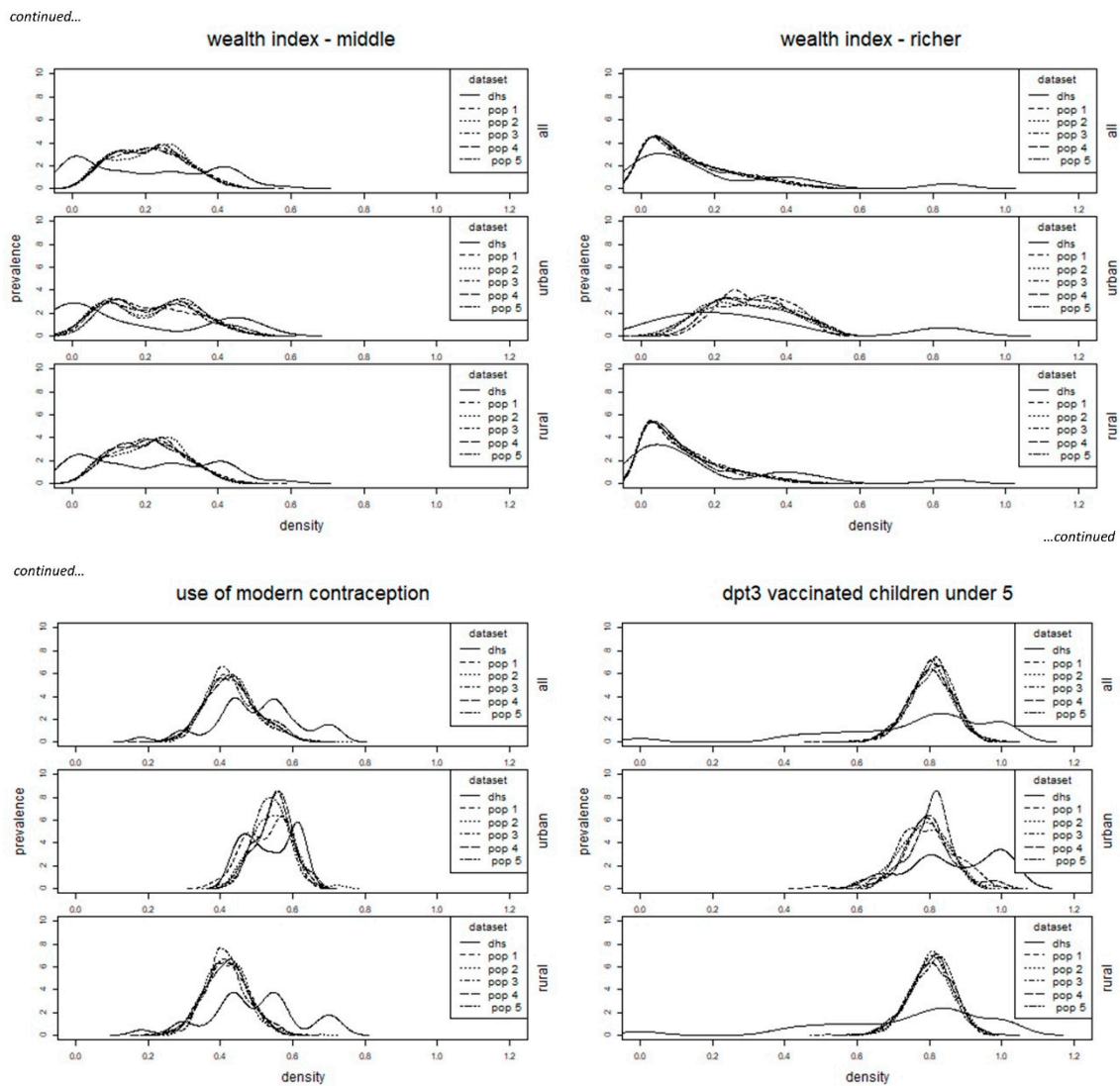
Figure 3. Comparison of prevalence ( y -axis) distributions ( x -axis) in the 2013 Namibia DHS for Oshikoto region (solid line) and five synthetic population realizations (dotted lines) across wealth categories, contraceptive use, and DTP3 vaccination.
