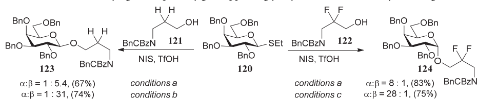
Scheme 2. Linkers of varying nucleophilicity gave opposite glycosylation stereoselectivity. (Seeberger, 2016).
