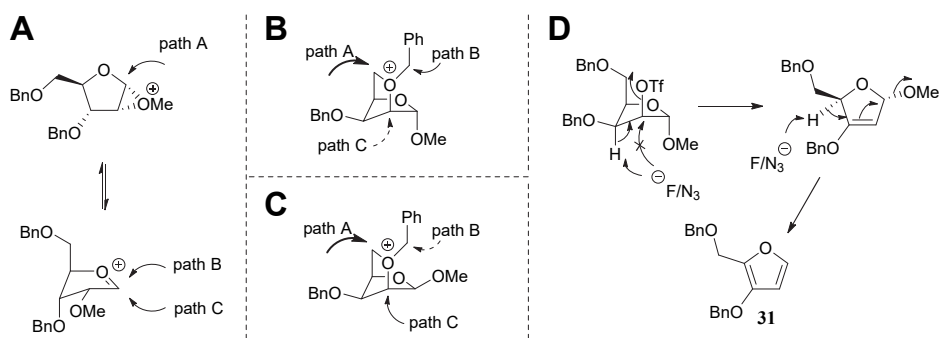
Figure 2. Mechanistic pathways underlying the formation of side products 26-31 .
