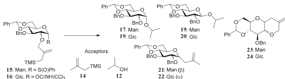
Figure 3. Cation-clock substitution products from external and internal nucleophiles.
