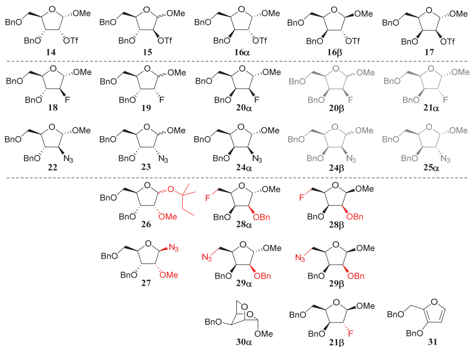
Figure 1. Furanosyl C-2-O-triflates (14-17) and their substitution products by fluoride inversion (18-21), and azide inversion (22-25). Major side products isolated from the reaction mixture (26-31), red color indicates the deviations from the expected products. Formation of the structures in grey was not observed.
