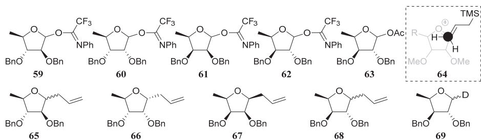
Figure 6. Imidate donors 59-62 , acetyl donor 63 and glycosylation products 65-69 of 5-deoxy furanosides. Inset: top view of the protruding C-H bonds on the acceptor.
