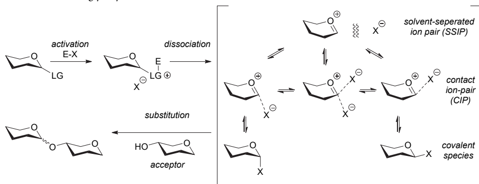
Scheme 2. General glycosylation mechanism. a
