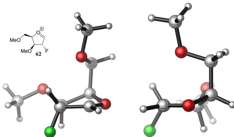
Figure 6. Ball-stick model of the {}^4E conformation of 2-fluoroxysyl oxocarbenium ion 62 , viewed through the C-2–C-3 bond and C-1–C-2 bond respectively.
