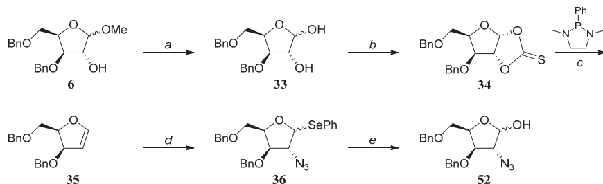
Scheme 3. Synthetic route towards 2-azidoxylose 52 via azidophenylselenation of glycal 35 .
