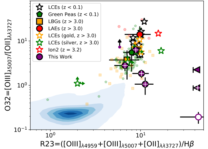
Figure 6. R23 vs O32 for our sample in comparison with various samples of high and low redshift star-forming galaxies. For most comparison samples, small symbols indicate individual galaxies and corresponding large, opaque symbols show averages for each sample. The exception is LyC emitting galaxies shown as white stars. Those with black edges are low- z galaxies from Izotov et al. (2016), Izotov et al. (2018a), and Izotov et al. (2018b), the red edged white star is the high- z galaxy Ion2 (de Barros et al. 2016; Vanzella et al. 2016), and orange and green edged white stars are z > 3.0 galaxies from the ‘‘gold subsample’’ and ‘‘silver subsample’’, respectively, of the LACES survey (Fletcher et al. 2018). Star-forming SDSS galaxies from (Zahid et al. 2013) are shown by the blue density contours. Galaxies in our MOSFIRE sample with detections of [OII] ( \lambda\lambda 3727 \text{ \AA} ), [OIII] ( \lambda 4959 \text{ \AA} ), [OIII] ( \lambda 5007 \text{ \AA} ), and H\beta are shown with large purple circles. Circles with white crosses indicate confirmed Ly\alpha emitters. Filled triangles represent those galaxies without H\beta observations indicating only O32 values and not R23 upper-limits. The small purple circle indicates the upper limit on O32 for galaxy 13459 (not detected in [OII] \lambda\lambda 3727 \text{ \AA} ). The open purple circle represents galaxy 17251, which shows evidence of being an ongoing merger (see Figure 2 and Section 5.1.1). Shocks associated with mergers may explain both the high R23 and low O32 values observed in this galaxy.
