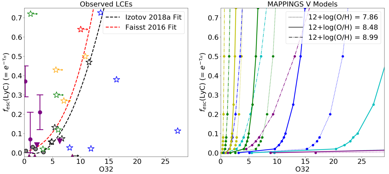
Figure 10. A comparison of the empirical relations between O32 and f_{esc}(LyC) suggested by Izotov et al. (2018b) and Faisst (2016) (left) with the theoretical predictions calculated using MAPPINGS V (right). On the left, LCEs at z \approx 0.05 from Izotov et al. (2016) and Izotov et al. (2018b) are shown as black, open stars as in Figures 6 and LCEs from Izotov et al. (2018a) are shown with blue, open stars. Lower redshift LCEs are indicated with grey circles. The open red star indicates the high redshift LCE, Ion2 (de Barros et al. 2016) and orange and green open stars show “gold” and “silver” subsamples of LCEs from the LACES survey (Fletcher et al. 2018). Observations for our sample are shown with purple symbols. Circles with error bars show galaxies with nonzero f_{esc}(LyC) from CLAUDS u -band photometry, downward triangles show upper limits on f_{esc}(LyC) based on CLAUDS u -band uncertainty, and small, upwards triangles show galaxies with f_{esc}(LyC) = 0.0 even when uncertainty in u is considered. The empirical fits presented in Izotov et al. (2018b) and Faisst (2016) and shown by black and red dashed lines, respectively. The fit of Faisst (2016) includes Ion2 and all black LCEs except for the one at the highest O32 and the fit of Izotov et al. (2018b) excludes Ion2 and includes all black, open stars. Blue open stars were reported more recently than either fit, and thus were not included. On the right, coloured lines show the outputs of the MAPPINGS V code at fixed Z with colours indicating different q_{ion} , identical to Figure 8. Different line styles for MAPPINGS V results correspond to different 12 + \log_{10}(O/H) as indicated in the legend.
