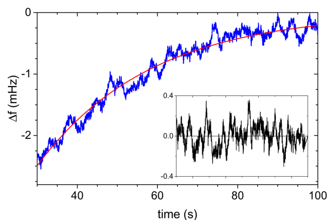
FIG. 7. Relaxation curve (1 Hz low-pass filter, 410 averages) measured at h = 1.0 \mu\text{m} and T = 21 \text{ mK} , for a pulse at frequency 882 kHz with B_{\text{RF}} = 172 \mu\text{T} and t_p = 80 \mu\text{s} . The solid red line is a fit to Eq. (2), from which we extract \Delta f_0 = -5.4 \text{ mHz} . The inset shows the difference between the data and the exponential fit, indicating a standard deviation of the measured frequency shift of 0.1 mHz.
