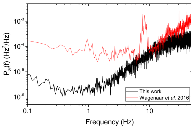
FIG. 2. Frequency noise spectrum P_{df} measured at a height of 1.3 \mu\text{m} . In red, we see the frequency noise spectrum from the initial experiment in our group, measured with a cantilever amplitude of 110 nm rms . 12 In black, we see the current experiment, measured with a cantilever amplitude of 43 nm rms . The reduction of the noise at higher frequencies in the black spectrum is due to the bandwidth of the PLL, which was set at 40 Hz.
