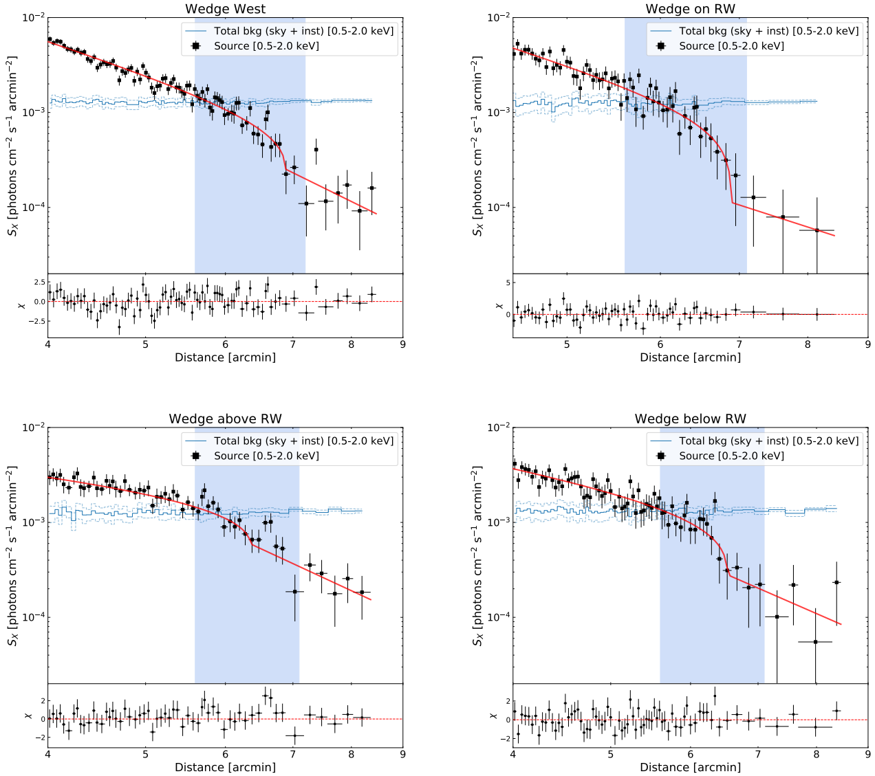
Figure 5. Surface brightness profiles across the western sector (top left panel) and the sub-sectors on, above and below RW (top right, bottom left and bottom right panels, respectively). The light blue rectangle identifies the position of the western radio relic. The total background level (i.e. instrumental and astrophysical) is shown by the light blue line, with the \pm 1\sigma uncertainties (light blue dashed lines). On the bottom of each panel, the residuals (i.e. \frac{S_{X,\text{obs}} - S_{X,\text{mod}}}{\Delta S_{X,\text{obs}}} ) are displayed.
