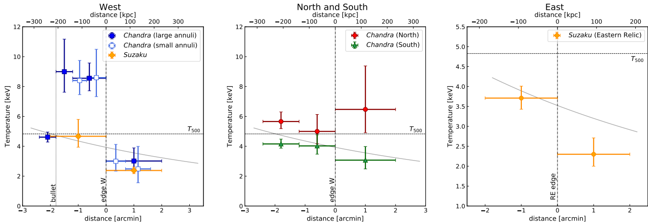
Figure 8. Radial temperature profiles westward (left), northward and southward (central) and on the eastern relic (right). All the values have been obtained by fixing the abundance and hydrogen column density at A = 0.3 Z_{\odot} and N_{\text{H}} = 0.311 \times 10^{22} \text{ cm}^2 , respectively. The horizontal dashed lines in the three panels represent the averaged temperature of the global cluster at R_{500} , obtained with Chandra . The vertical dot-dashed lines display the position of the western edge (left and central panel) and the edge of the eastern relic (right panel); the vertical dotted line in the left panel displays the position of the cold front. The solid gray line represents the averaged temperature profile according to Burns et al. (2010).
