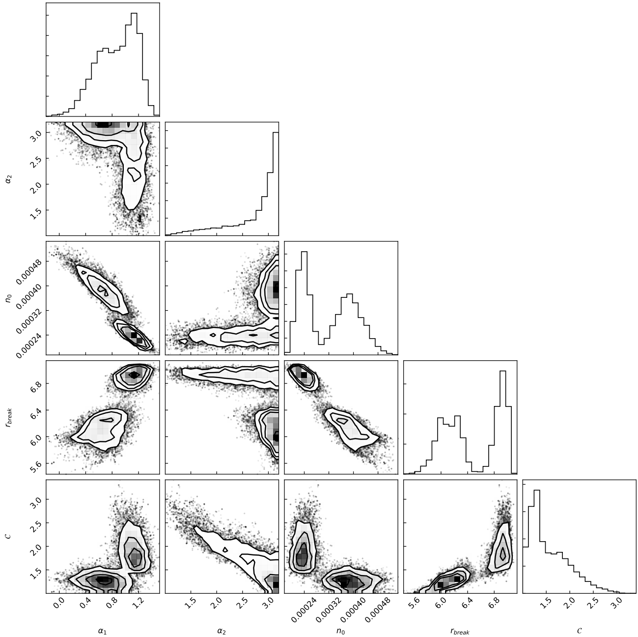
Figure A.4. The MCMC “corner plot” for the X-ray surface brightness profile across the wedge above the western relic (see bottom left panel in Fig. 5)
