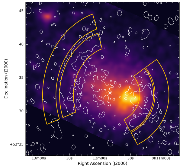
Figure 4. Suzaku 0.5–4.0 keV image of ZwCl0008. WSRT radio contours are drawn in white at the 3\sigma_{\text{rms}} level. Orange sectors overlaid represent the regions where the temperature measurements were extracted for the western and eastern relic (see left and right panel in Fig. 8, respectively). As for Fig. 3, the white cross represents the cluster center.
