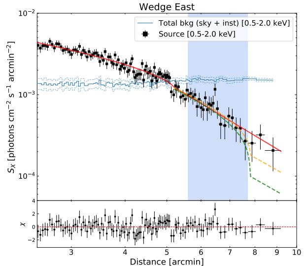
Figure 6. Surface brightness profile across the eastern sector. The light blue rectangle identifies the position of the eastern radio relic. The total background level (i.e. instrumental and astrophysical) is shown by the light blue line, with the \pm 1\sigma uncertainties (light blue dashed lines). On the bottom, the residuals (i.e. \frac{S_{X,\text{obs}} - S_{X,\text{mod}}}{\Delta S_{X,\text{obs}}} ) are displayed, representative of the broken power-law best-fit (red line). Models of density jumps of \mathcal{C} = 1.7 and \mathcal{C} = 2.3 at fixed r_{\text{break}} = 7.8 arcmin are also overlaid (dashed orange and green lined, respectively).
