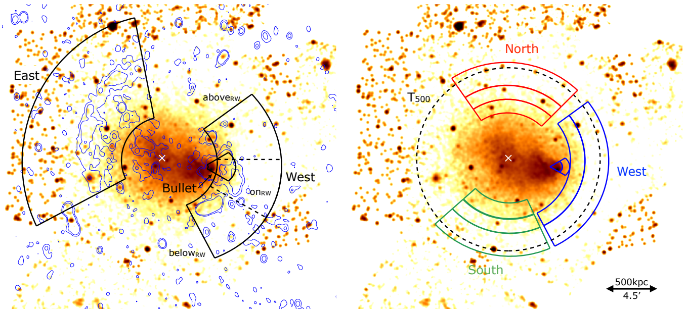
Figure 3. Smoothed ( 4'' ) Chandra 0.5–2.0 keV images showing the sectors used for extracting the surface brightness (left panel) and temperature (right panel) profiles shown in Figs. 5, 6, 7 and 8. The dashed lines in the left panel show the division for the western edge (sub-sectors above, on, and below the western relic). Radio contours in the same panel are drawn at [1, 4] \times 3\sigma_{\text{rms}} levels ( \sigma_{\text{rms}} is the same as that used in the bottom right panel in Fig. 1). The black dashed circle in the right panel represents the R_{500} region, from which the cluster average temperature has been obtained. The white cross represents the cluster center.
