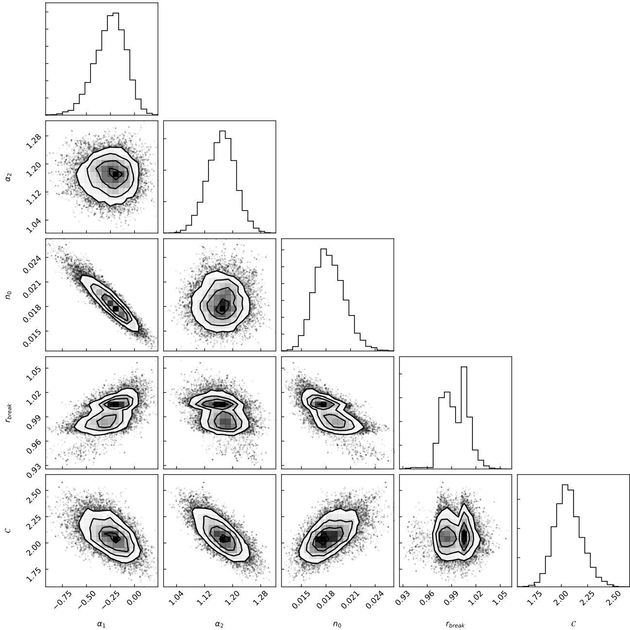
Figure A.3. The MCMC “corner plot” for the X-ray surface brightness profile across the bullet (see Fig. 7)
