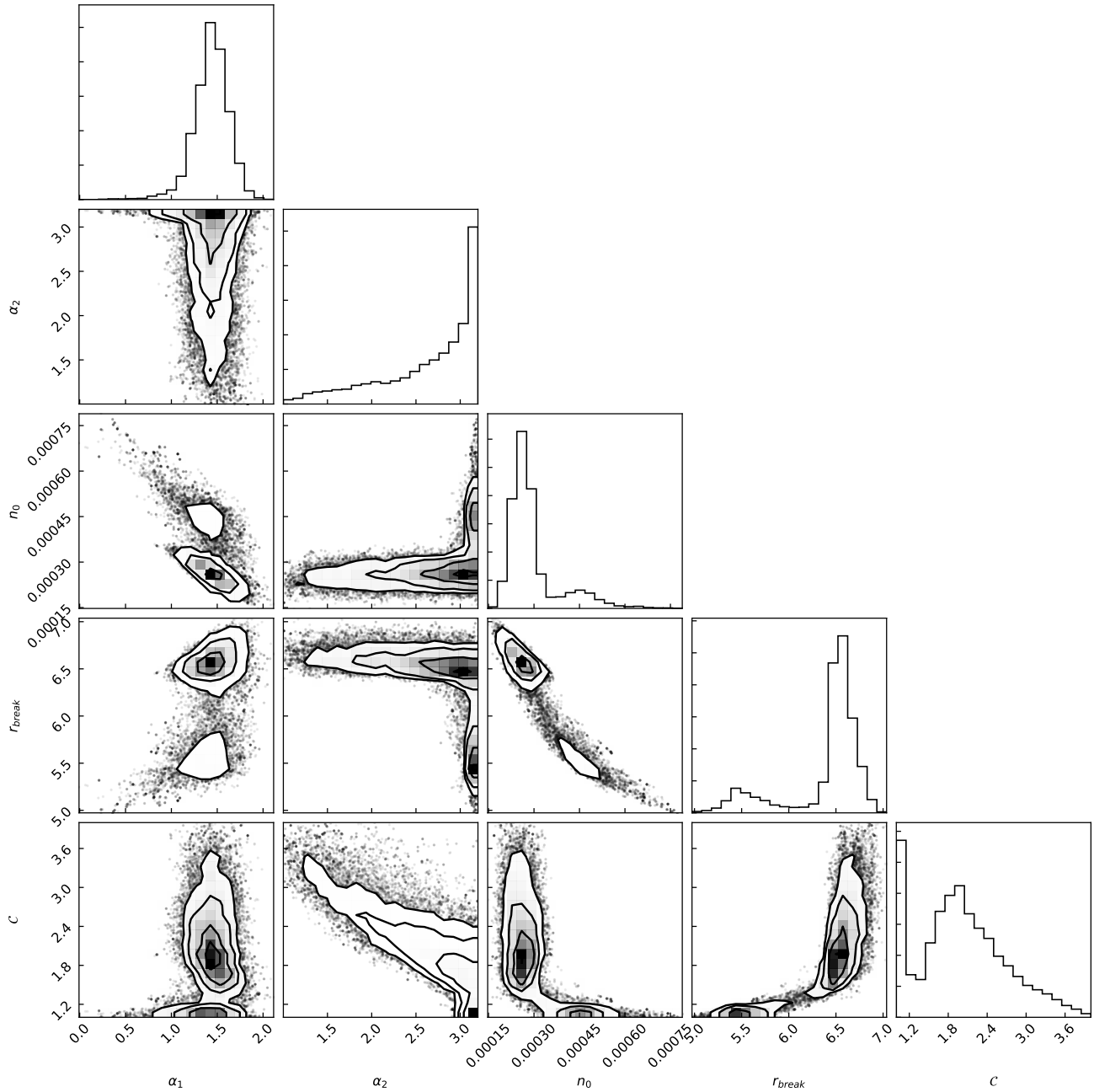
Figure A.6. The MCMC “corner plot” for the X-ray surface brightness profile across the wedge below the western relic (see bottom right panel in Fig. 5)
