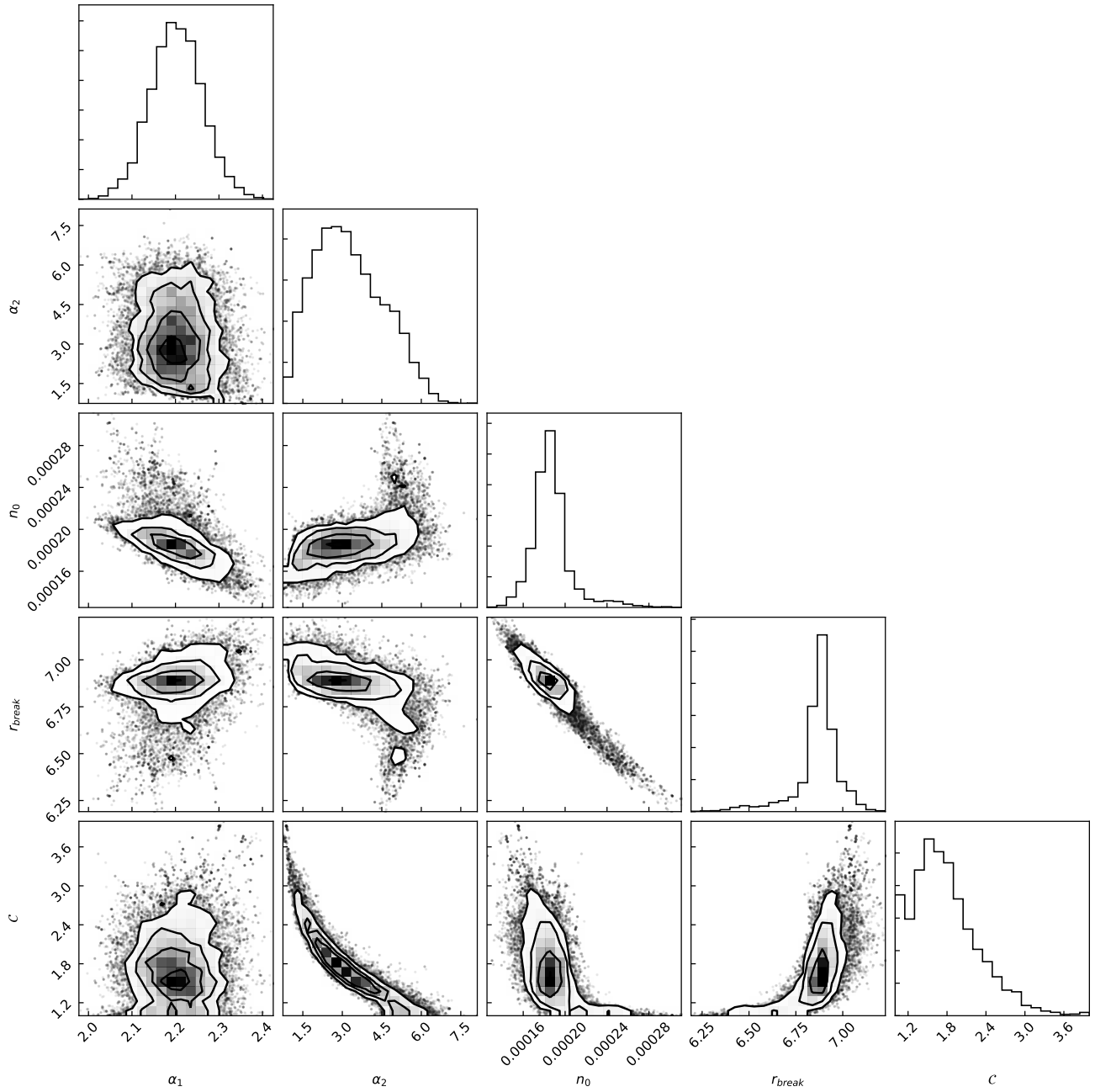
Figure A.1. The MCMC “corner plot” for the X-ray surface brightness profile across the western edge (see top left panel in Fig. 5)
