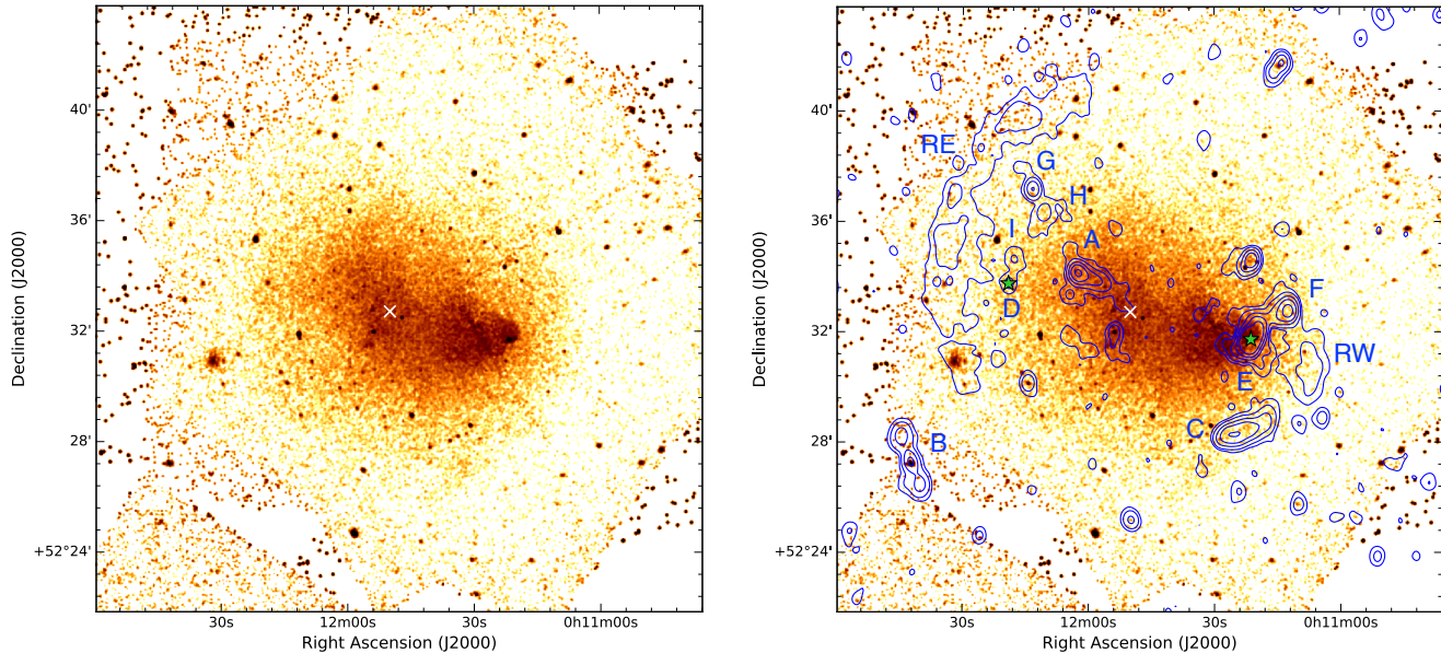
Figure 1. Left panel: background-subtracted, vignetting- and exposure-corrected 0.5–2.0 keV Chandra image of ZwCl0008 smoothed with a 2D Gaussian with \sigma = 2'' (i.e. 1 image pixel). Right panel: the same as the left panel with the 1.4 GHz WSRT radio contours at 4\sigma_{\text{rms}} \times [1, 4, 16, \dots] overlaid; the noise level of the radio map is \sigma_{\text{rms}} = 27 \mu\text{Jy beam}^{-1} (van Weeren et al. 2011b). Radio sources in the right panel have been labeled following van Weeren et al. (2011b), and the two bright central galaxies (BCGs) are identified by the two green stars. The cluster center is identified in the two panels by the white cross.
