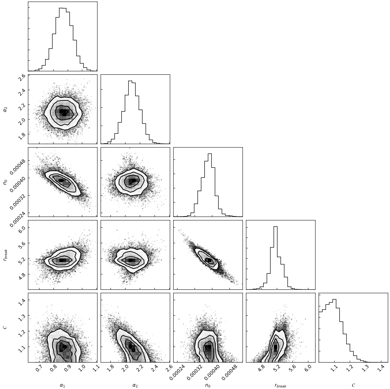
Figure A.2. The MCMC “corner plot” for the X-ray surface brightness profile across the eastern edge (see Fig. 6).
