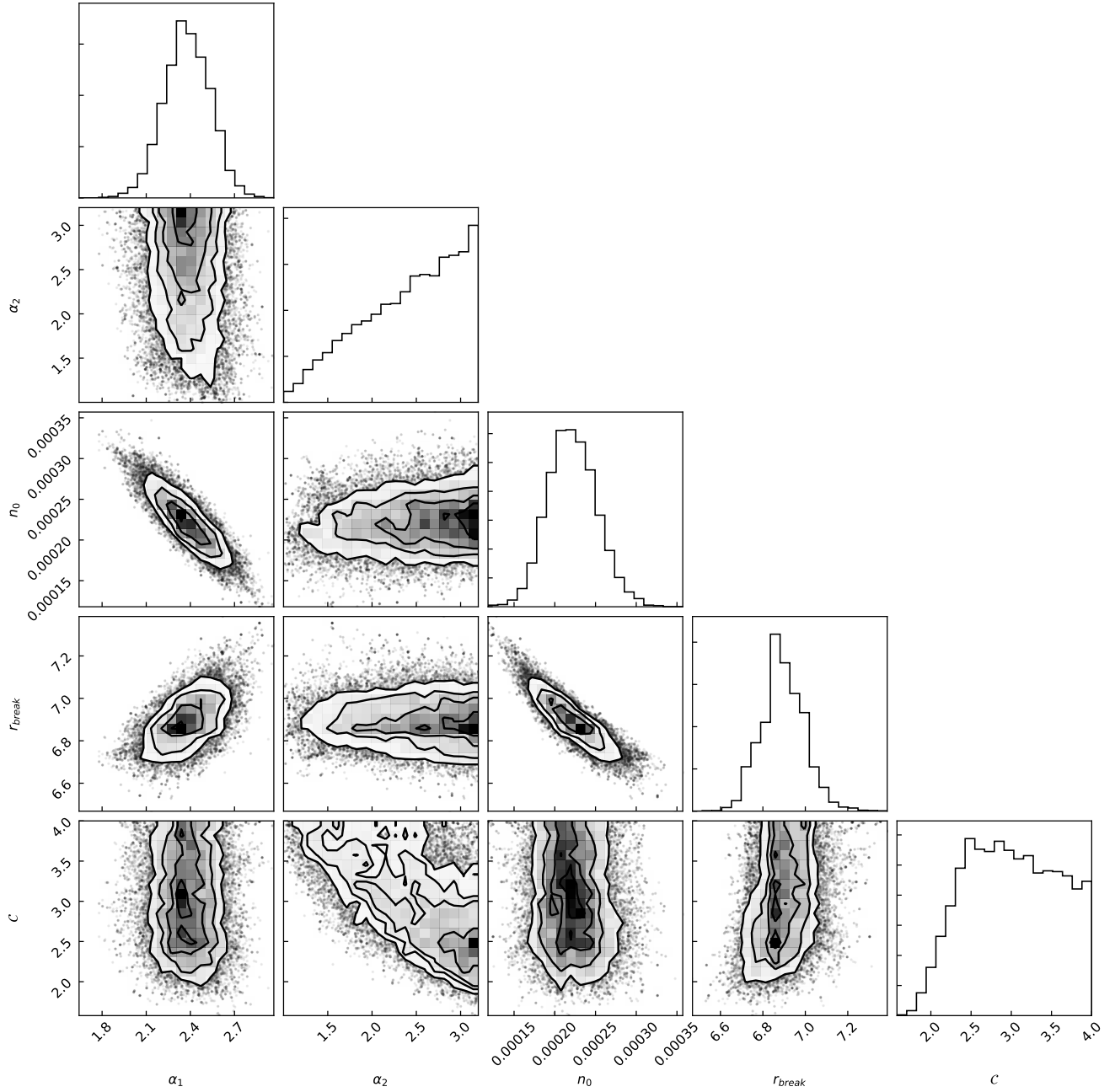
Figure A.5. The MCMC “corner plot” for the X-ray surface brightness profile across the wedge on the western relic (see top right panel in Fig. 5)
