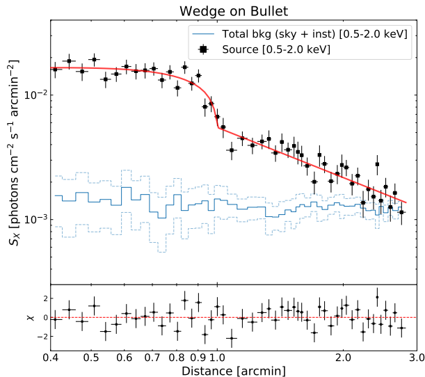
Figure 7. Surface brightness profile across the bullet sector. The total background level (i.e. instrumental and astrophysical) is shown by the light blue line, with the \pm 1\sigma uncertainties (light blue dashed lines). On the bottom, the residuals (i.e. \frac{S_{X,obs} - S_{X,mod}}{\Delta S_{X,obs}} ) are displayed.
