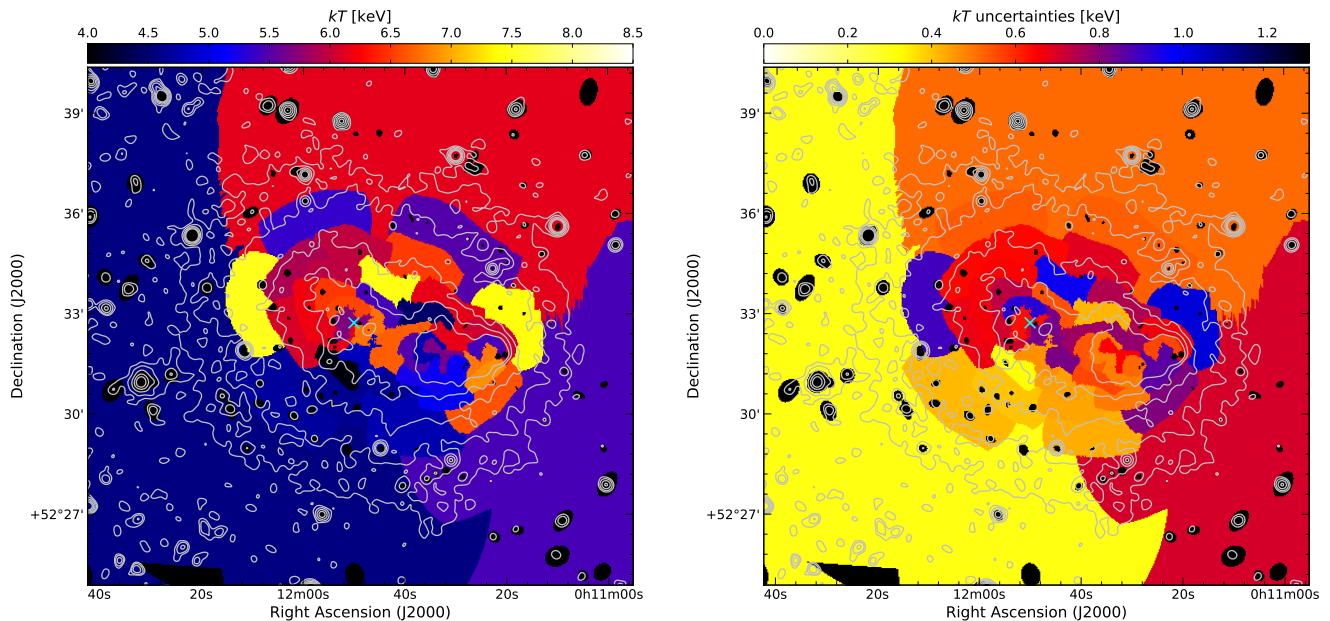
Figure 2. Temperature map (left) and the relative uncertainties (right) of ZwCl0008. Each region has a S/N = 40. Black ellipses represent the compact sources excluded from our spectral and spatial analysis. The cyan cross displays the cluster center (as Fig. 1). X-ray contours (gray) are drawn at [1.2, 2.4, 4.8, 8.2, 12] \times 10^{-6} photons \text{cm}^{-2} \text{s}^{-1} .
