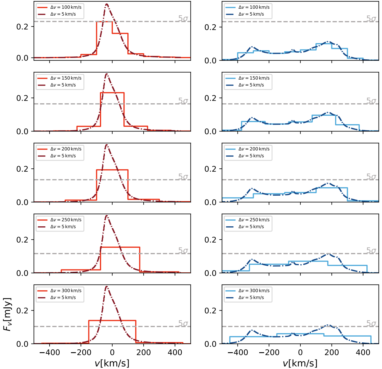
Figure 11. Comparison of the [C II] observability for face-on orientations (left panels) vs edge-on (right panels) ones when Althæa has \log(L_{\text{CII}}/L_{\odot}) = 7.7 , at z = 6.28 (Spiral Disk). From top to bottom the spectrum is re-binned with an increasing channel width ( \Delta v ). As a reference, the \Delta v = 5 \text{ km s}^{-1} case is reported in all panels. The dashed horizontal line corresponds to 5\sigma noise level, that is calculated by assuming a 10 hours ALMA observation.
