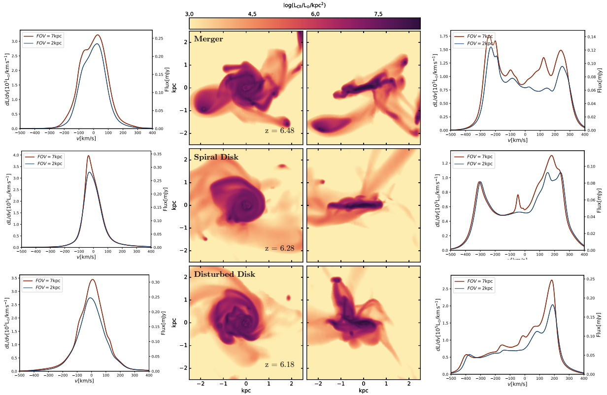
Figure 6. Left panel: [C II] spectra for the face-on inclinations taken from FOV = 7 kpc (red solid lines) and FOV = 2 kpc (blue solid lines). Middle panels: Face-on and edge-on emission maps for Althæa in different representative stages of evolution: Merger stage (top), Spiral Disk (centre), and Disturbed Disk (bottom). Right panel: [C II] spectra for the edge-on inclinations taken from FOV = 7 kpc (red solid lines) and FOV = 2 kpc (blue solid lines).
