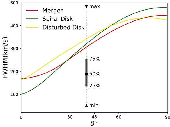
Figure 8. The FWHM of Althæa spectra as a function of inclination. Each line corresponds to a different evolutionary stage (see Fig. 6). As a reference, we over-plot the statistical properties of the FWHM from observed in high-redshift galaxies (see Table 1).
