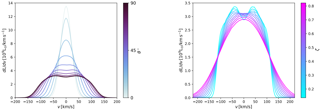
Figure 2. Spectral profile of a geometrically thin disk with an exponential profile. Left panel: Disk inclination is between \theta = 0^\circ (face-on) and \theta = 90^\circ (edge-on). In addition to rotational velocities, isotropic turbulent motions extracted from a Gaussian distribution having an r.m.s. amplitude of 20 \text{ km s}^{-1} are added to the disk. Right panel: The inclination of the disk is fixed to be edge-on and we vary the amplitude of turbulent motions. Both inclination and large turbulent motions broaden the wings of the line and lower the amplitude by a factor of \sim 4 and \sim 1.2 respectively.
