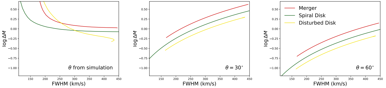
Figure 9. Analysis of the error in the dynamical mass determination using empirical estimates 16. The mass-error-function ( \Delta M , eq. 17) is plotted as a function of the FWHM for known inclination, as calculated in the simulation (left panel), and by assuming a fixed inclination of 30^\circ (central panel) and 60^\circ (right panel). Different lines indicate the three selected evolutionary stages (see Fig. 6).
