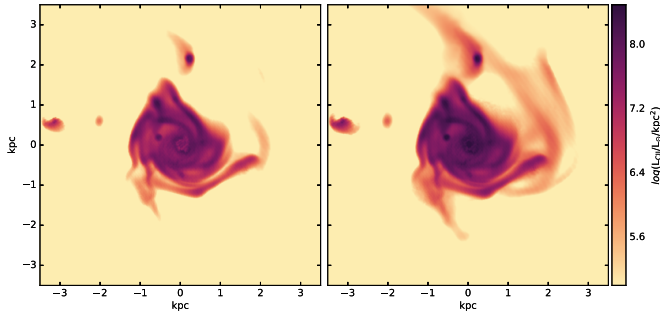
Figure A1. [C II] surface brightness of Althæa at redshift z = 6 . In the left panel ( L_{\text{tot}} = 10^{8.19}L_{\odot} ) the effect of CMB is included while in the right panel ( L_{\text{tot}} = 10^{8.52}L_{\odot} ) it is not.
