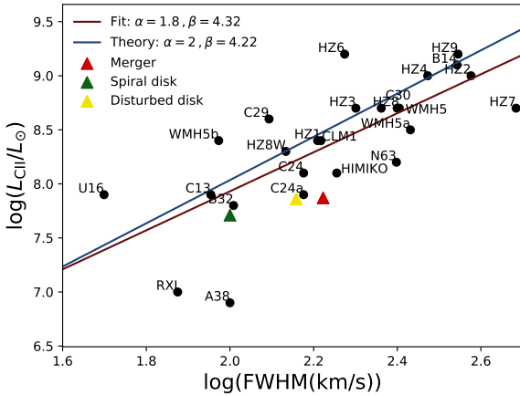
Figure 10. Correlation between L_{\text{CII}} and FWHM for the sample of observed high- z galaxies (black dots, Tab. 1). The red line indicates the fit to the data (functional form and parameters in eq.s 18). The blue line indicates the approximate relation given in eq. 21 assuming R = 1 kpc and \sin \theta = 0.5 .
