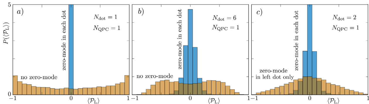
Figure 6. Same as Figure 4, but now comparing the situation with or without isolated Majorana zero-modes in a quantum dot. The quantum dots are weakly coupled ( N_{\text{QPC}} = 1 ) and they have the same number of electronic levels N_L = N_R = N_{\text{dot}} . For the blue histograms each quantum dot has a pair of isolated Majorana zero-modes (no intradot coupling, only interdot coupling). a,b) For the brown histograms, there are either no isolated zero-modes at all, or c) they are only in one of the two quantum dots. Weak coupling ensures that the peak at vanishing local fermion parity becomes a distinctive feature of isolated Majorana zero-modes in each quantum dot.
