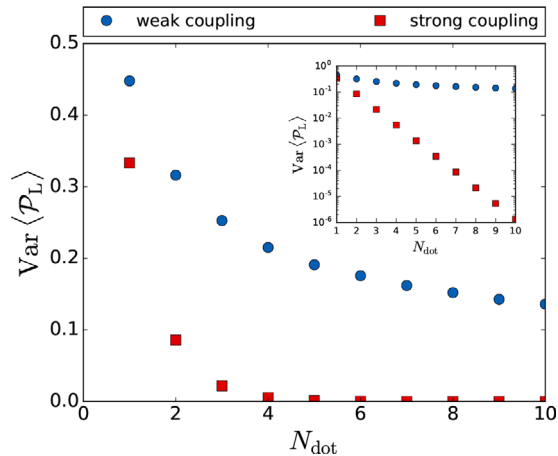
Figure 5. Comparison of the variance of P(\langle \mathcal{P} \rangle) in the skew-CRE of strongly coupled quantum dots (red data points, calculated from Equation (25)) and in the weakly coupled ensemble (blue data points, numerical results for N_{\text{QPC}} = 1 ). The inset shows that the decay is exponential in both cases, but with widely different decay rates.
