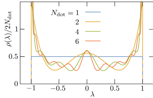
Figure 2. Density \rho(\lambda) of the eigenvalues of the 2N_L \times 2N_L matrix [-i\tilde{\mathcal{A}}]_{LL} in the skew-CRE, calculated by integration of the distribution (20) for N_L = N_R = N_{\text{dot}} \in \{1, 2, 4, 6\} . The density has a peak at the band edges and at the band center.
