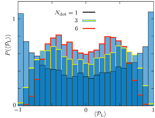
Figure 4. Probability distribution of the local fermion parity for the RMT model (27) of two weakly coupled quantum dots, calculated numerically by sampling the Gaussian matrix elements in \Omega_L, \Omega_R, \Gamma for N_{\text{QPC}} = 1, N_L = N_R = N_{\text{dot}} \in \{1, 3, 6\} . In contrast to the strongly coupled skew-CRE ensemble of Figure 3, the distribution narrows only slowly with increasing N_{\text{dot}} .
