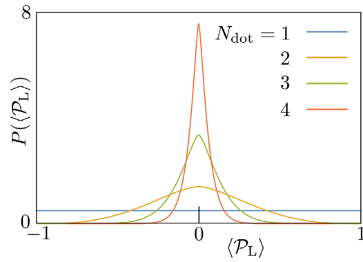
Figure 3. Probability distribution of the local fermion parity in the ensemble of antisymmetric orthogonal matrices (skew-CRE), representative of strongly coupled quantum dots. The curves are calculated from Equation (20) for N_L = N_R = N_{\text{dot}} \in \{1, 2, 3, 4\} . It takes just a few levels in the quantum dot to have \langle \mathcal{P}_L \rangle \approx 0 with high probability, so equal weight of even and odd fermion parity.
