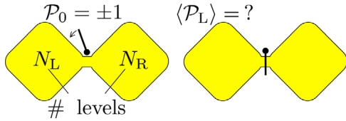
Figure 1. The left panel shows two superconducting regions (quantum dots) connected (fused) by a point contact. The entire system is in a state of definite fermion parity \mathcal{P}_0 , even (+1) or odd (−1). The parity \mathcal{P}_L of the occupation number of the N_L electronic levels in one single quantum dot has quantum fluctuations. The expectation value \langle \mathcal{P}_L \rangle \in [-1, 1] may be obtained by rapidly closing the point contact and decoupling the quantum dots (right panel), followed by a measurement of the fermion parity of a single dot. The effective number of levels N_{\text{dot}} \simeq \hbar/\delta_0\tau_c in each quantum dot that contributes to the fermion parity fluctuations is determined by the single-particle level spacing \delta_0 and the time scale \tau_c on which the interdot coupling is broken. [6] We address the question when a vanishing fermion parity \langle \mathcal{P}_L \rangle \approx 0 in such a fusion experiment is a signature of isolated Majorana zero-modes.
