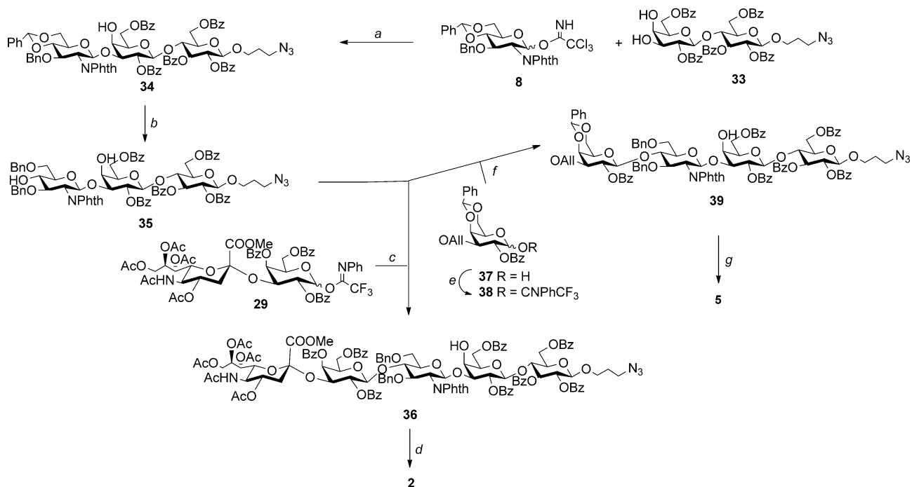
Scheme 3. Assembly of linear GBS PS Ia fragments 2 . Reagents and conditions: a) TMSOTf, CH 2 Cl 2 dry, -10 °C, (β-) 68%; b) Me 3 N-BH 3 , BF 3 -Et 2 O, MeCN, 0 °C, 65%; c) TMSOTf, CH 2 Cl 2 dry, 0 °C, (β-) 65%; d) Lil, Py, 120 °C; H 2 NCH 2 CH 2 NH 2 , EtOH, 90 °C; Ac 2 O, Py; MeONa, MeOH; H 2 , Pd-C, 33% (over five steps); e) TFA/Cl, Cs 2 CO 3 , CH 2 Cl 2 , 61%; f) TMSOTf, -20 °C, CH 2 Cl 2 , (β-) 72%; g) Pd/Cl, MeOH; H 2 NCH 2 CH 2 NH 2 , EtOH, 90 °C; Ac 2 O, Py; MeONa, MeOH; H 2 , Pd-C, 42% (over five steps).
