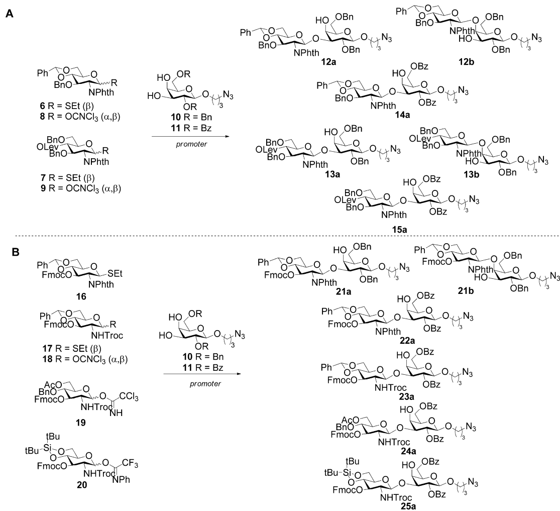
Scheme 1. A) Preparation of disaccharide intermediates 12–15 for the synthesis of GBS CPS Ia repeating unit. Promoters and conditions are described in Table 1. B) Preparation of disaccharide intermediates 21–25 for the synthesis of GBS PSIIb repeating unit. Promoters and conditions are described in Table 2.
