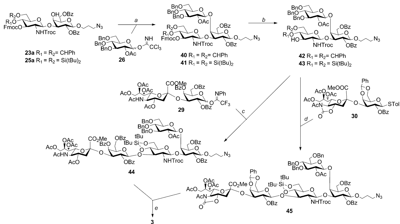
Scheme 4. Assembly of GBS PS Ib pentasaccharide branched unit 3 . Reagents and conditions: a) TMSOTf, \text{CH}_2\text{Cl}_2 dry, 0 °C, ( \beta -) 63% for 41 , ( \beta -) 70% or 42 ; b) piperidine, \text{CH}_2\text{Cl}_2 dry, 92%; c) TMSOTf, \text{CH}_2\text{Cl}_2 dry, 0 °C, ( \beta -) 80%; d) TfOH, NIS, \text{CH}_2\text{Cl}_2 dry, -40^\circ\text{C} , ( \beta -) 65%; e) HF/pyridine, 0 °C; 3 M NaOH, THF, reflux; \text{Ac}_2\text{O}/\text{MeOH} ; \text{H}_2/\text{Pd-C} , 40%.
