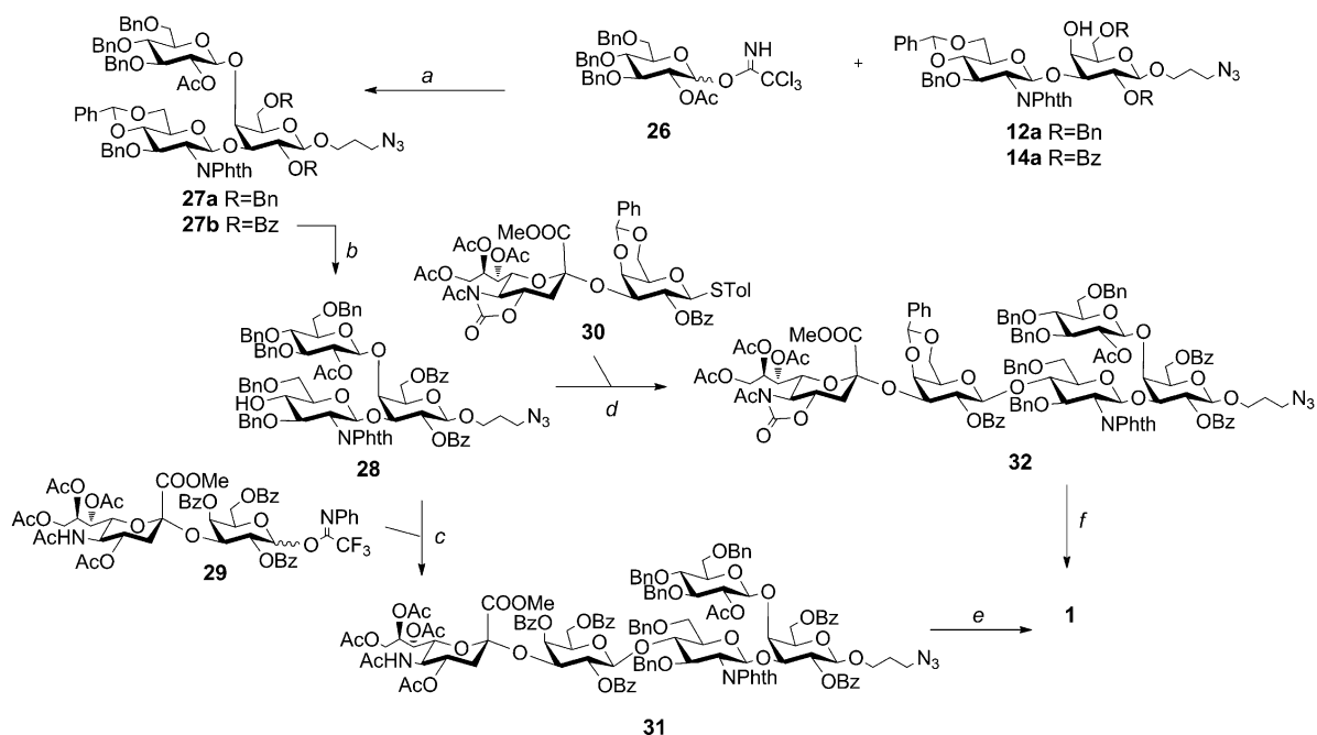
Scheme 2. Assembly of GBS CPS Ia repeating unit. Reagents and conditions: a) TMSOTf, CH 2 Cl 2 dry, -10 °C, (β-) 75% from 12a , 68% (β-) from 14a ; b) Me 3 N-BH 3 , BF 3 -Et 2 O, MeCN, 0 °C, 70%; c) TMSOTf, CH 2 Cl 2 dry, 0 °C, (β-) 75%; d) TFOH, NIS, CH 2 Cl 2 dry, -40 °C, (β-) 73%; e) Lil, Py, 120 °C; H 2 NCH 2 CH 2 NH 2 , EtOH, 90 °C; Ac 2 O, Py; MeONa, MeOH; H 2 , Pd-C, 40% (over five steps); f) 3 M NaOH, THF, reflux; Ac 2 O, MeOH; H 2 , Pd-C, 45% (over three steps).
