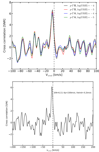
Figure 2: Cross Correlation Functions (CCFs) with the largest significance obtained for all H 2 O bands in the 1.0–1.7 μm range. Top: for HD 189733 b (after [4]). Bottom: preliminary results obtained for HD 209458 b. Note the different scales.
